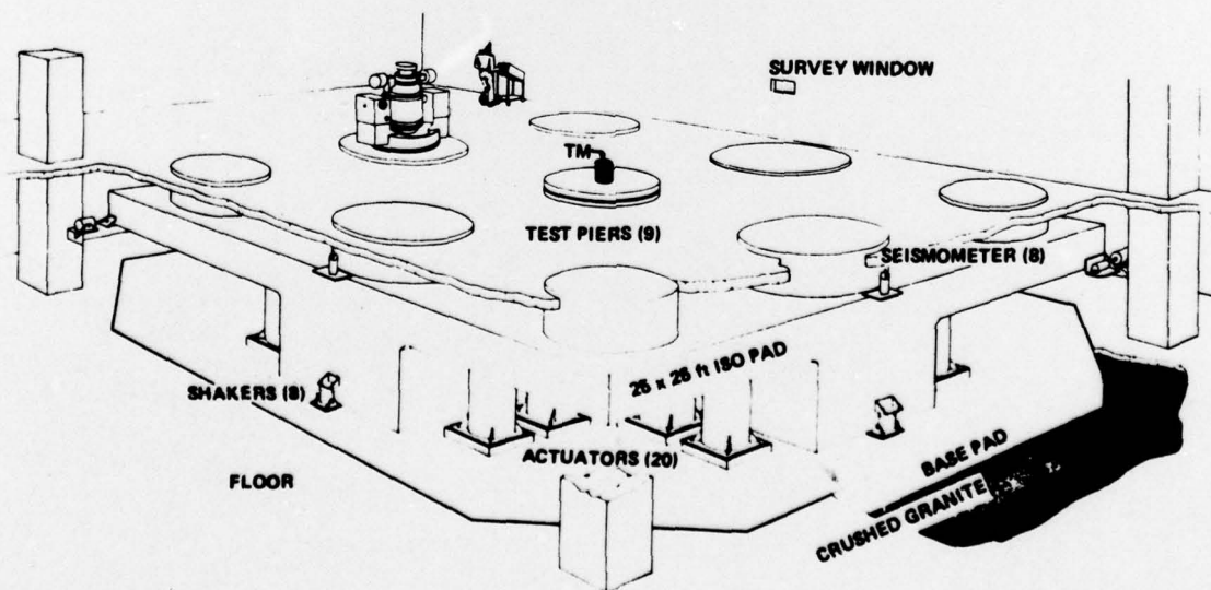
FIGURE 2. Iso-pad Pictorial
