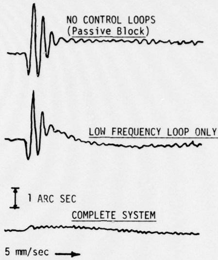
FIGURE 9. Response of the N-S Axis Angular Control System to a 60 lb-ft Step Torque Input
