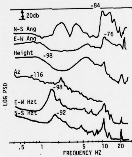
FIGURE 8. Active-servo Performance
