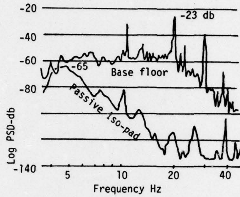
FIGURE 3. Passive Isolation
