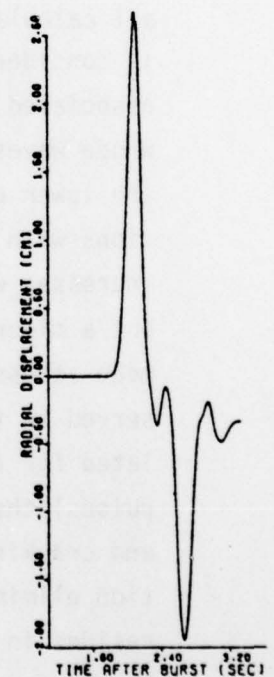
Fig. 7--Displacement pulses in the elastic near-field of a 150-kiloton burst, for three depths of burial in a half-space of wet sandstone. The pulses refer to points of a down-going ray 15° off the vertical, at distances from the shot point denoted by values of "RANGE."
