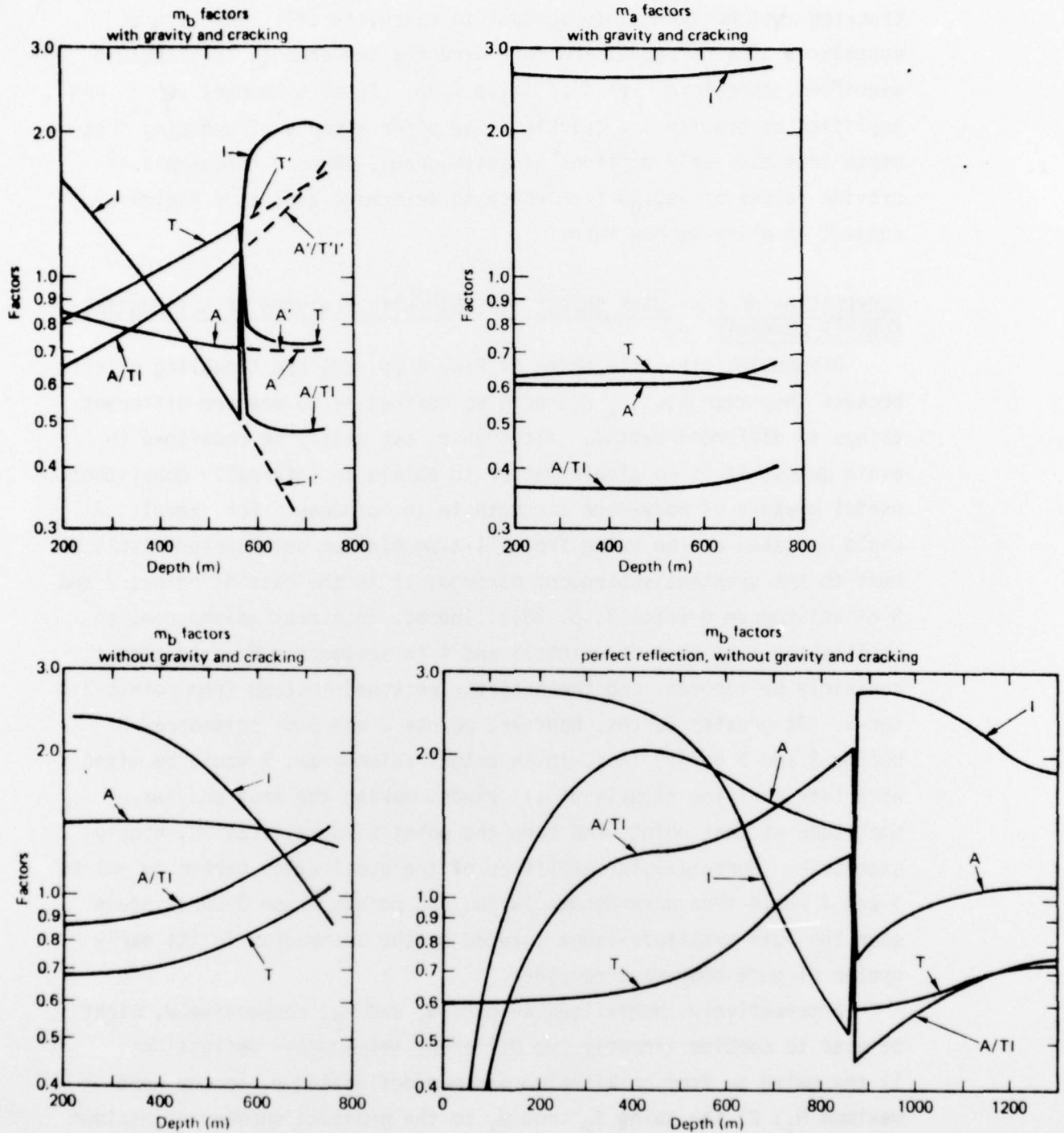
Fig. 11--Three depth-dependent factors that determine body-wave magnitudes m_a and m_b , versus shot depth, for 150-kiloton bursts in a wet-sandstone half-space. Amplitude A is equal to the seismometer deflection from its all-time minimum, either to its next-earlier maximum ( m_a ), or to its next-later maximum ( m_b ). T is twice the time-interval between the extremes that define A ; the instrument correction I varies with T only. Changes in magnitude with depth are identical to changes in \log_{10}(A/TI) --also shown.
