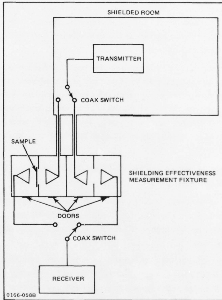
Figure A-6 Shielding Effectiveness Measurement Set-Up
