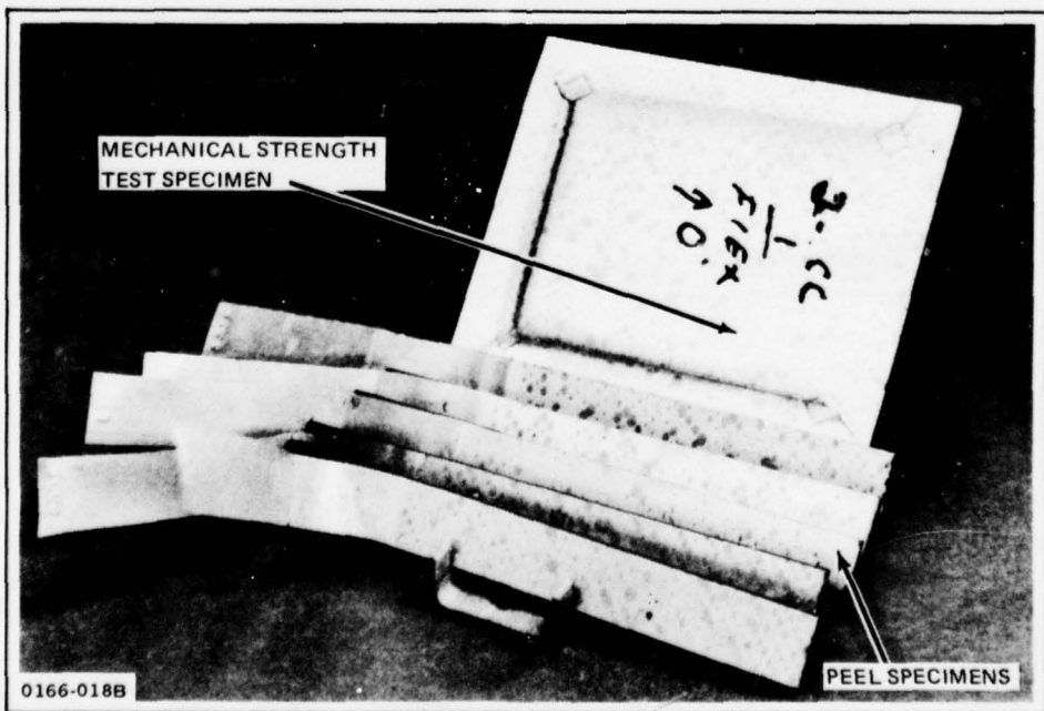
Figure 4-16 Cocured Foil-Coated Graphite/Epoxy Humidity Exposure Test Specimens
