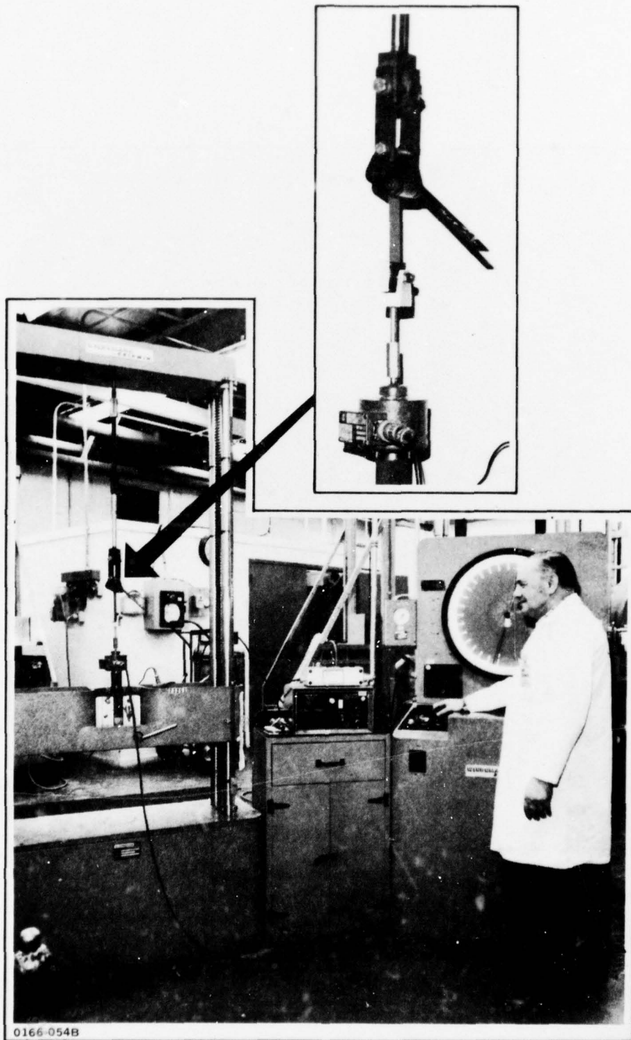
Figure A-2 Bell Method Peel Test Setup
