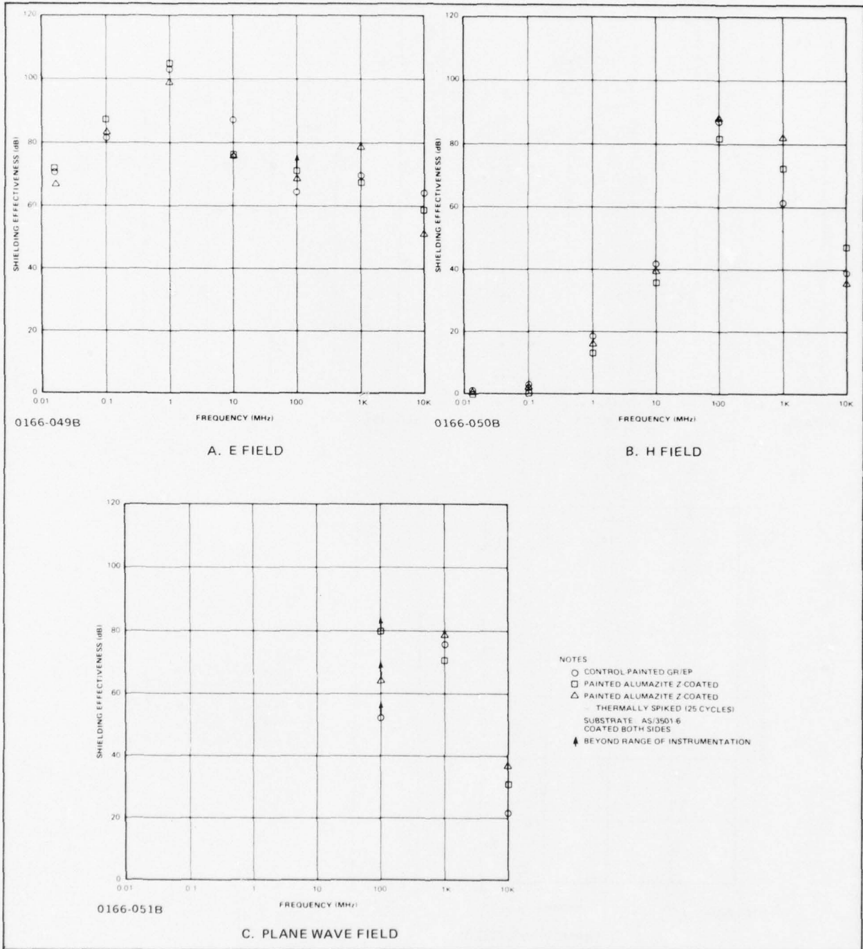
Figure 5-15 Effect of Thermal Spiking on EMI Shielding Effectiveness of Alumazite Z-Coated Graphite/Epoxy
