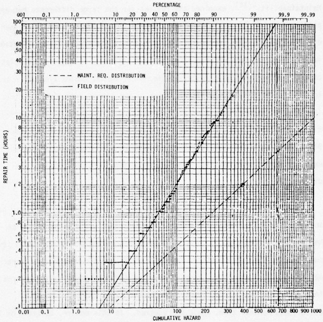
FIGURE 25. FIELD-TIME-TO-REPAIR LOGNORMAL DISTRIBUTION
