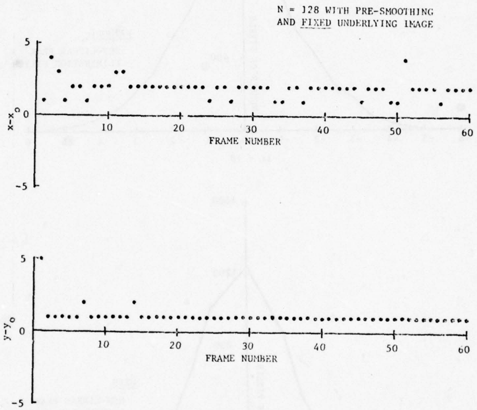
Figure 39. Accumulated Tracking Error
