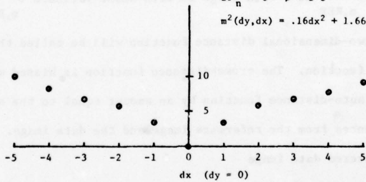
Figure 7. Auto-Distance Function for a Simulated Noisy Image
