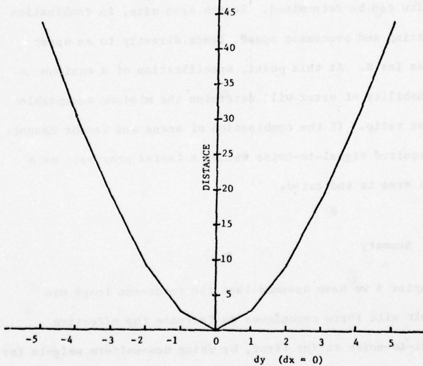
Figure 35. Auto-Distance Function for a 32 by 32 Block of Contiguous Pixels
