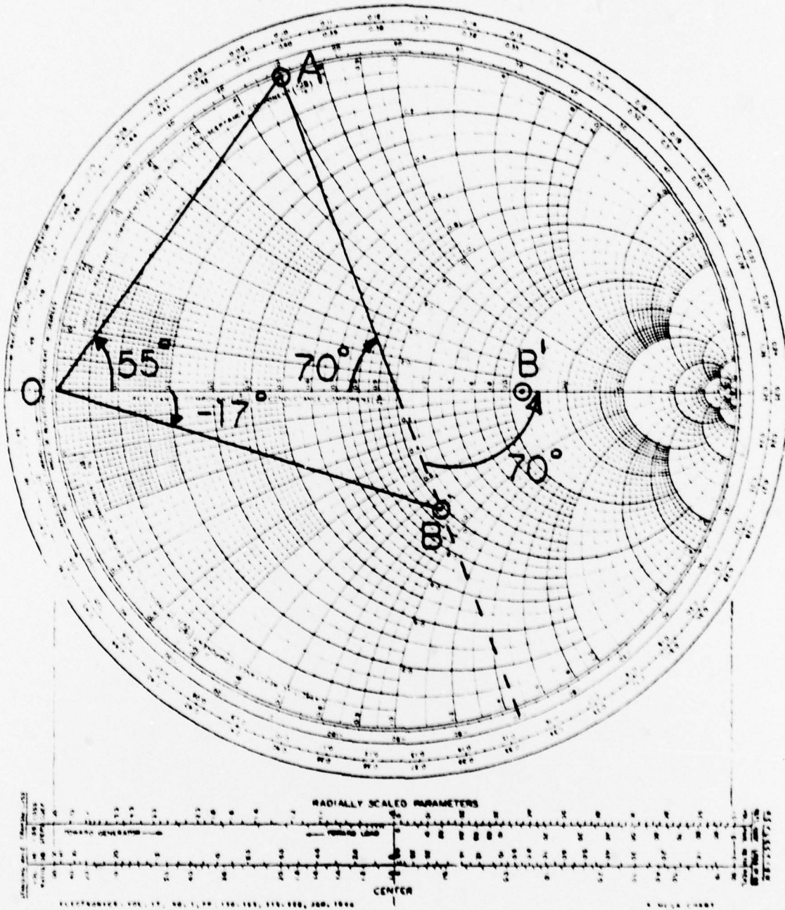
Figure A-3 Example of Impedance Measurement Procedure
