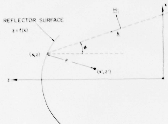
Figure 2. Reflector Treated as a Receiving Antenna
