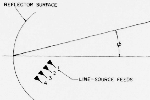
Figure 1. Example of Limited - Scan Reflector
