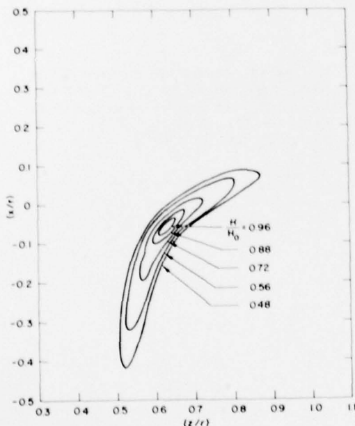
Figure 15. Contour Plot of the Received Magnetic Field Amplitude When the Reflector Defined by Eq. (2) is Illuminated by a Plane Wave Incident at \phi = 0^\circ . Also, \theta_0 = -80.5^\circ , \theta_1 = 0^\circ and r_0 = 15\lambda
