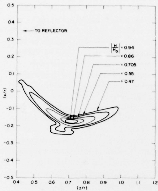
Figure 13. Contour Plot of the Received Magnetic Field Amplitude When the Reflector Defined by Eq. (2) is Illuminated by a Plane Wave Incident at \phi = 12^\circ . Also, \theta_0 = -45^\circ , \theta_1 = 45^\circ , and r_0 = 15\lambda
