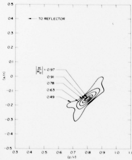
Figure 17. Contour Plot of the Received Magnetic Field Amplitude When the Reflector Defined by Eq. (2) is Illuminated by a Plane Wave Incident \phi = 12^\circ . Also, \theta_0 = -80.5^\circ , \theta_1 = 0^\circ and r_0 = 15\lambda
