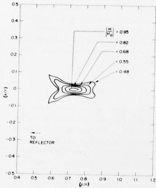
Figure 11. Contour Plot of the Received Magnetic Field Amplitude When the Reflector Defined by Eq. (2) is Illuminated by a Plane Wave at \phi = 0^\circ . Also, \theta_0 = -45^\circ , \theta_1 = 45^\circ , and r_0 = 15\lambda
