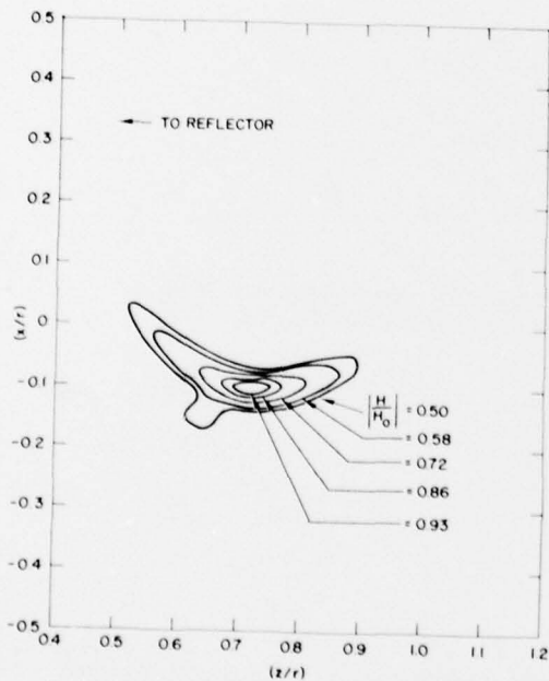
Figure 12. Contour Plot of the Received Magnetic Field Amplitude When the Reflector Defined by Eq. (2) is Illuminated by a Plane Wave at \phi = 7^\circ . Also, \theta_0 = -45^\circ , \theta_1 = 45^\circ , and r_0 = 15\lambda
