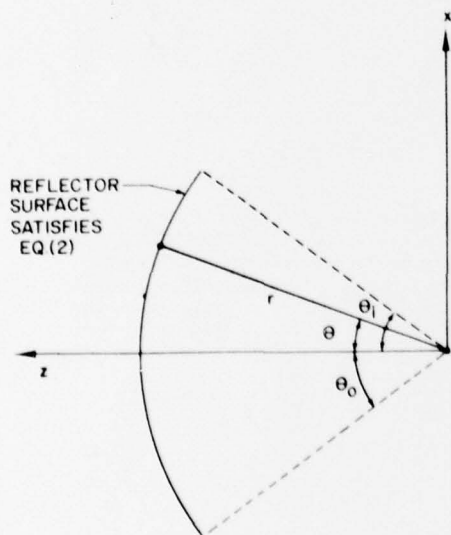
Figure 10. Geometry for Study of the Surface Defined by Eq. (2)
