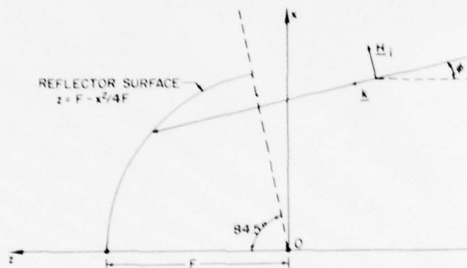
Figure 3. Offset Parabolic Cylinder. The ratio of the focal length, F , to diameter, D , is F/D = 1/2
