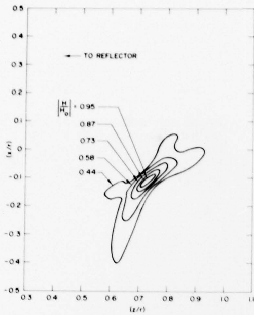
Figure 16. Contour Plot of the Received Magnetic Field Amplitude When the Reflector Defined by Eq. (2) is Illuminated by a Plane Wave Incident at \phi = 7^\circ . Also, \theta_0 = -80.5^\circ , \theta_1 = 0^\circ and r_0 = 15\lambda
