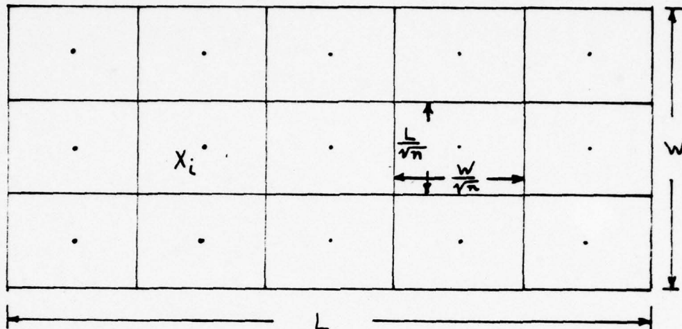
Figure 6. Fixed lattice of points
