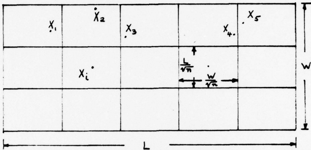
Figure 13. n carriers randomly patrolling a 2 dimensional area.
