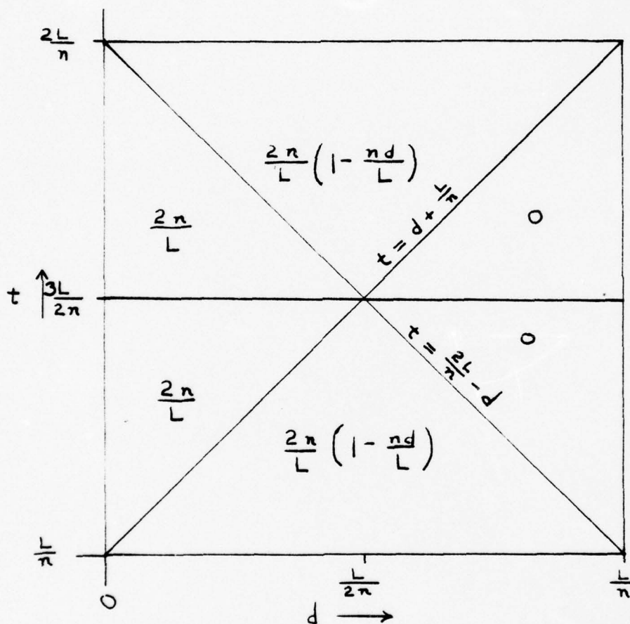
Figure 4. Unconditional probability density function
