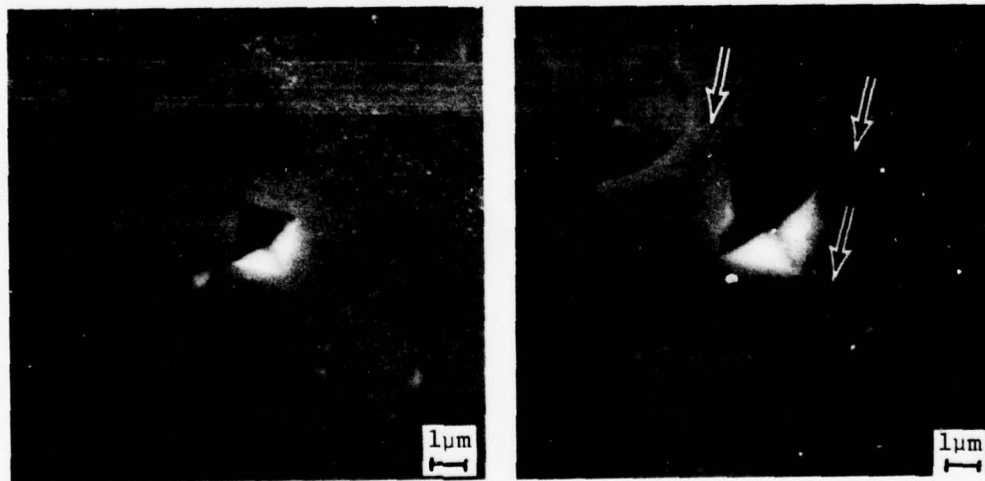
(b) 50 gm load, radial cracking (arrow), twins formed
