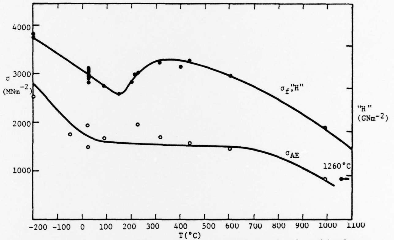
Fig. 1. Compressive strength, acoustic emission stress level, and hardness, versus temperature for Al 2 O 3 .
