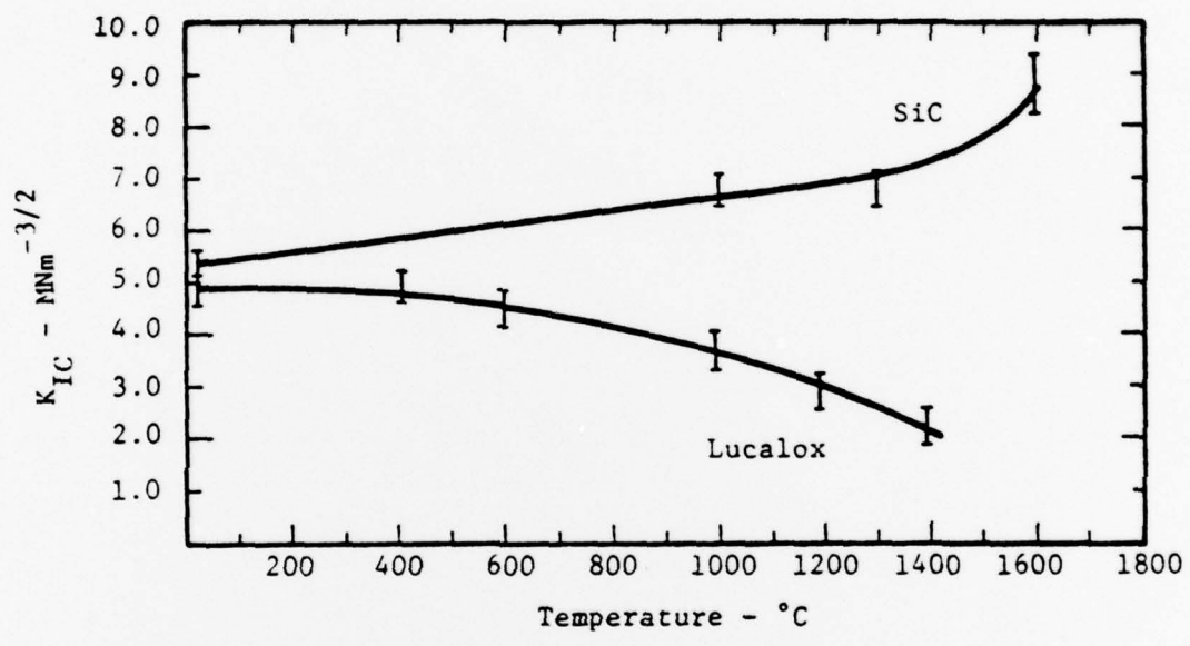
Fig. 6 . Fracture toughness versus temperature for \alpha\text{-SiC} (Kraft and Doohar, 1976) and Lucalox \text{Al}_2\text{O}_3 (Evans, Linzer, and Russell, 1974).
