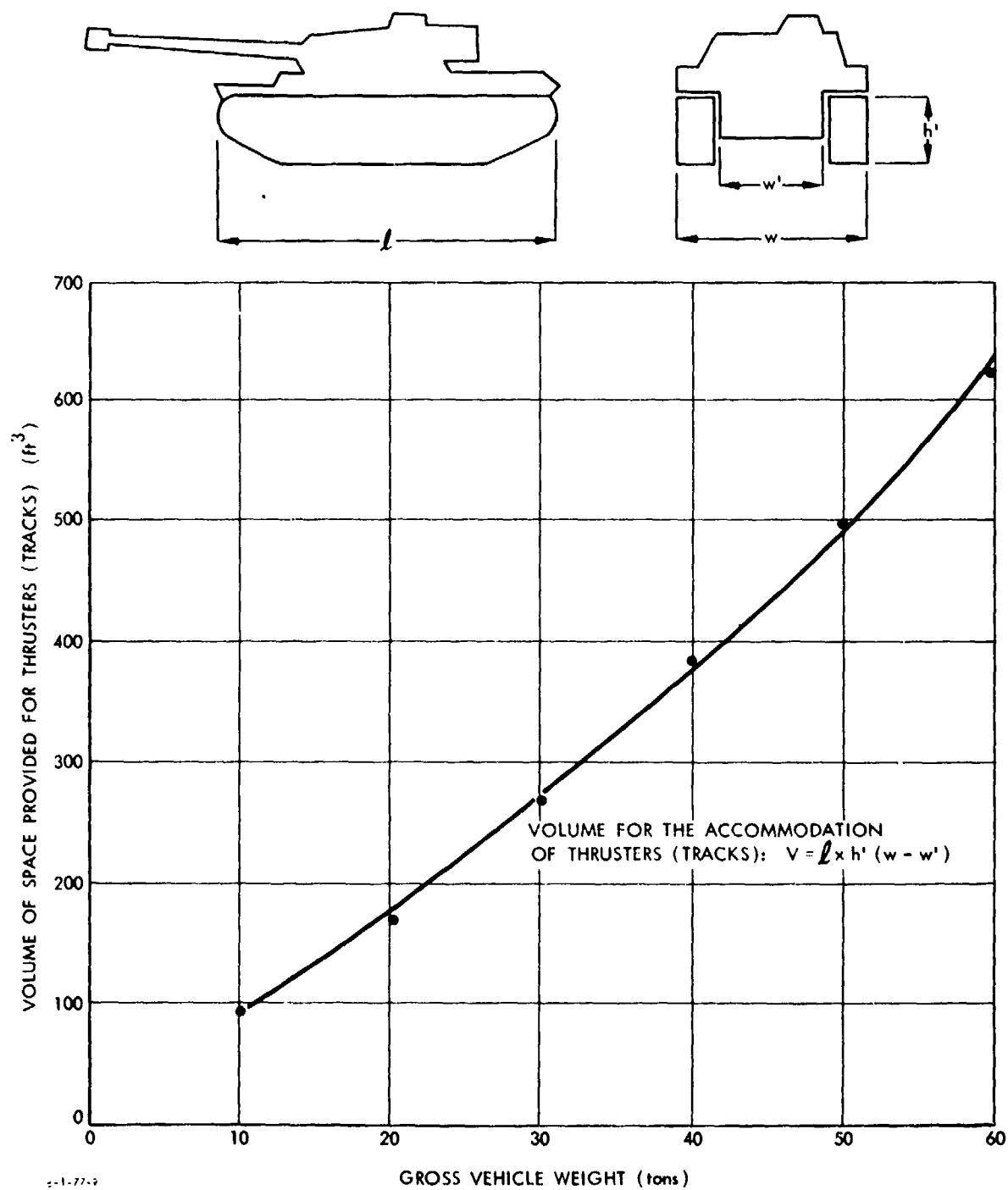
FIGURE K-9. Volume of space provided for thrusters versus gross vehicle weight.
