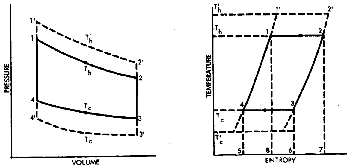
FIGURE G-5. Pressure-volume and temperature-entropy diagrams of ideal Stirling cycle, illustrating effect of variation in cycle temperature limits.
