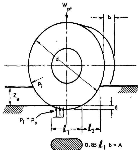
FIGURE K-29. Explanatory diagram for notation of Eq. K-16.
