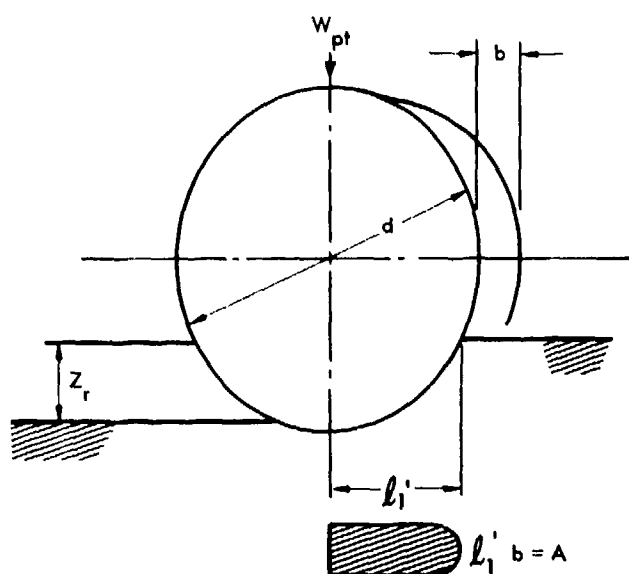
FIGURE K-30. Explanatory diagram for notation of Eq. K-17.
