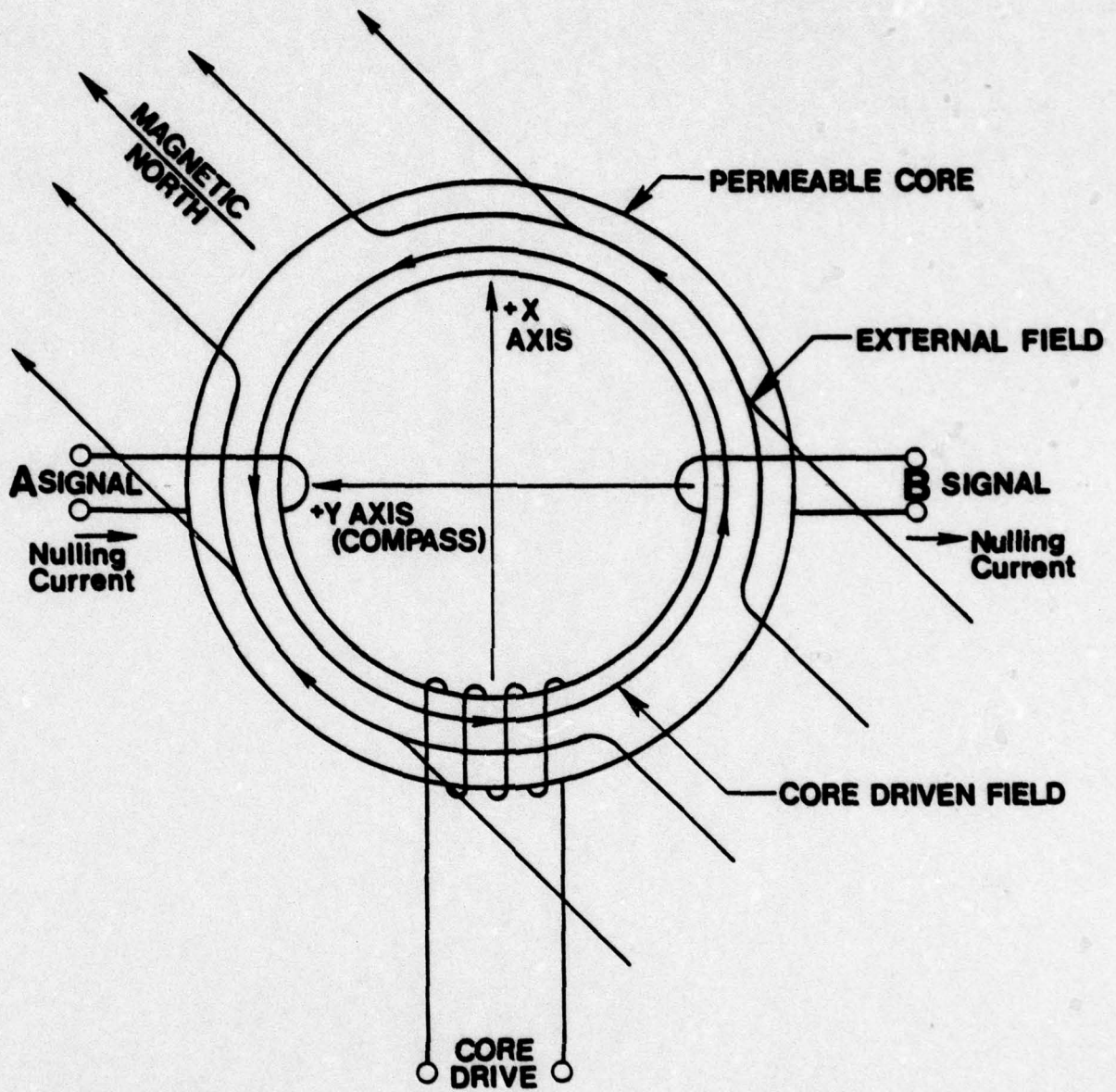
CONCEPTUALIZED COMPASS WINDINGS (1 AXIS)
