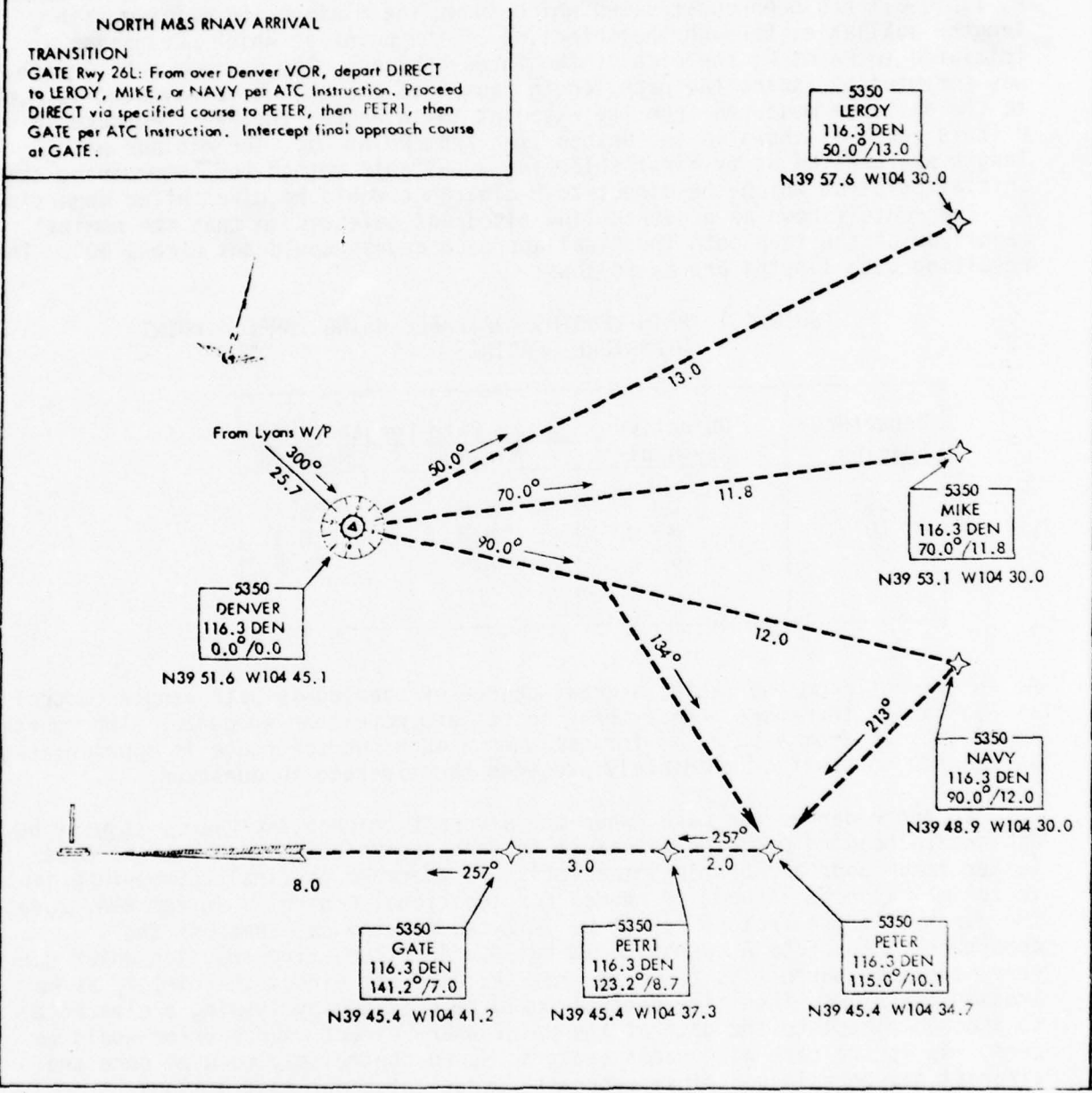
Figure C.3 Example RNAV M&S STAR Procedure
