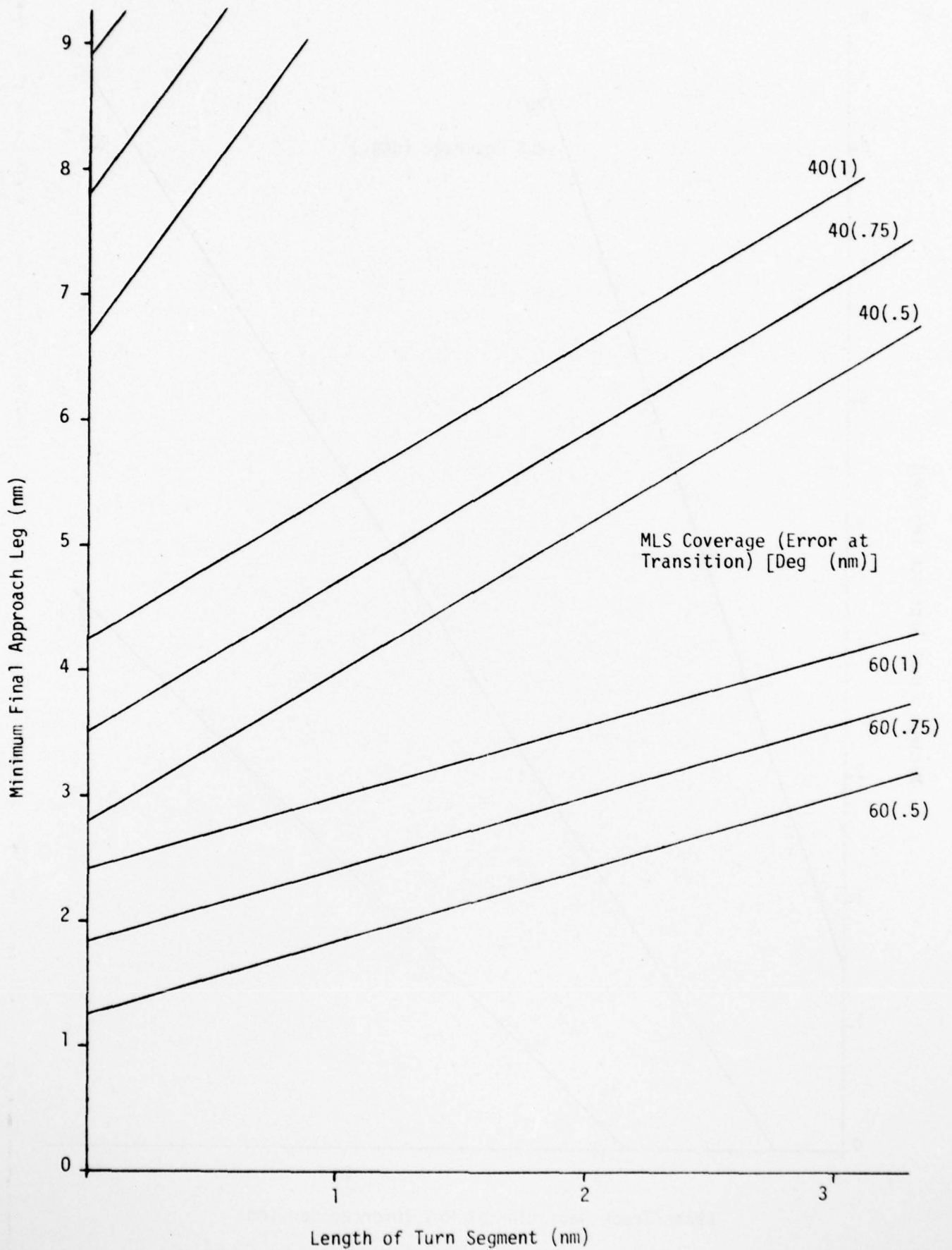
Figure D.5 Minimum Final Approach Leg for 180° Turn-to-Final
