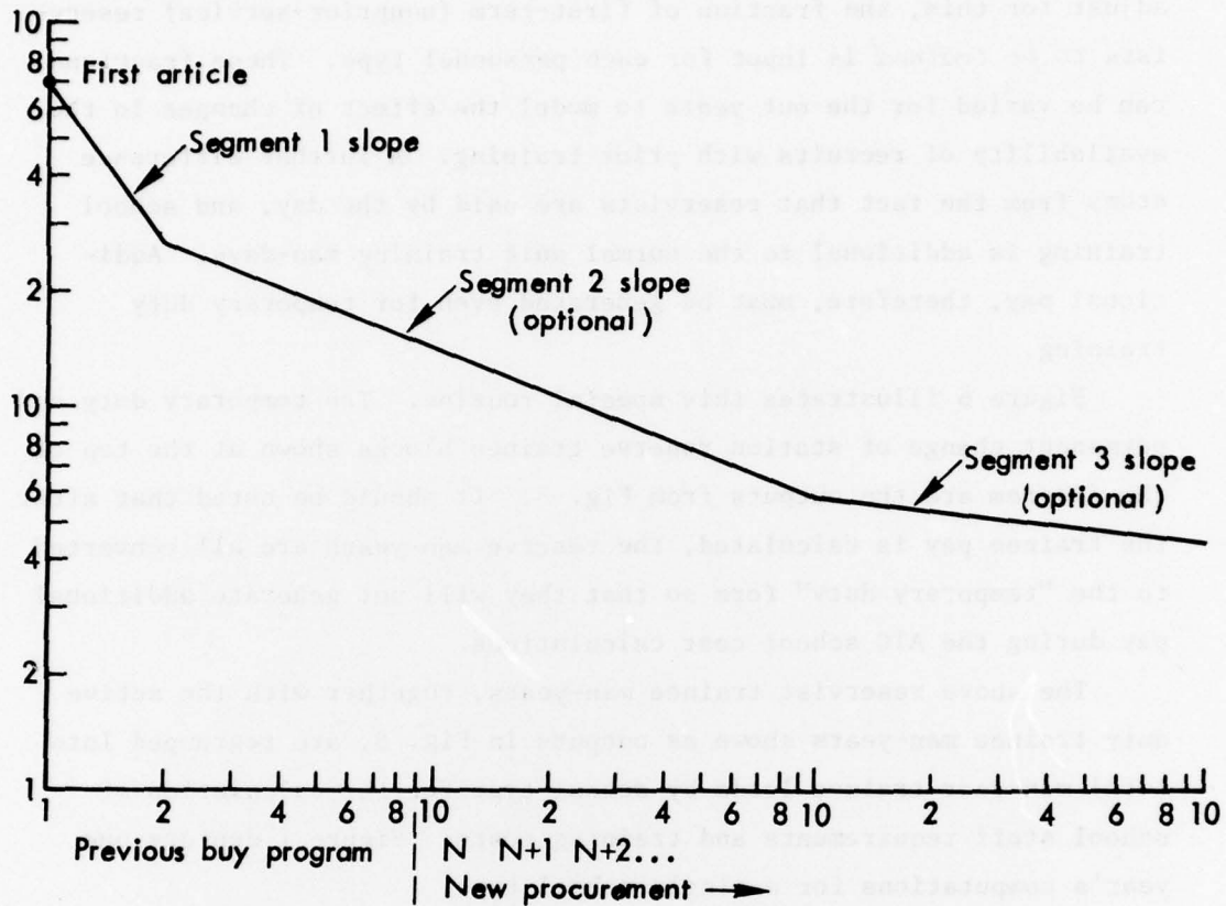
Fig. 8 — Equipment cost estimating routine
