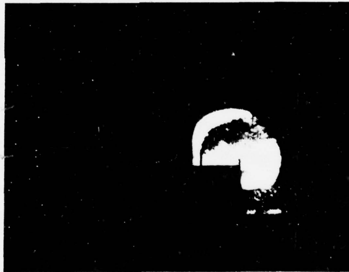
Figure 22. Spark Shadowgraphs of Injection Jet
