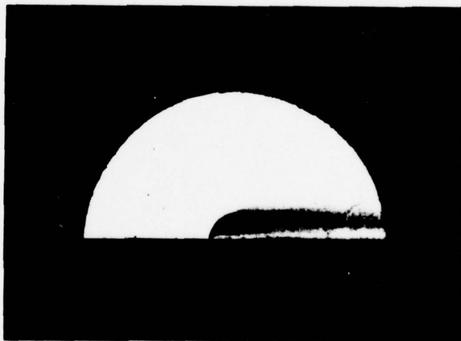
Figure 18. Streak Shadowgraphs of Injection Jet
