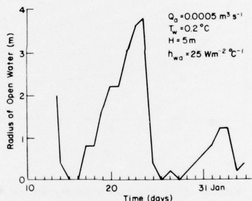
Figure 8. Variation of open water area for simulation example.
