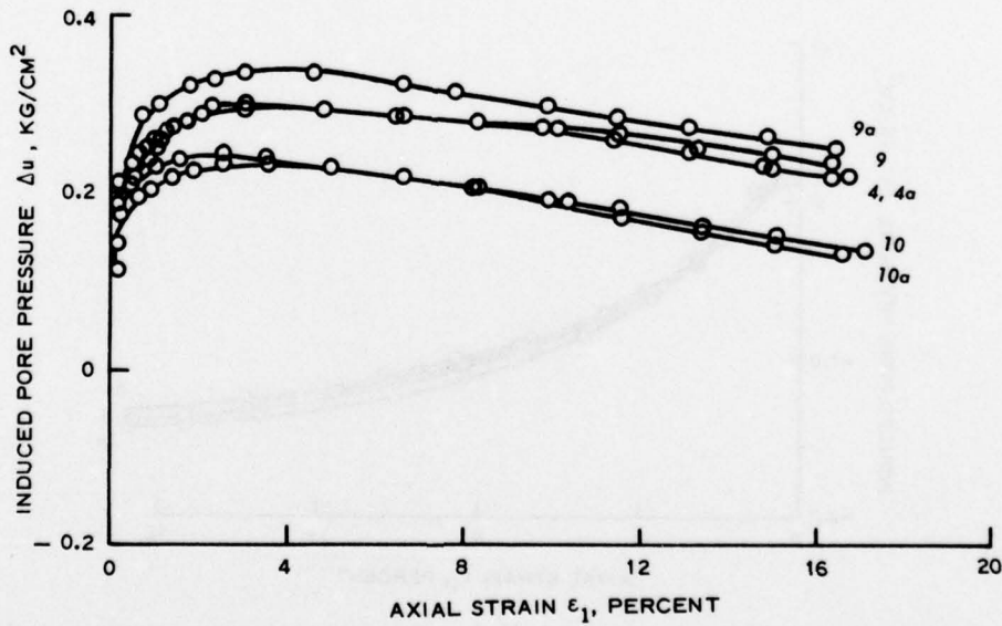
Figure 11. Deviator stress and induced pore pressure versus axial strain curves for tests in which the magnitude of the effective consolidation stress during saturation was varied, CH specimens
