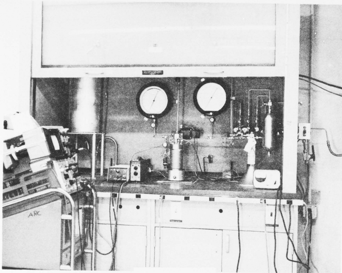
Figure 3. Gas-Handling Apparatus
