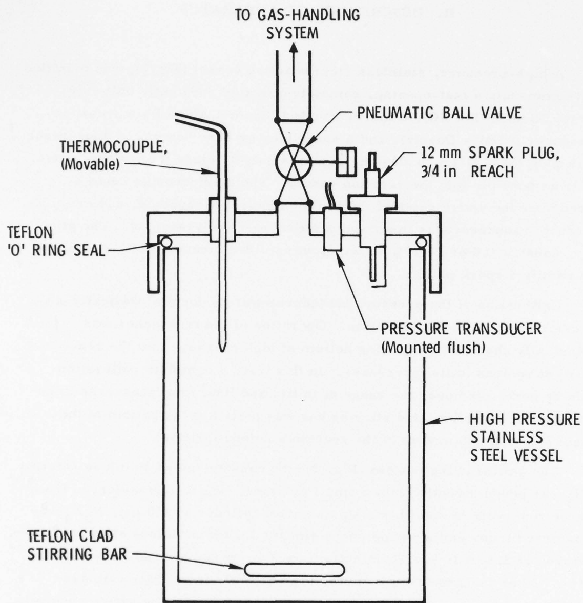
Figure 1. Reaction Vessel
