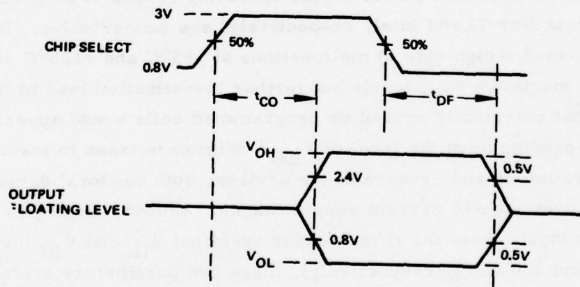
Figure 6. Switching time reference levels for t_{DF} .
