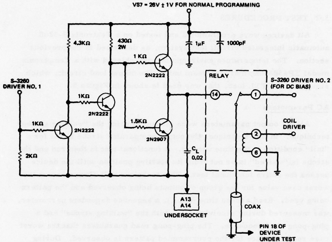
Figure 4. Driver circuit for programming UV-PROMs on the S-3260.
