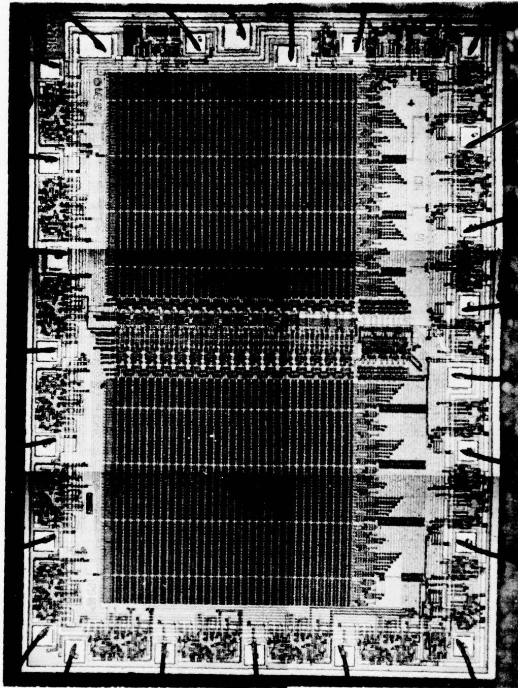
Figure 2. Intel's UV-PROM chip, MC2708. The actual chip size is 0.135 x 0.188 inch.
