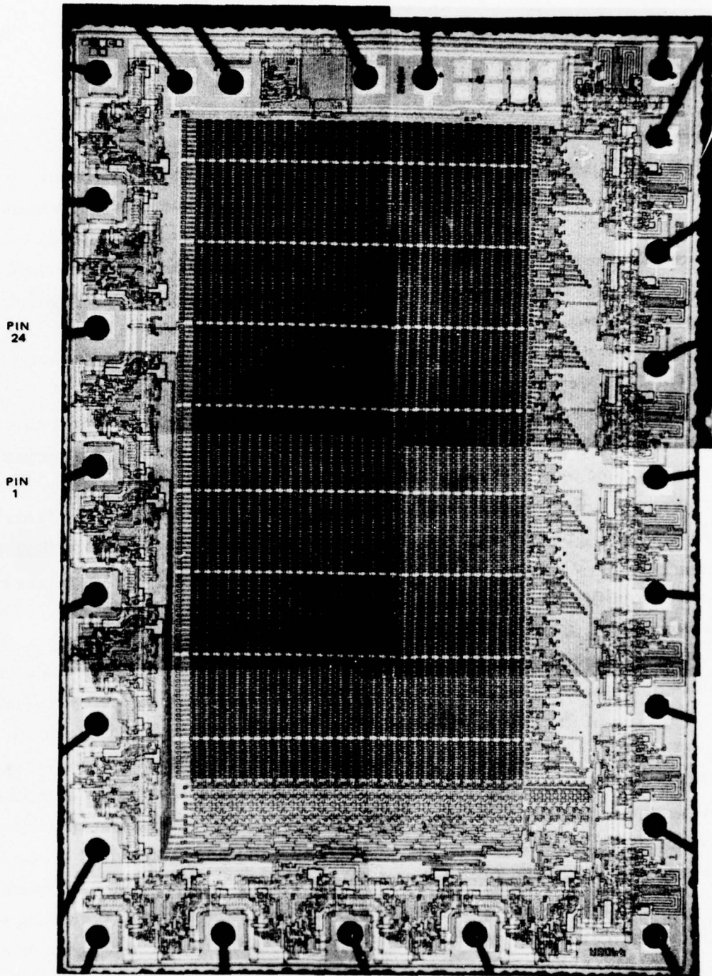
Figure 3. Texas Instrument's UV-PROM chip, SMJ2708. The actual chip size is 0.190 x 0.125 inch.
