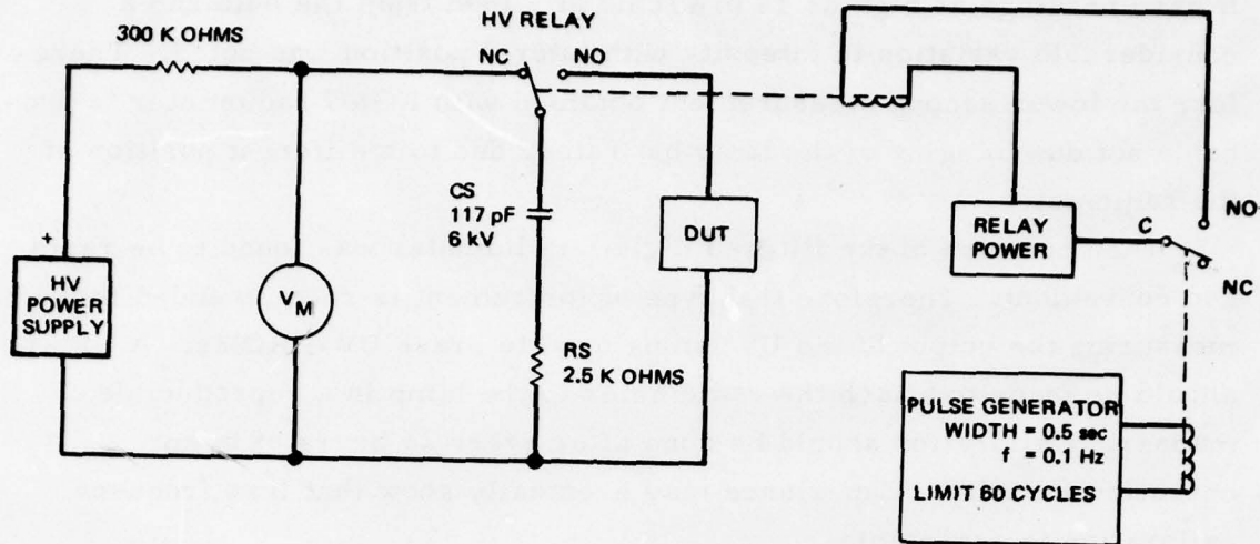
Figure 7. Electrostatic discharge stress circuit.
