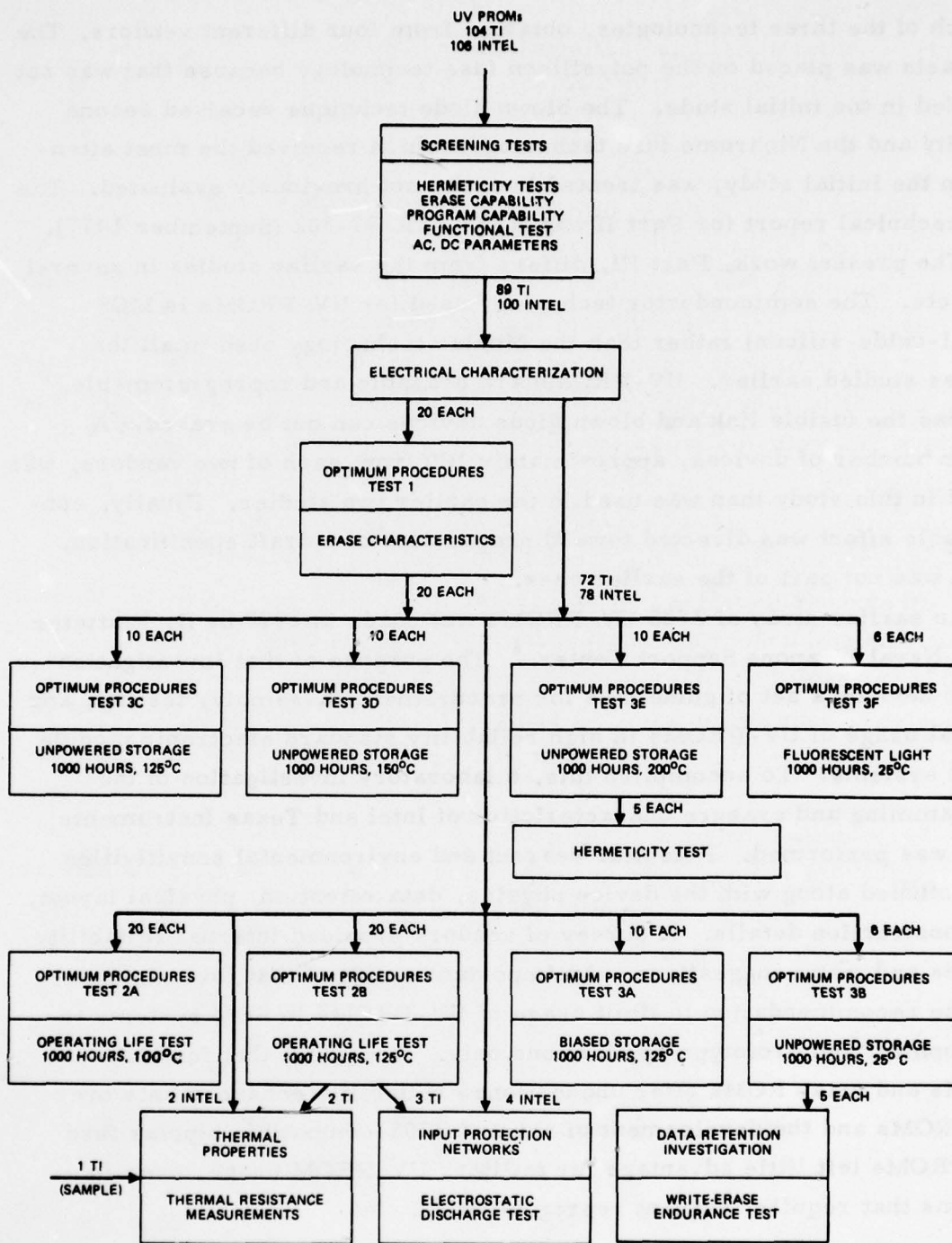
Figure 1. Reliability evaluation of ultraviolet erasable PROMs.
