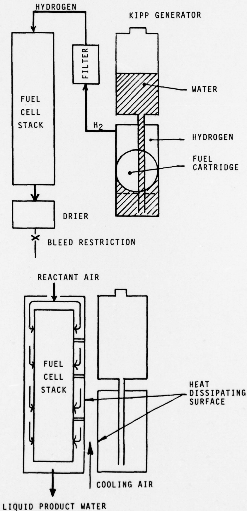
FIGURE 1 - SYSTEMS SCHEMATIC
