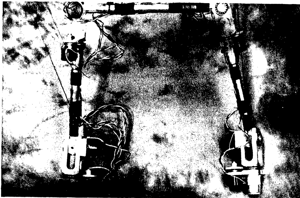
Fig. 10. Close-up view of the exoskeletal device (ESD).
