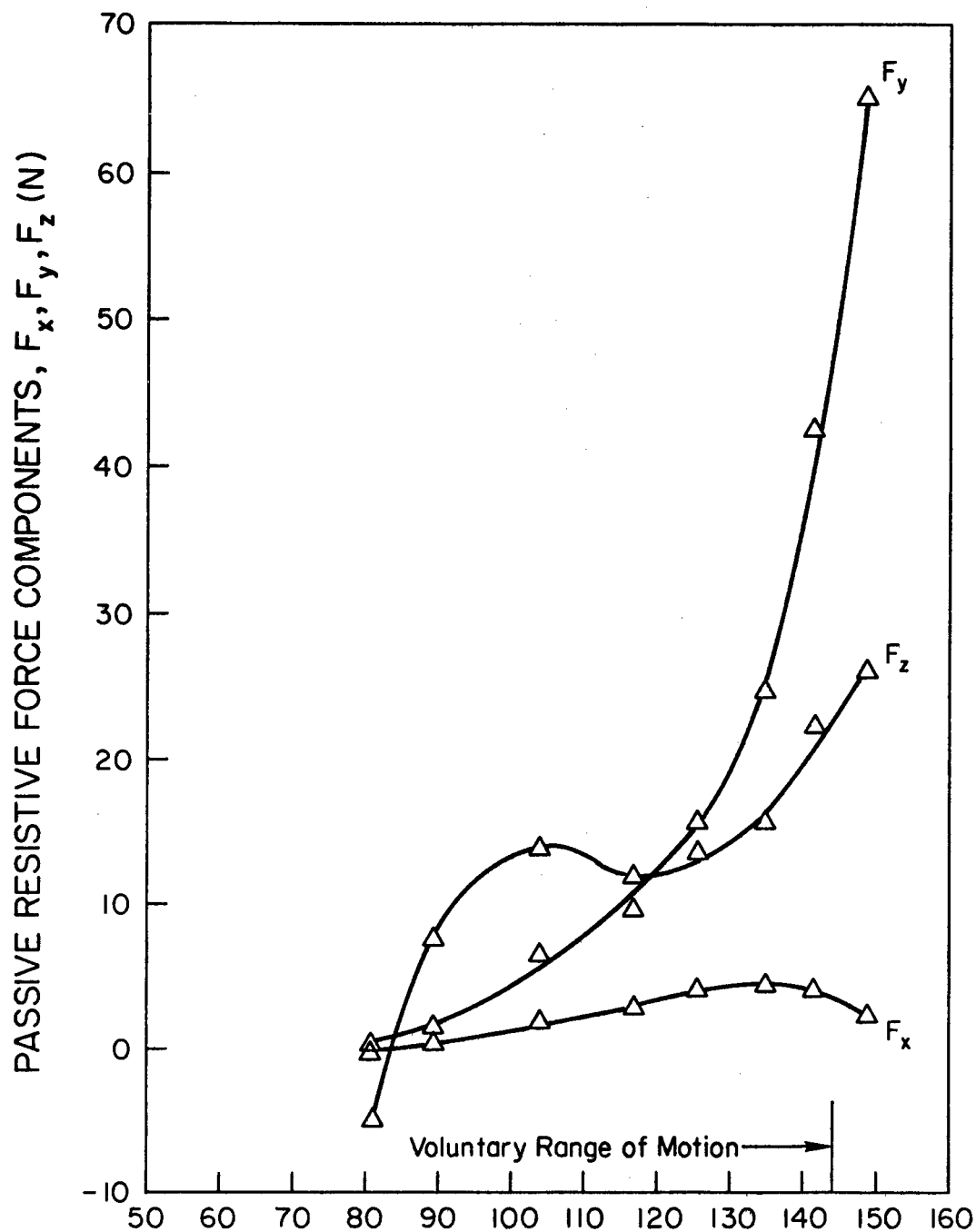
FORCED SWEEP OF THE ARM FOR SHOULDER ABDUCTION, \theta^\circ
