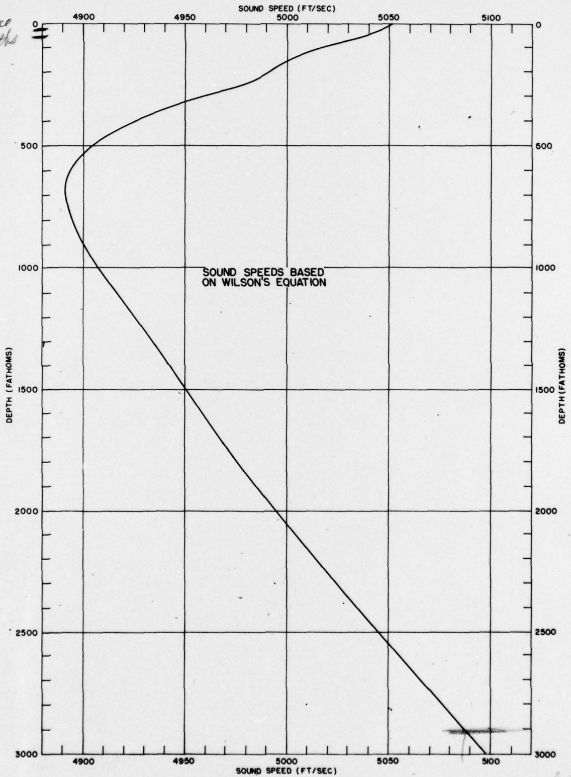
FIGURE 1 TYPICAL SOUND SPEED PROFILE FOR APRIL THROUGH JULY
