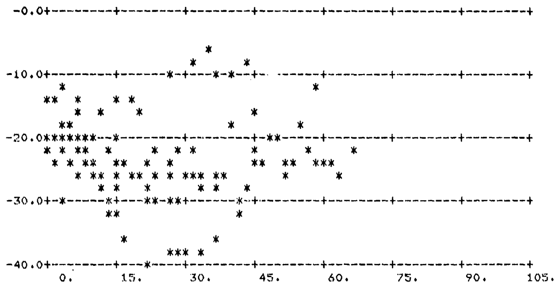
FIGURE A-5. \sigma_0 vs \phi_s ; \theta_s = 70^\circ , \theta_i = 60^\circ
