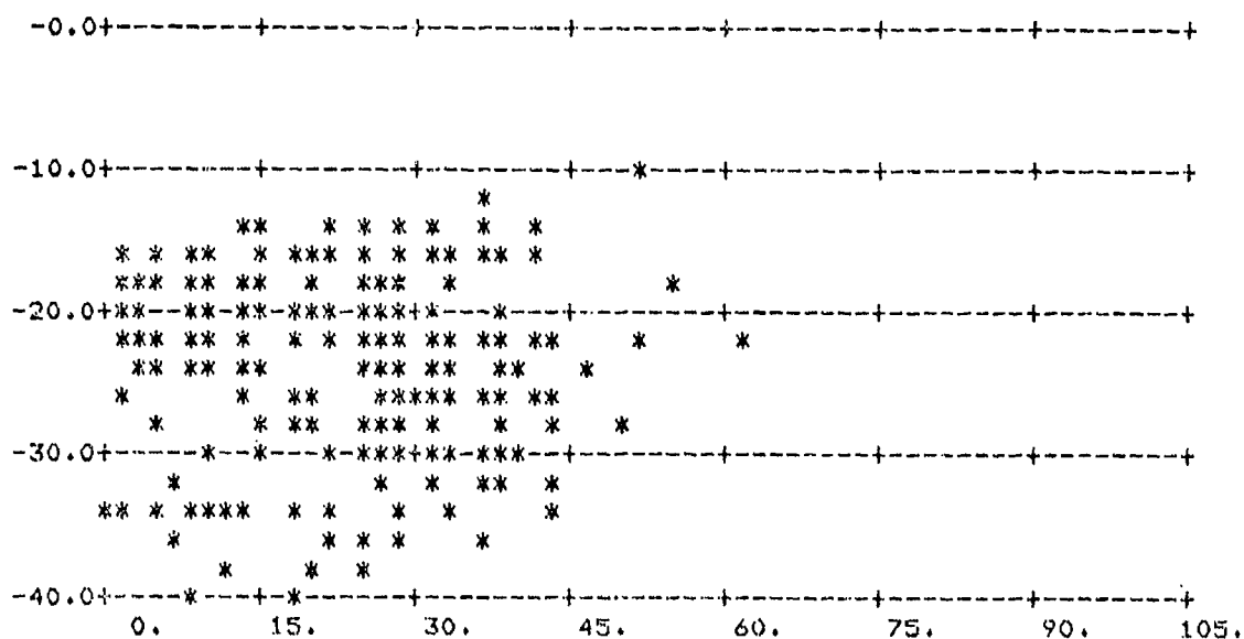
FIGURE A-13. \sigma_O vs \phi_S ; \theta_S = 84^\circ , \theta_I = 60^\circ
