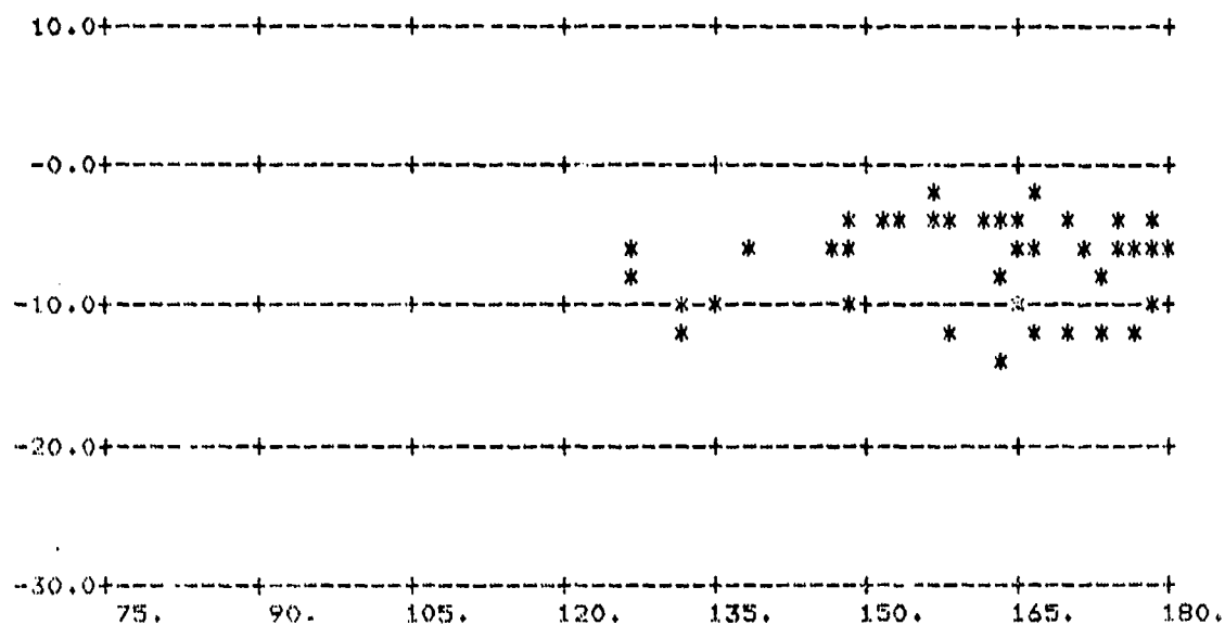
FIGURE A-96. \sigma_0 vs \phi_s ; \theta_s = 84^\circ , \theta_i = 80^\circ
