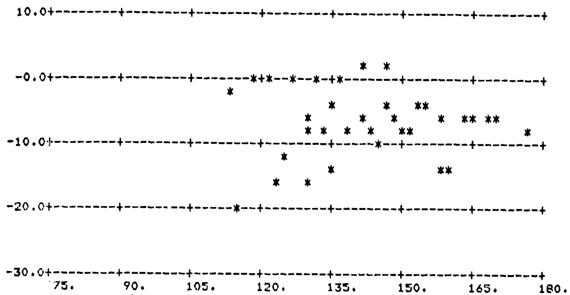
FIGURE A-142. \sigma_0 vs \phi_s ; \theta_s = 60^\circ , \theta_t = 60^\circ
