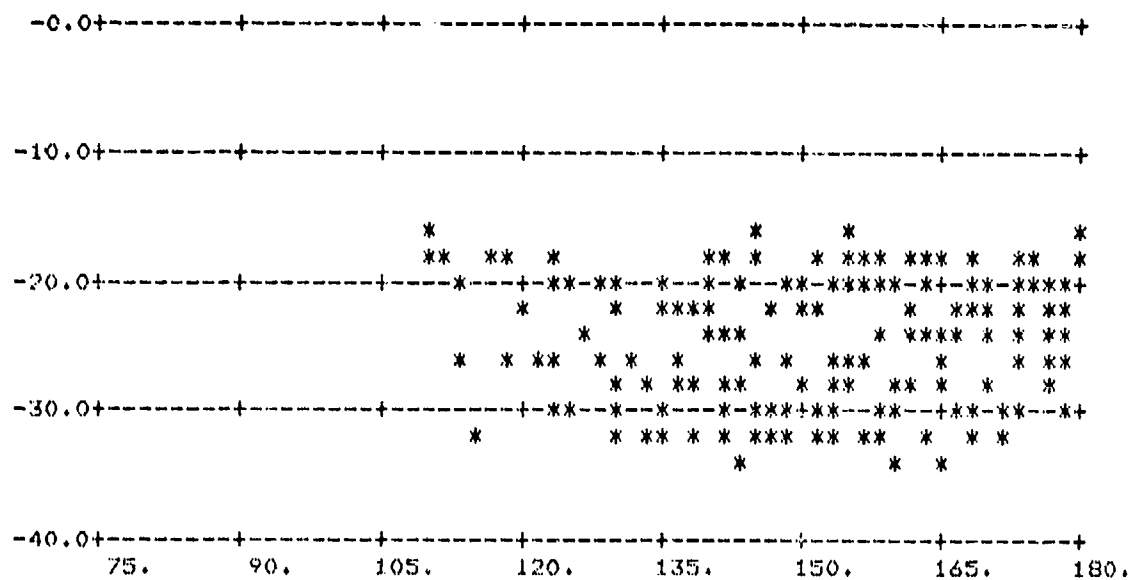
FIGURE A-101. \sigma_O vs \phi_s ; \theta_s = 60^\circ , \theta_i = 60^\circ
