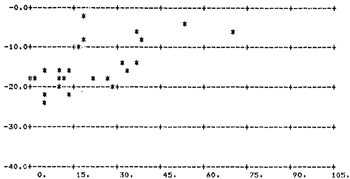
FIGURE A-77. \sigma_0 vs \phi_s ; \theta_s = 84^\circ , \theta_i = 70^\circ
