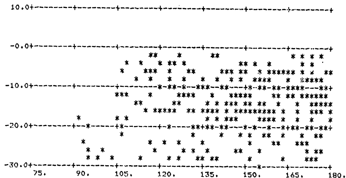
FIGURE A-40. \sigma_0 vs \phi_s ; \theta_s = 70^\circ , \theta_i = 80^\circ
