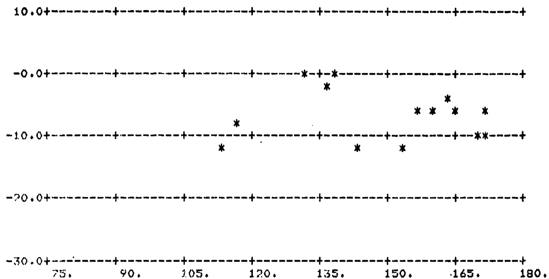
FIGURE A-66. \alpha_0 vs \phi_s ; \theta_s = 60^\circ , \theta_i = 70^\circ
