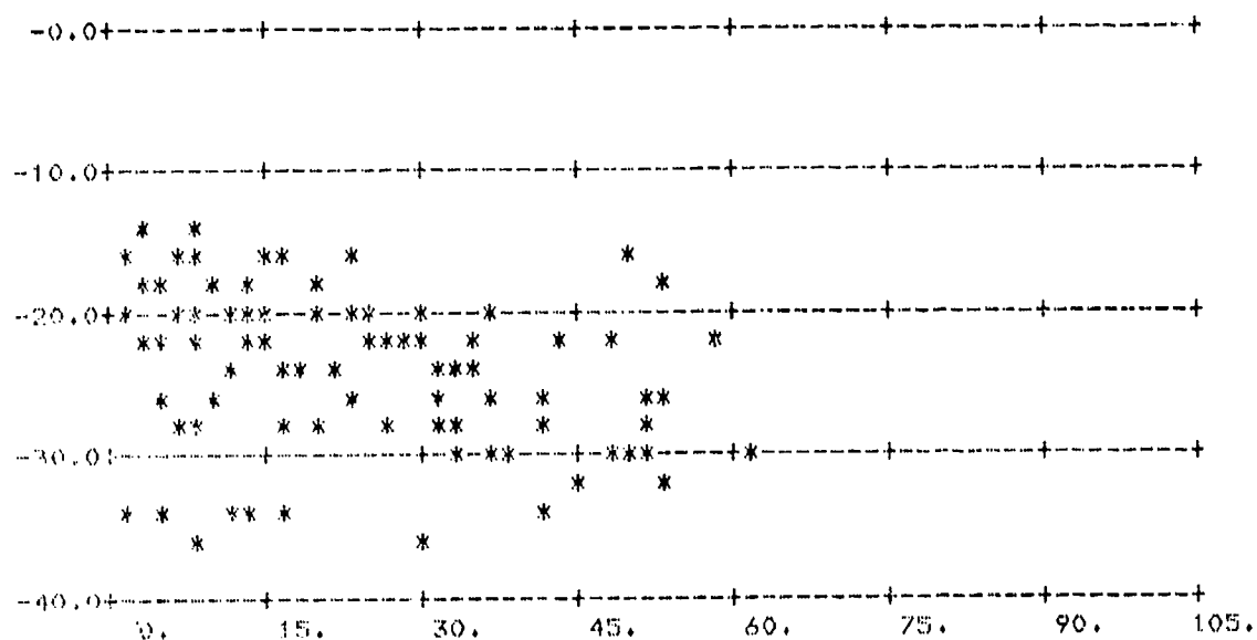
FIGURE A-131. \sigma_0 vs \phi_s ; \theta_s = 60^\circ , \theta_1 = 80^\circ
