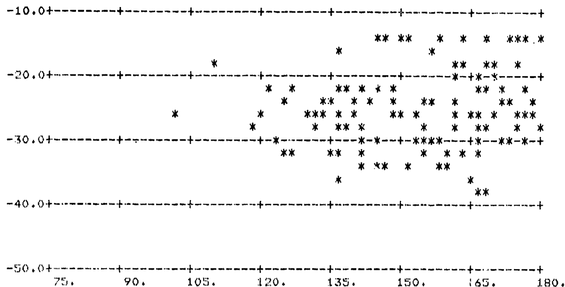
FIGURE A-136. \sigma_O vs \phi_S ; \theta_S = 70^\circ \theta_1 = 80^\circ
