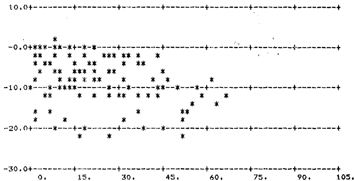
FIGURE A-55. \sigma_0 vs \phi_s ; \theta_s = 70^\circ , \theta_i = 60^\circ
