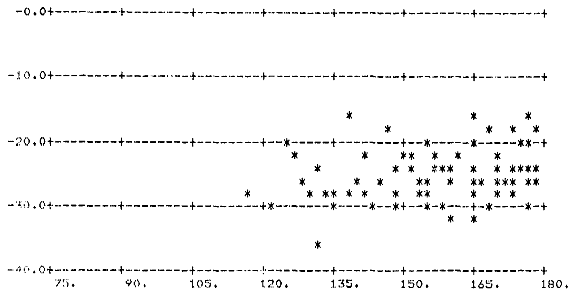
FIGURE A-120. \sigma_0 vs \phi_s ; \theta_s = 60^\circ , \theta_i = 70^\circ
