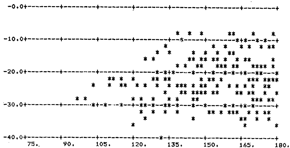
FIGURE A-36. \sigma_0 vs \phi_0 ; \theta_s = 60^\circ , \theta_i = 80^\circ
