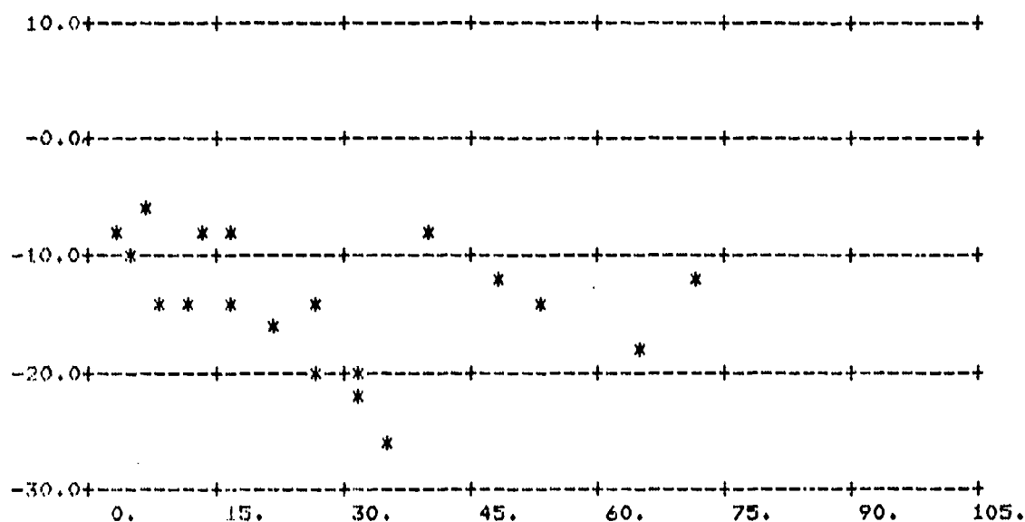
FIGURE A-67. \sigma_0 vs \phi_s ; \theta_s = 60^\circ , \theta_i = 70^\circ
