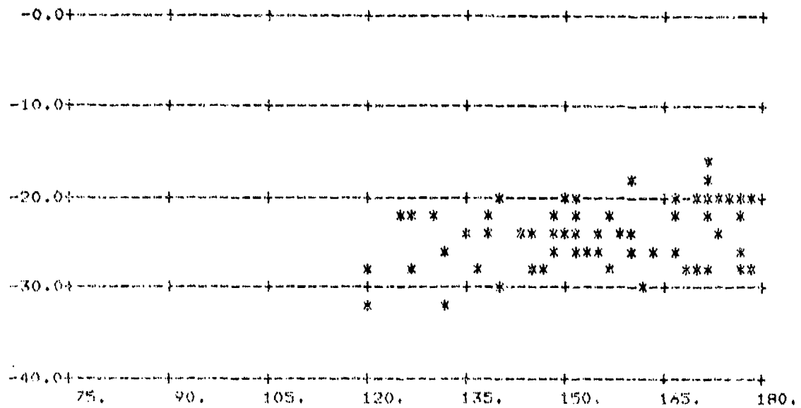
FIGURE A-14C. \sigma_0 vs \phi_0 ; \theta_s = 80^\circ , \theta_i = 80^\circ
