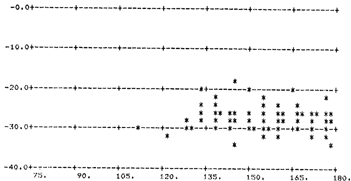
FIGURE A-128. \sigma_O vs \phi_s ; \theta_s = 80^\circ , \theta_i = 70^\circ
