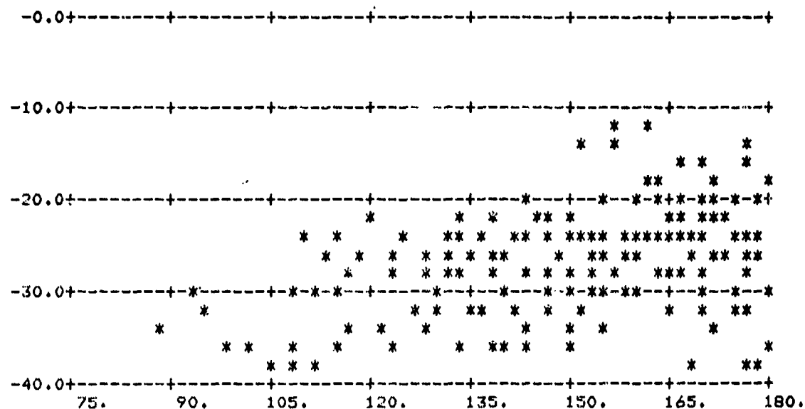
FIGURE A-18. \alpha_0 vs \phi_s ; \theta_s = 60^\circ , \theta_i = 70^\circ
