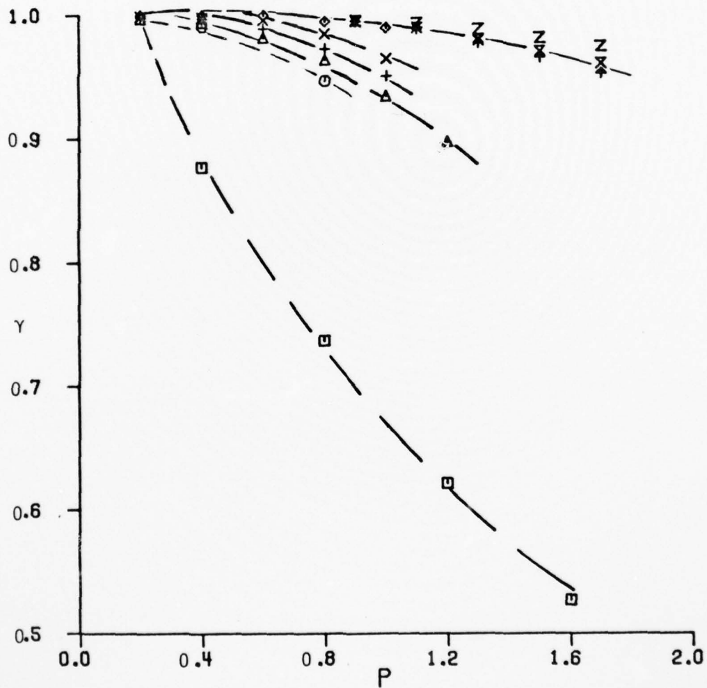
Figure 3-24. \gamma vs. P at x/D = 45 , y/b = 0 .
