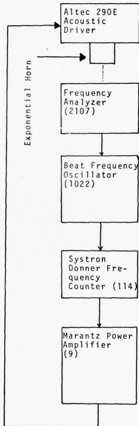
Figure 3-10. Schematic of Instrumentation for Acoustic Excitation.
