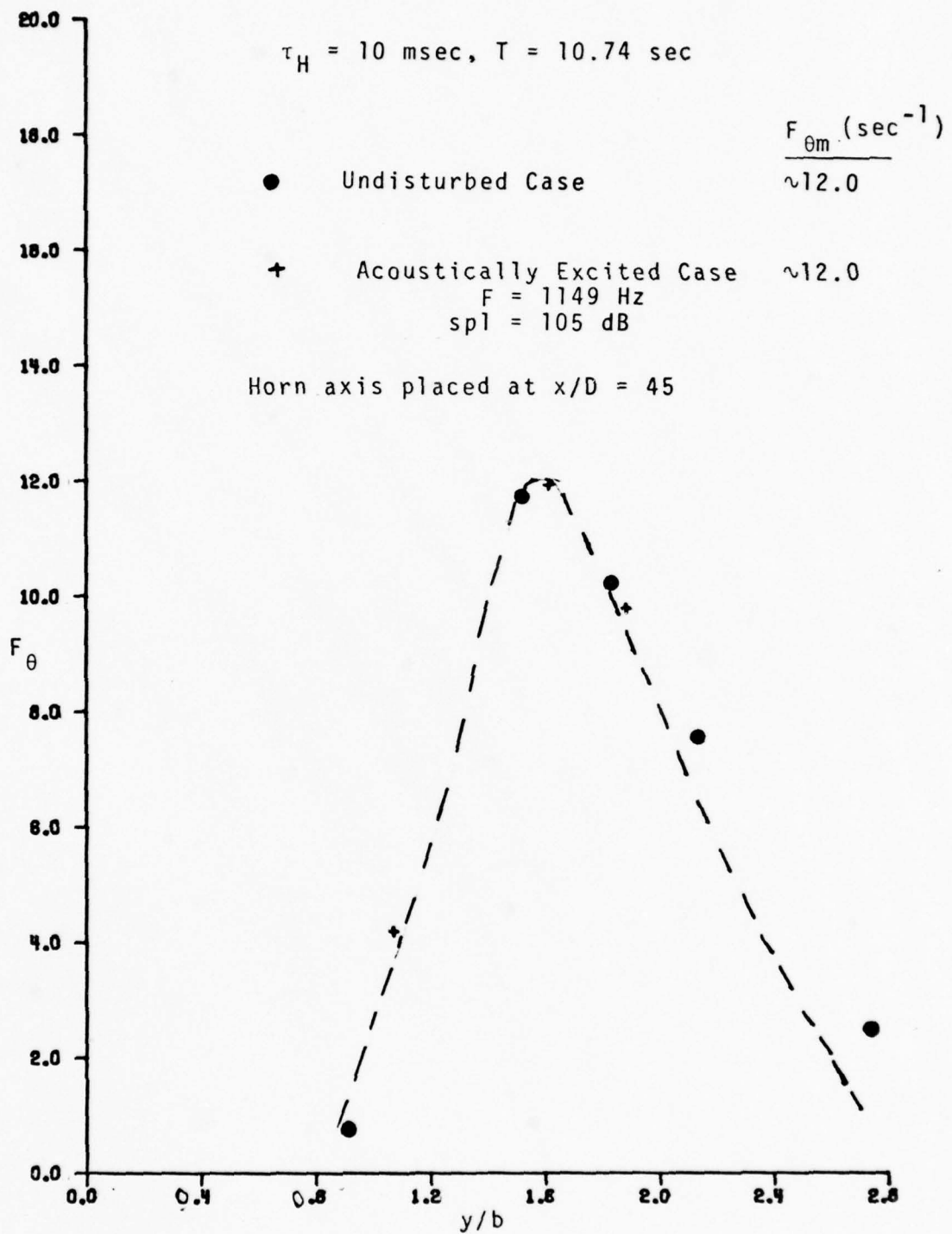
Figure 4-16. Fold-Over Frequency vs. y/b at x/D = 35 .
