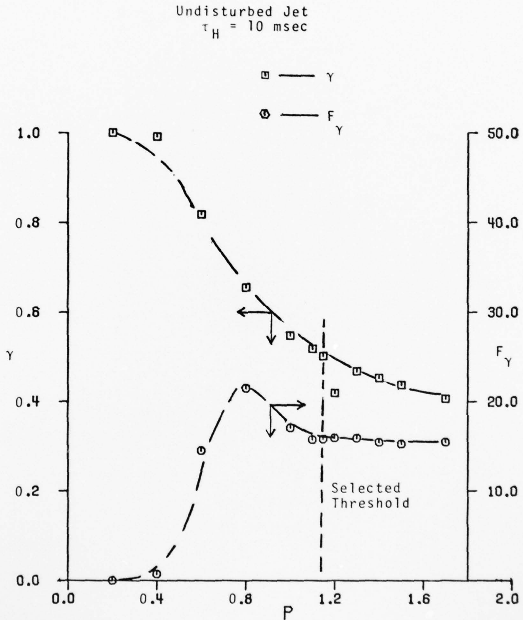
Figure 3-28. \gamma and F_\gamma vs. P at x/D = 45 , y/b = 1.61 , \tau_H = 10 msec.
