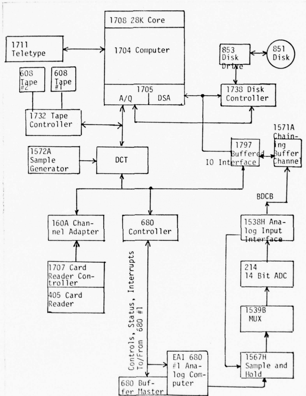
Figure A-3. Schematic of Hybrid Computer System.
