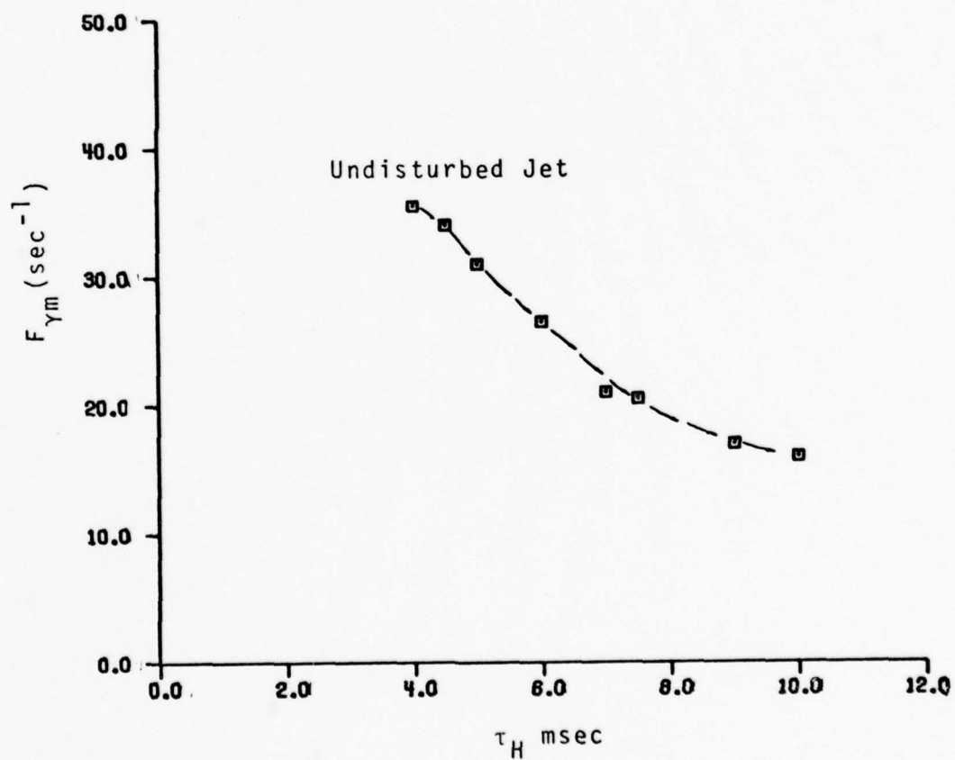
Figure 5-1. Maximum Crossing Frequency vs. \tau_H at y/b = 1.61 , \gamma = 0.5 .
