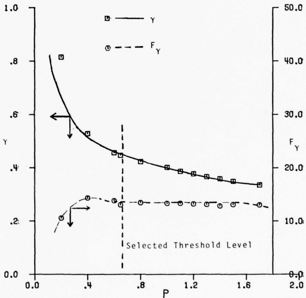
Figure 3-17. \gamma and F_\gamma vs. P at x/D = 45 , y/b = 1.66 .
