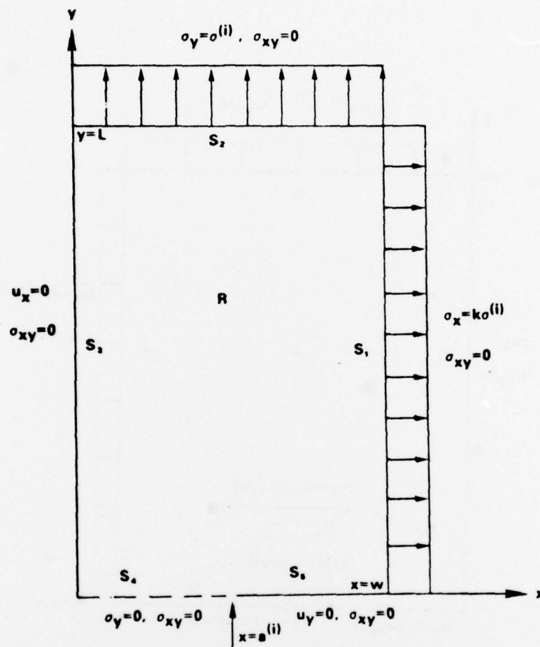
Fig. 4 Boundary Conditions of l -th State
