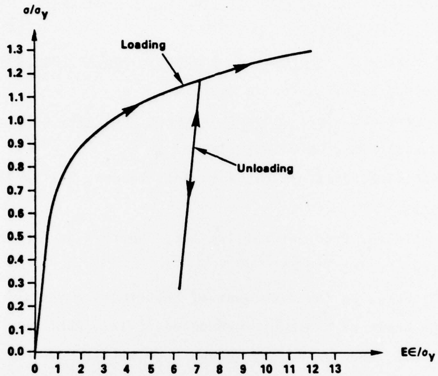
Fig.1 Stress - Strain Relation in Simple Tension Test
