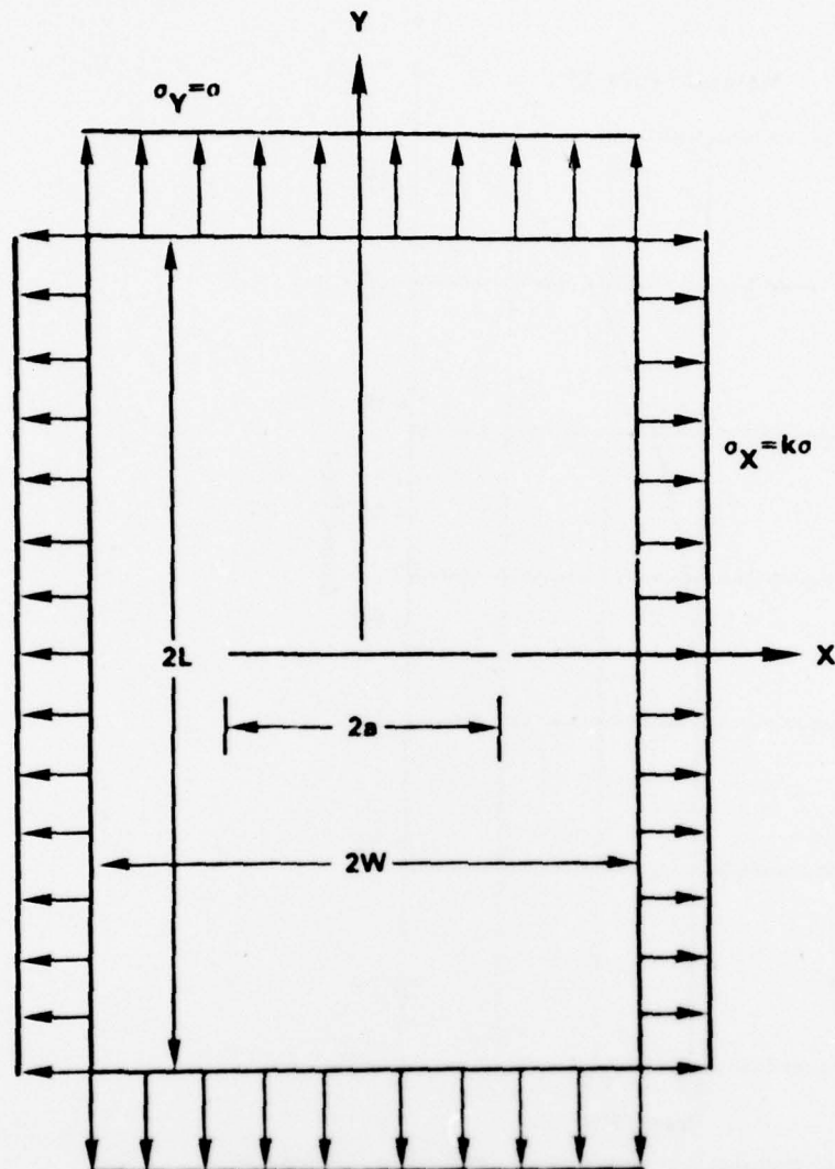
Fig. 2 Center - Cracked Specimen
