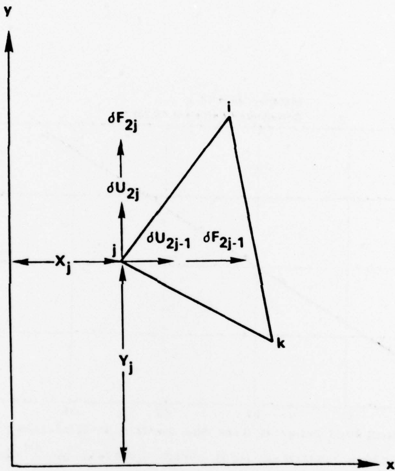
Fig. 6 Coordinates, Incremental Displacements and Forces of the j -th Nodal Point
