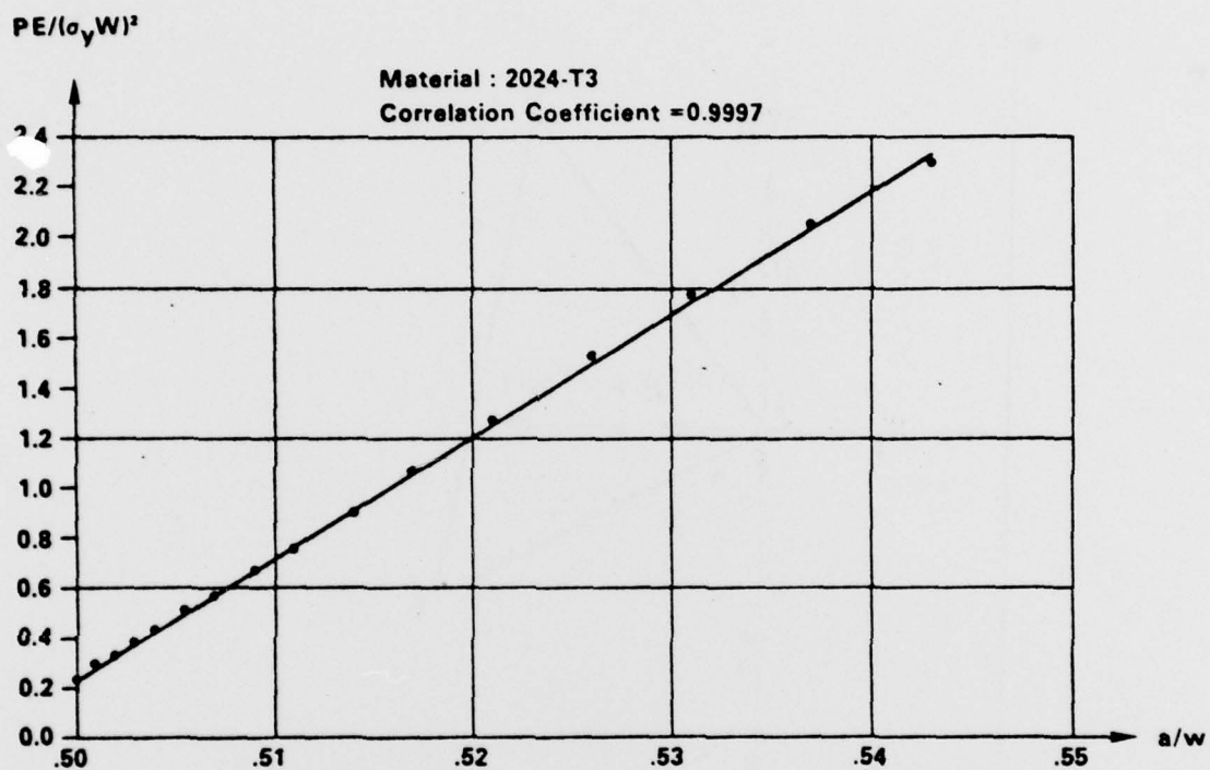
Fig. 7 Plastic Strain Energy vs Crack Size; 2w=12 in., 2L=32 in., 2a_0=6 in.,
