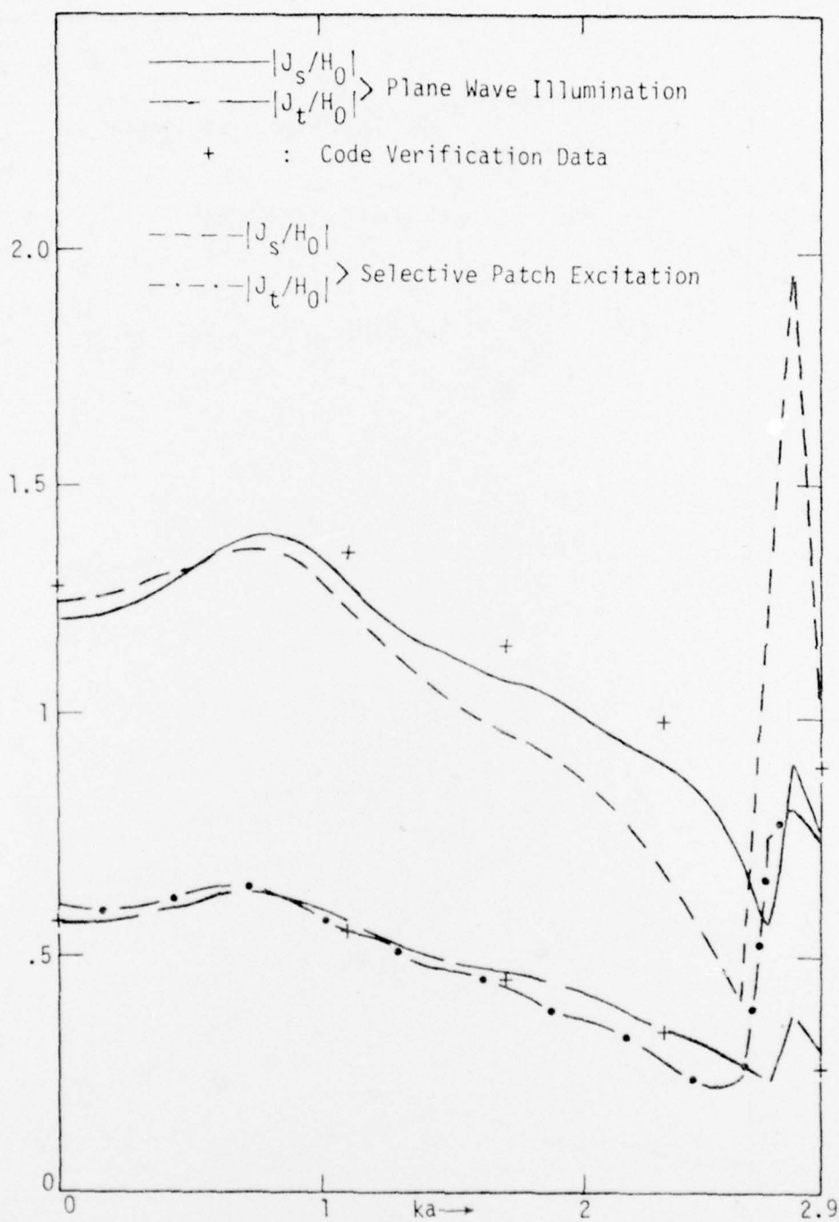
Figure 6. Normalized Current Densities on Patch 4. Selective Patch Excitation is Obtained by Exciting all Patches but Nos. 2, 3, 14, 15, 18, 19, 30, 31.
