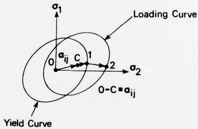
Fig. 3 - Kinematic hardening in plane stress.
