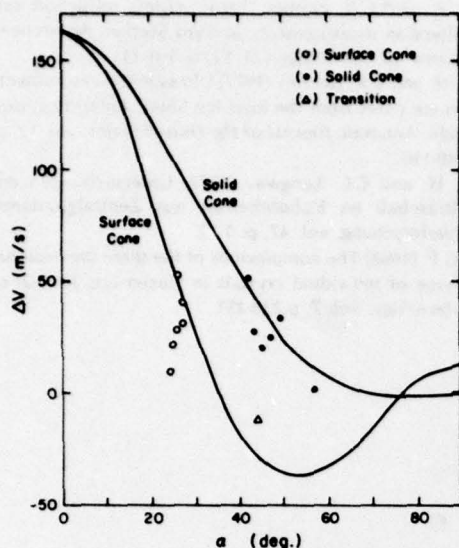
Figure 11. Plot of the P-wave velocity differences \Delta V vs the half-apex cone angles \alpha for ice cores from Little America V, Ross Ice Shelf, Antarctica. \Delta V curves for solid and surface cones were calculated from Bennett (1972).
