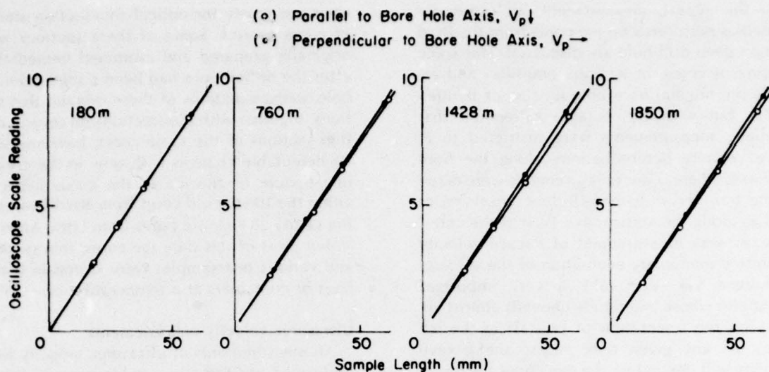
Figure 2. Travel time curves for core samples from different depths at Byrd Station. One oscilloscope scale unit measures approximately 1.75 microseconds. Divergence of travel time curves is directly related to the anisotropic state (oriented condition) of the ice crystals in the cores.
