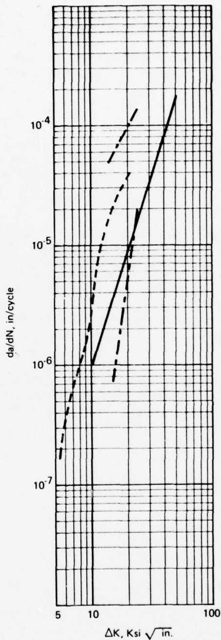
Figure 51.—Comparison of Environmental FCP Behavior of Phase III DA Sheet to MA Sheet. — Phase III DA Sheet, R = .05 , f = 60 cpm, T-L Orient, 3.5% NaCl --- MA Sheet, R = .08 , f = 60 cpm, T-L Orient, Sump Tank Water, Ref. 11, pg. A-113 - - - Phase I MA Sheet, R = .05 , f = 60 cpm, T-L Orient, 3.5% NaCl
