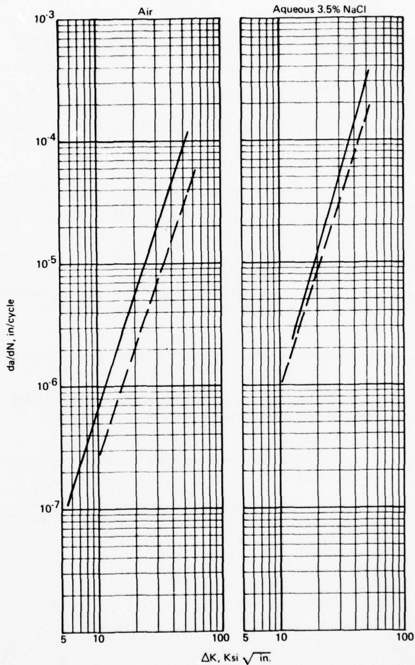
Figure 52.—Comparison of FCP Behavior of Phase III DA Sheet as a Function of R Ratio, f = 60 cpm, Tested in Transverse Direction.
