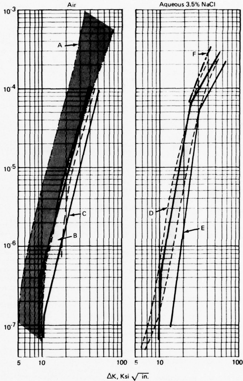
Figure 42.—Comparison of BA and RA Plate FCP Behavior. A — MA Plate, R = .08 , f = 60-1500 cpm, L-T - Orient, Air, Ref. 22, pp. 8.44, 5, 7, 8 B — RA Plate, R = .08 , f = 360 cpm, T-L Orient, Air, Ref. 11, p. 8-398 C — Phase III BA Plate, R = .05 , f = 60 cpm, T-L Orient, Air D — RA Plate, R = .08 , f = 60 cpm, T-L Orient, Sump Tank Water, Ref. 11, p. 8-403 E — Phase III BA Plate, R = .05 , f = 60 cpm, T-L Orient, 3.5% NaCl F — RA Plate, R = .1 , f = 6 cpm, T-L Orientation, Ref. 23
