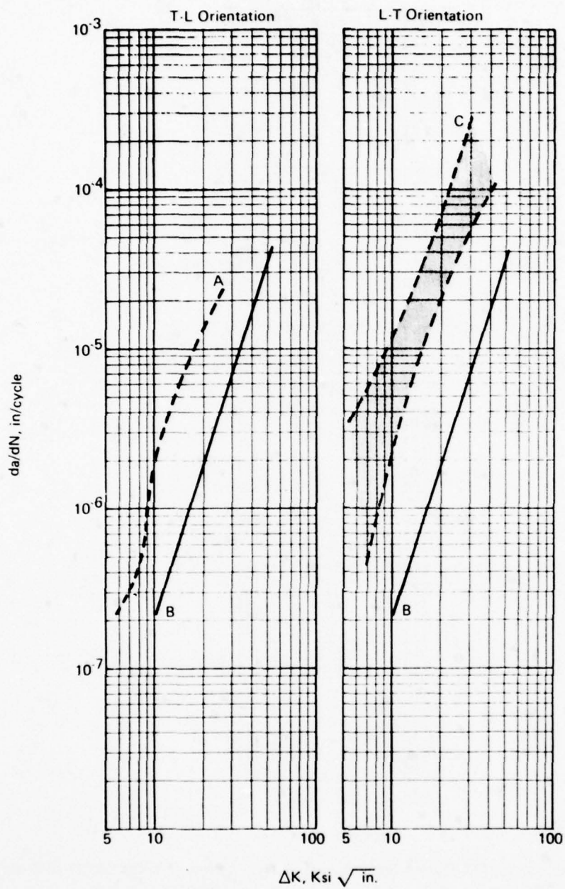
Figure 50.—Comparison of FCP Behavior of Phase III DA Sheet to MA Sheet In Air. A — MA Sheet, R = .08 , f = 60 cpm, Ref. 11, Pg. A-108 B — Phase III, D.A. Sheet, R = .05 , f = 60 cpm C — MA Sheet, R = .08 , f = 60 to 360 cpm, Ref. 22, pp. 8.4-94, 98, 100
