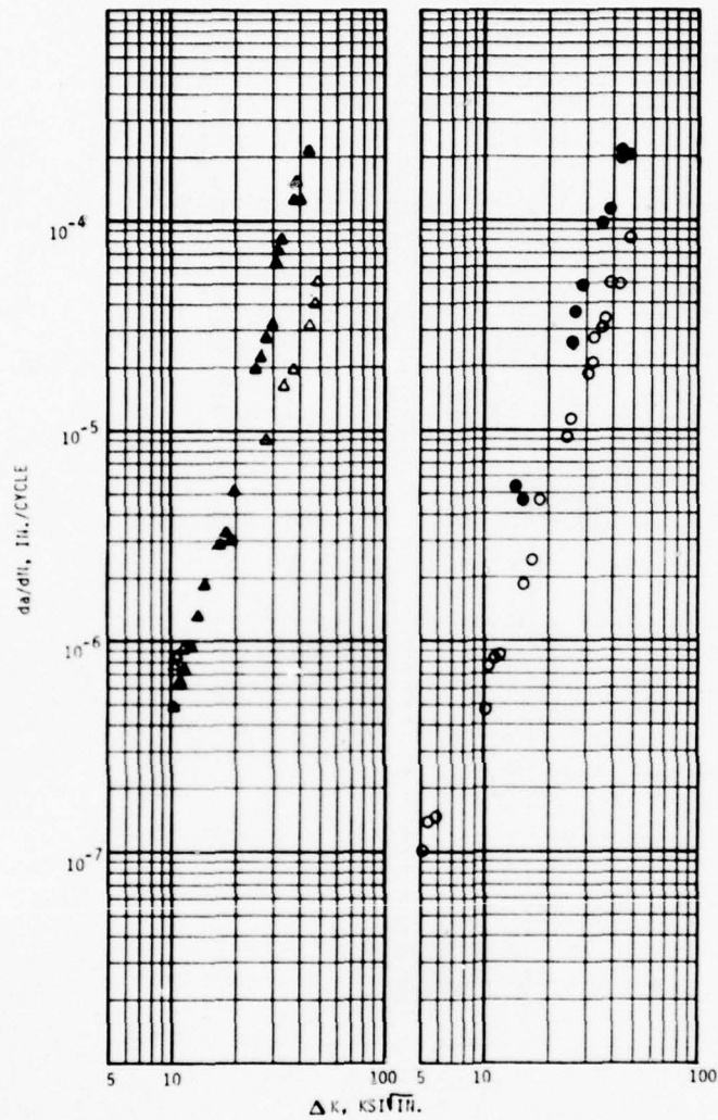
Figure B6.—Fatigue Crack Propagation Rate Vs. Stress Intensity Range for Ti-6Al-4V Sheet (Phase III Material).
