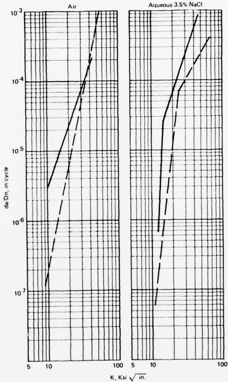
Figure 47.—Comparison of FCP Behavior of BA Plate at R = 0.05 and 0.5 in Air and Salt Water, f = 60 \text{ cpm} , T-L Orientation.
