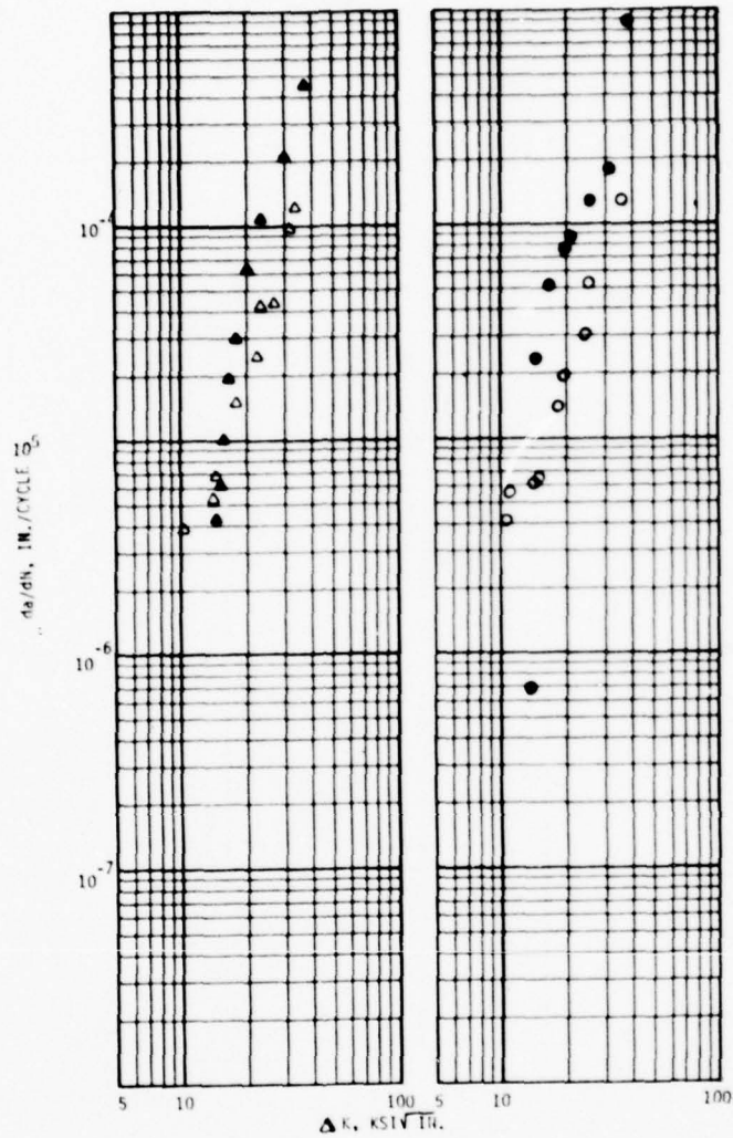
Figure B3.—Fatigue Crack Propagation Vs. Stress Intensity Range for Ti-6Al-4V Plate (Phase III Material).
