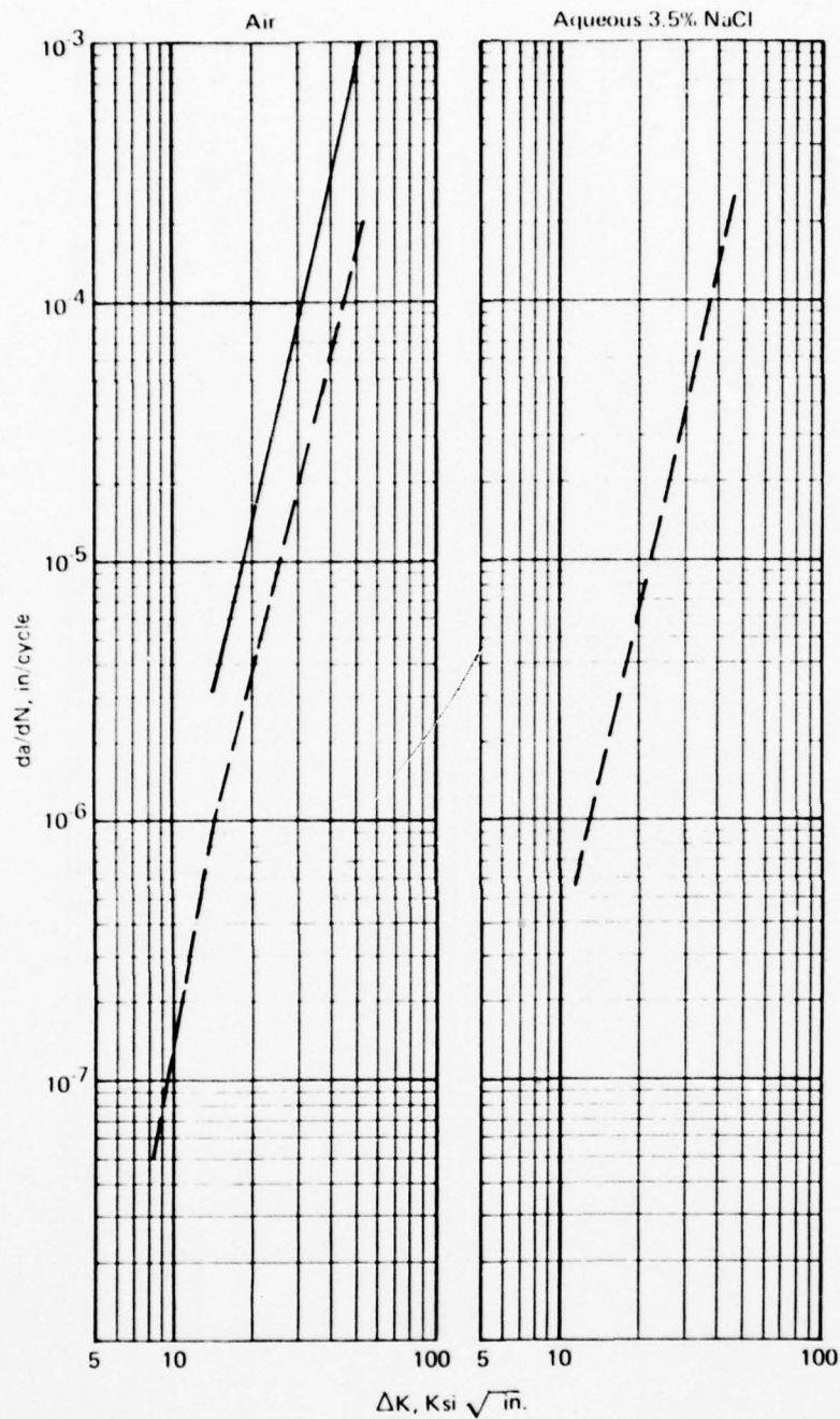
Figure 48.—Comparison of FCP Behavior of BA Plate at R = 0.05 and 0.5 in Air and Salt Water, f = 6 cpm, T-L Orientation.
