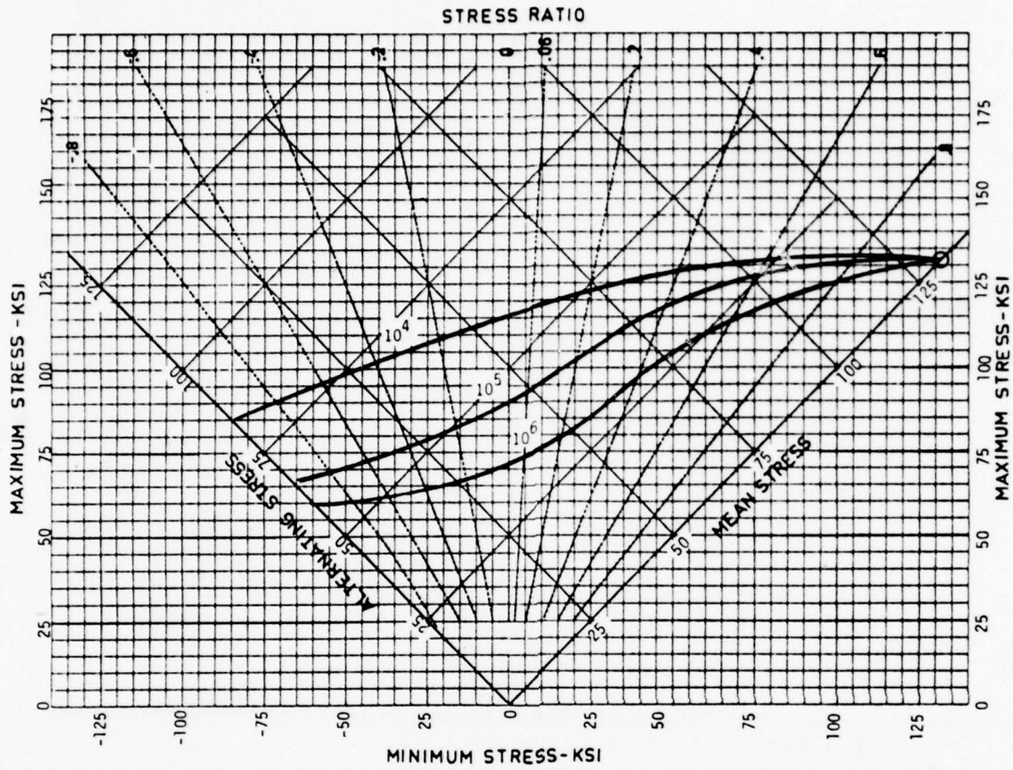
Figure B8.—Constant-life Diagram for Phase III BA Plate Tested at Room Temperature, K_t = 1 , f = 1800 cpm.
