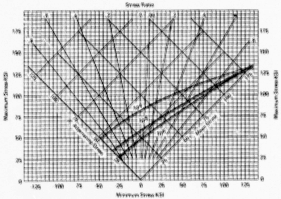
Figure 36.—Constant life Diagram for Phase III BA Plate Tested at Room Temperature, K_f = 2.53 , f = 1000 cpm.
