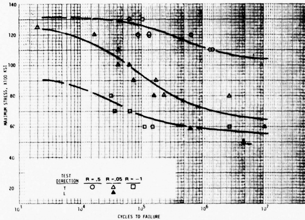
Figure B7.—Fatigue Life of Beta-annealed Ti-6Al-4V Alloy Plate in Air, at Room Temperature, 1800 cpm, K_t = 1 .
