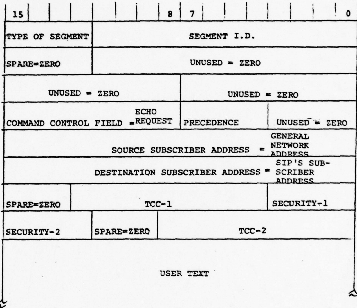
SCM - TO - SIP ECHO REQUEST SEGMENT
