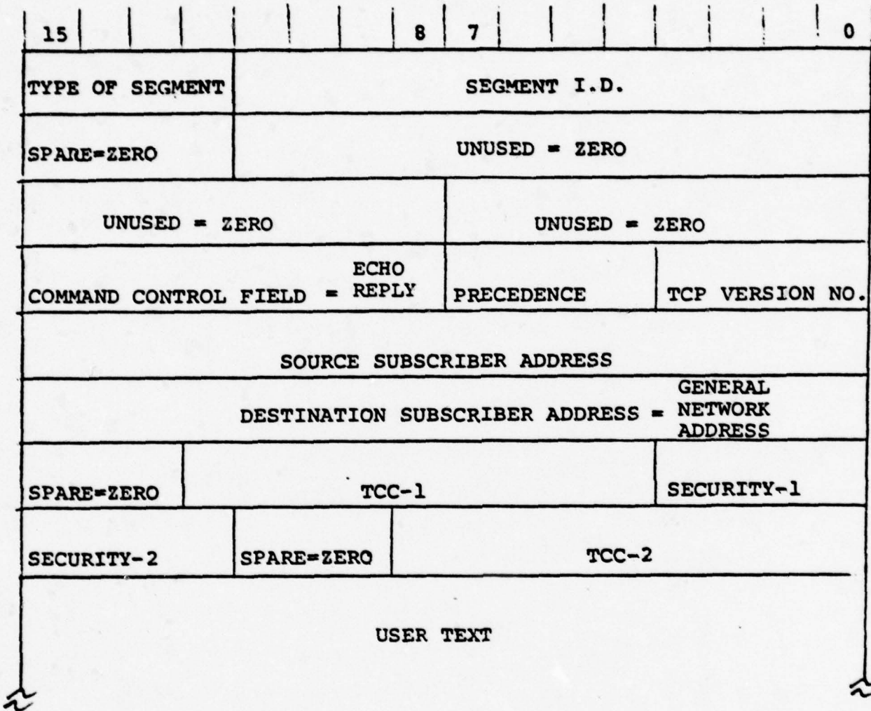
SIP - TO - SCM ECHO REPLY SEGMENT
