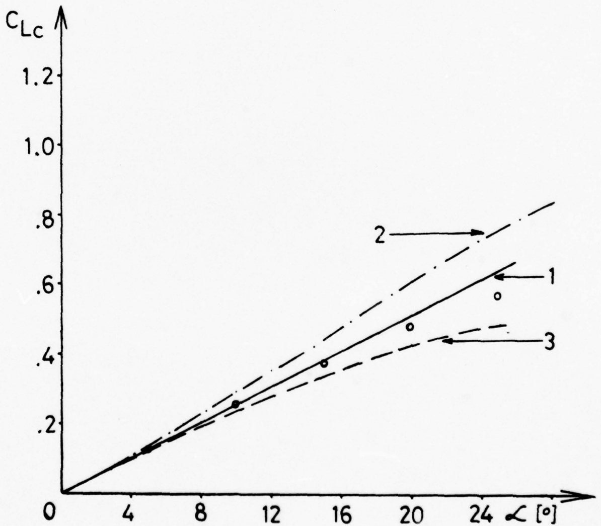
FIGURE 14 - COMPARISON OF EXPERIMENTAL RESULTS TO VARIOUS THEORETICAL RESULTS FOR CONFIGURATION No.2.
