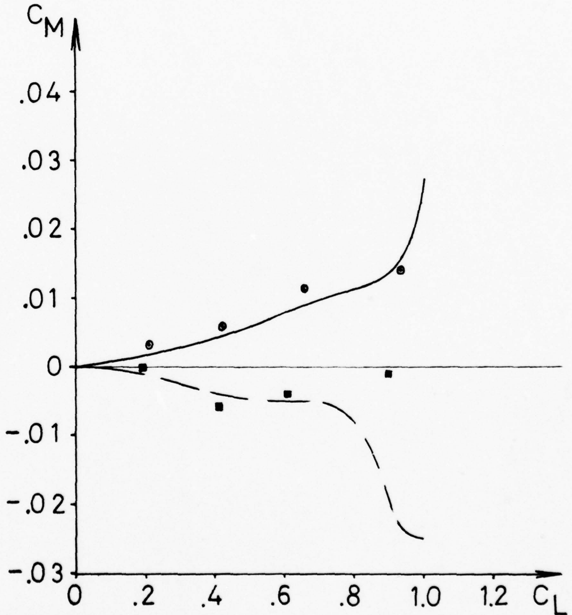
FIGURE 4 - PITCHING MOMENT COEFFICIENT Vs. LIFT COEFFICIENT FOR HIGH AND LOW CANARDS, CONFIGURATION No. 1.
