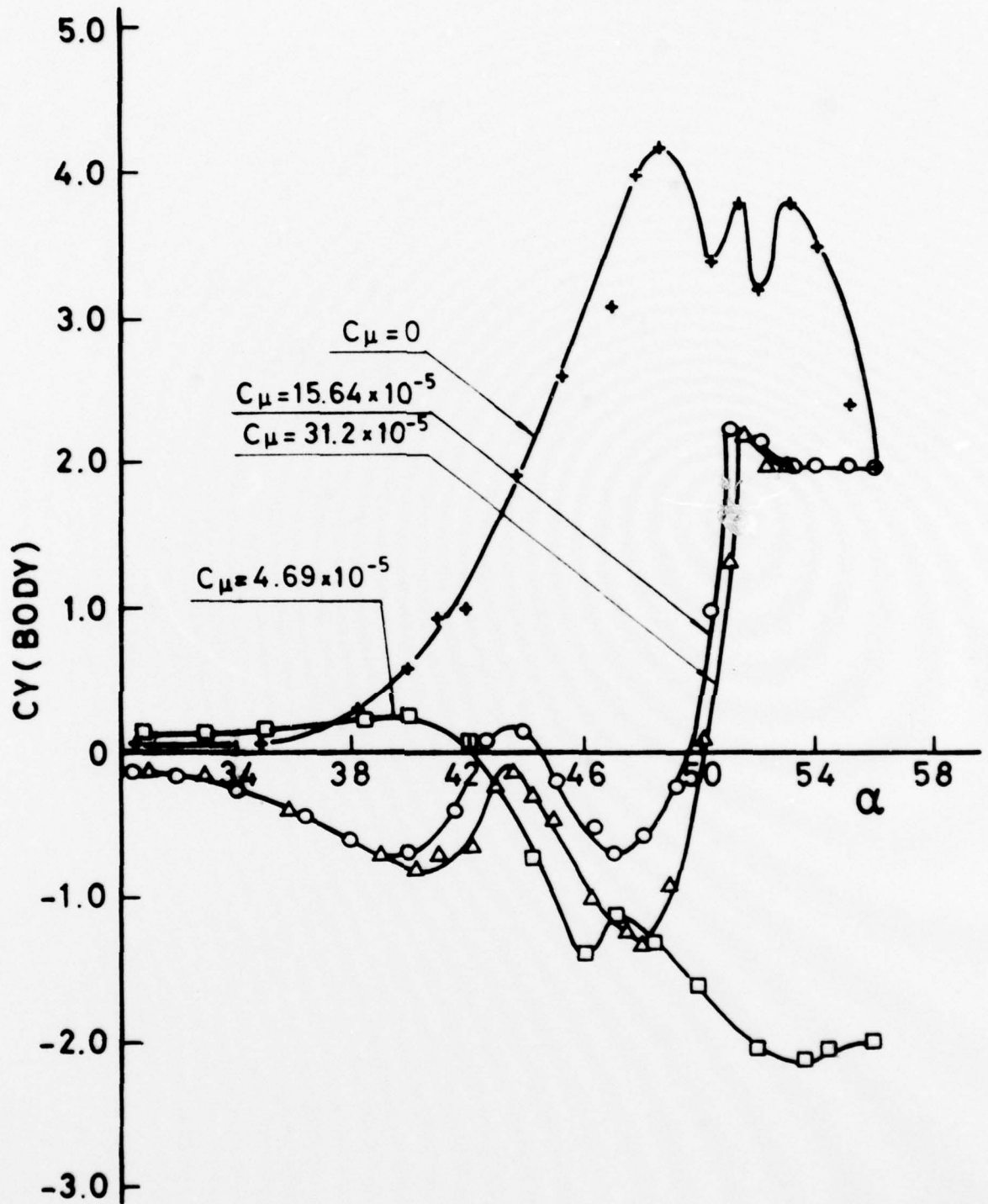
FIG.28-SIDE FORCE COEFFICIENT VERSUS ANGLE OF ATTACK FOR INJECTION AT STA. I ANGLE -30° ( POINTED CONE V = 20 \frac{m}{sec} )
