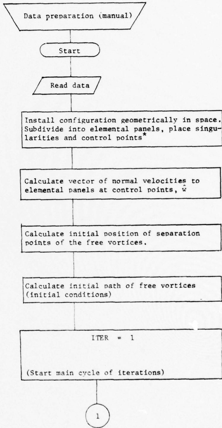
FIGURE 23 - SCHEMATIC FLOW-CHART OF THE CALCULATION, (PRESENT METHOD).
