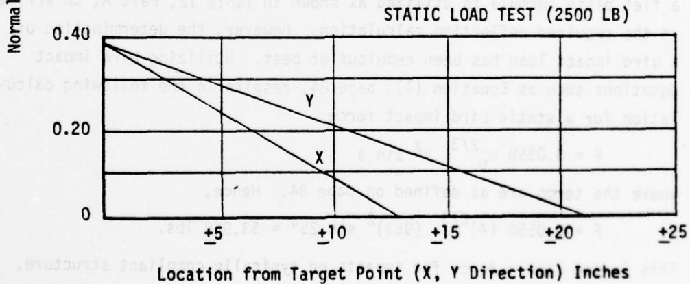
Figure 42. B-1 Windshield Deflection, Test Number BM006.
