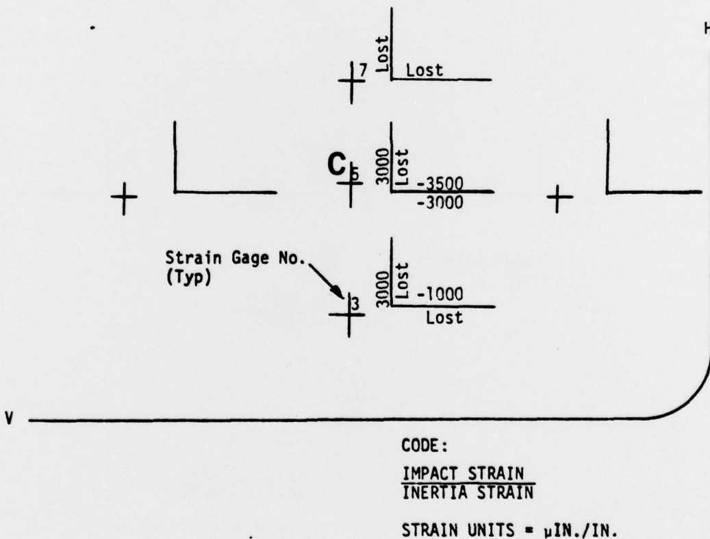
Figure B.21. Test Windshield Strain Map - Test BM019 - Gages 3, 5, 7.
