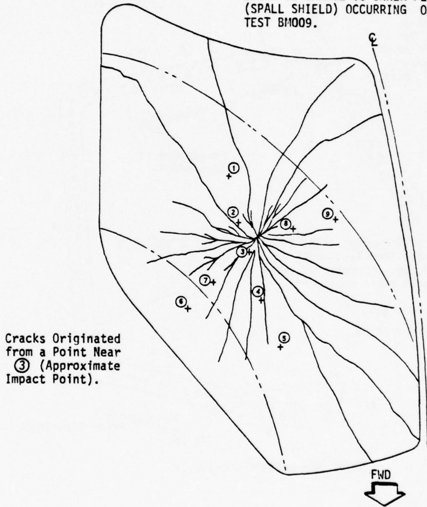
Figure A.4. B-1 windshield test specimen (SWU107), inner ply surface, post-test BM009.
