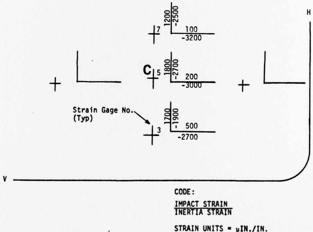
Figure B.27. Test Windshield Strain Map - Test BM014 - Gages 3, 5, 7.
