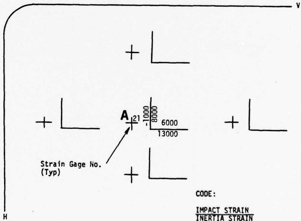
Figure B.17. Test Windshield Strain Map - Test BM013 - Gage 21.
