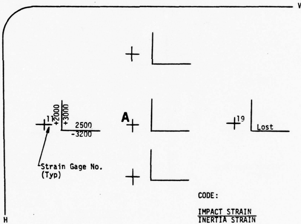
Figure B.7. Test Windshield Strain Map - Test BM012 - Gages 11, 19.
