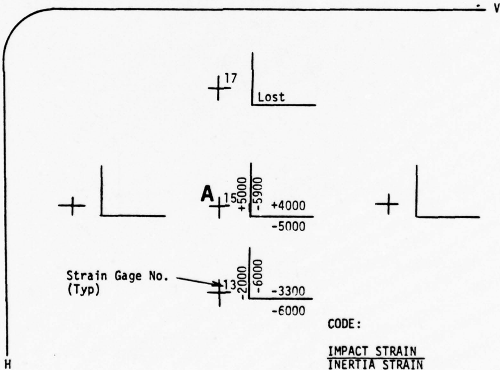
Figure B.9. Test Windshield Strain Map - Test BM012 - Gages, 13, 15, 17.
