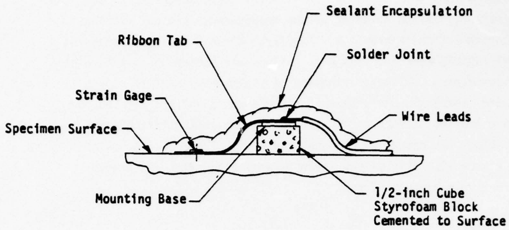
Figure 11. Styrofoam Block Shock Absorber.
