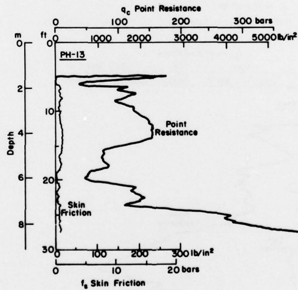
Figure B13. Point resistance and skin friction profiles, site PH-13.
