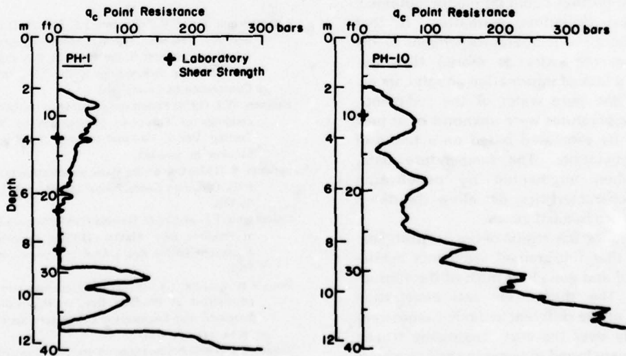
Figure 18. Comparison of triaxial test results with point resistance data at sites PH-1 and PH-10.
