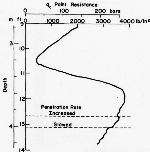
Figure 12. Expanded portion of site PH-16 point resistance.
