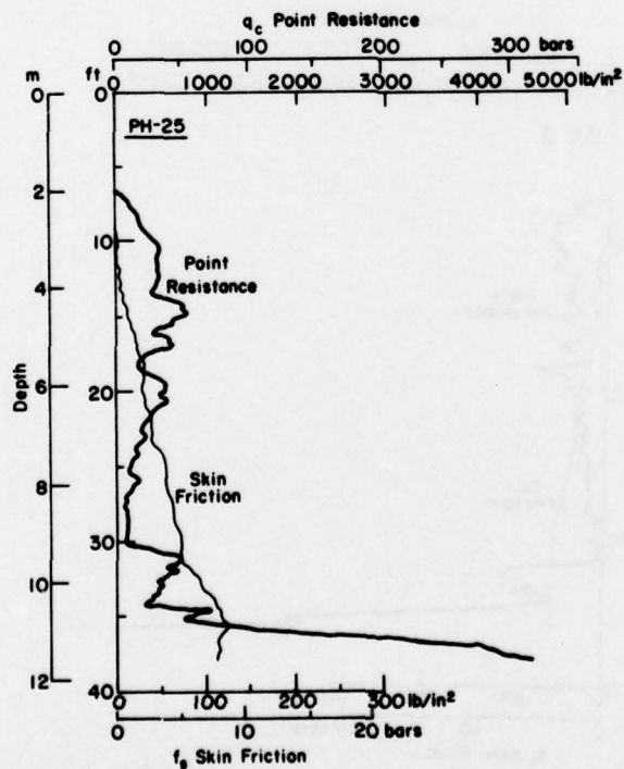
Figure B25. Point resistance and skin friction profiles, site PH-25.
