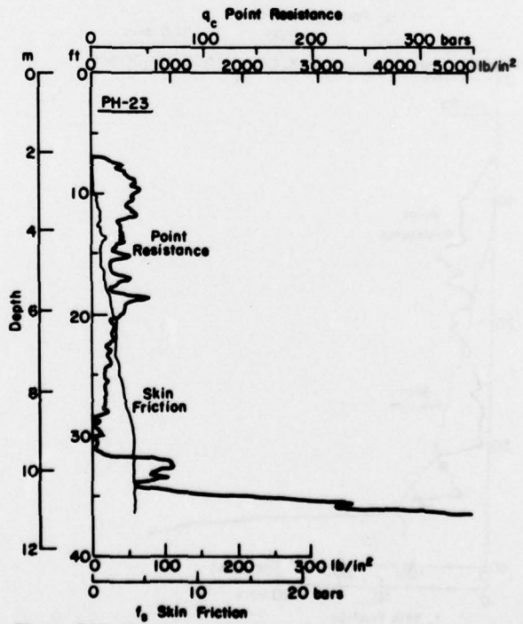
Figure B23. Point resistance and skin friction profiles, site PH-23.
