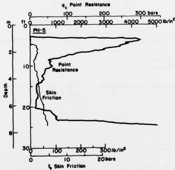
Figure B5. Point resistance and skin friction profiles, site PH-5.
