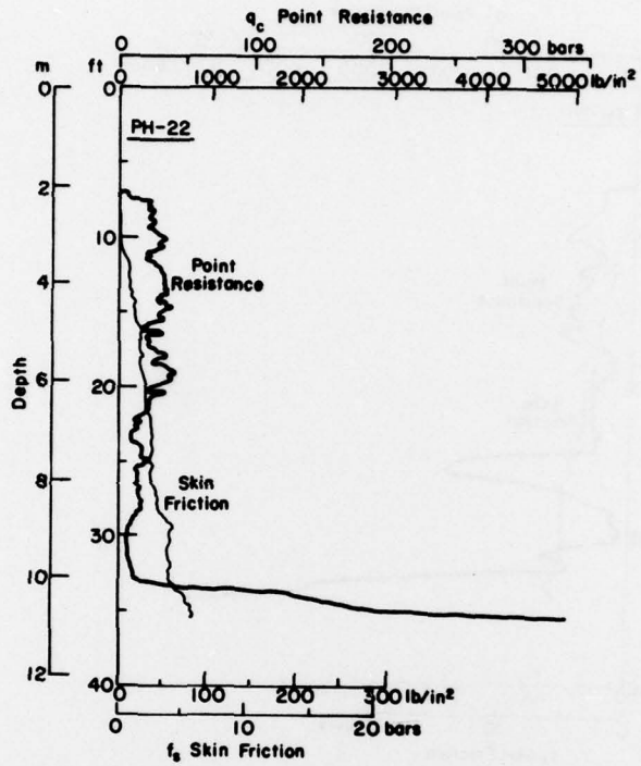
Figure B22. Point resistance and skin friction profiles, site PH-22.
