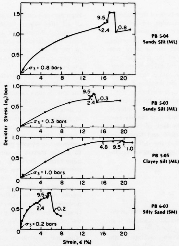
Figure 17. Results of staged triaxial tests for four test samples obtained from sites PB-5 and PB-6. (1 bar = 14.5 psi)
