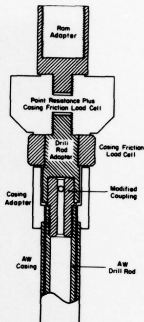
Figure A7. Diagram of force measuring system.
