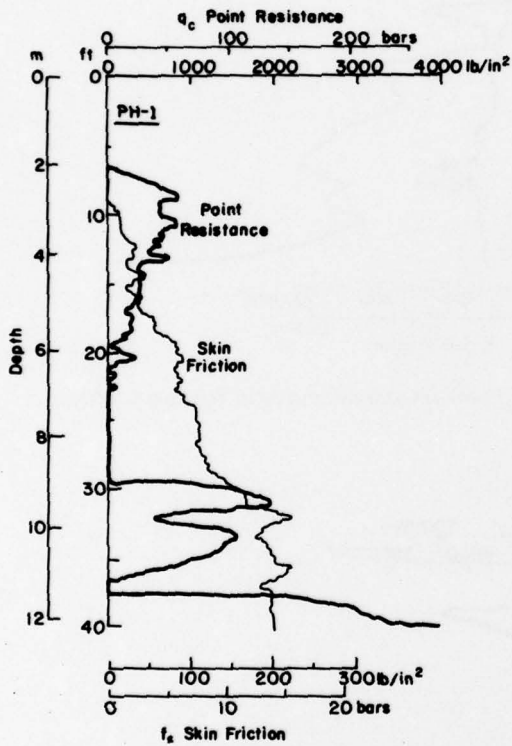
Figure B1. Point resistance and skin friction profiles, site PH-1.
