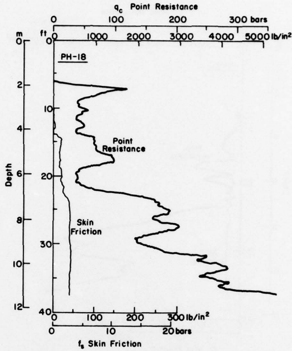
Figure B18. Point resistance and skin friction profiles, site PH-18.
