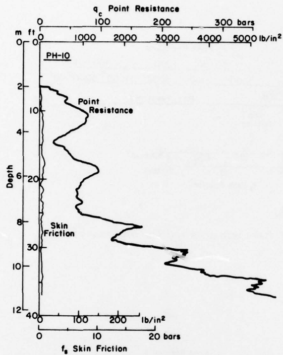
Figure B10. Point resistance and skin friction profiles, site PH-10.
