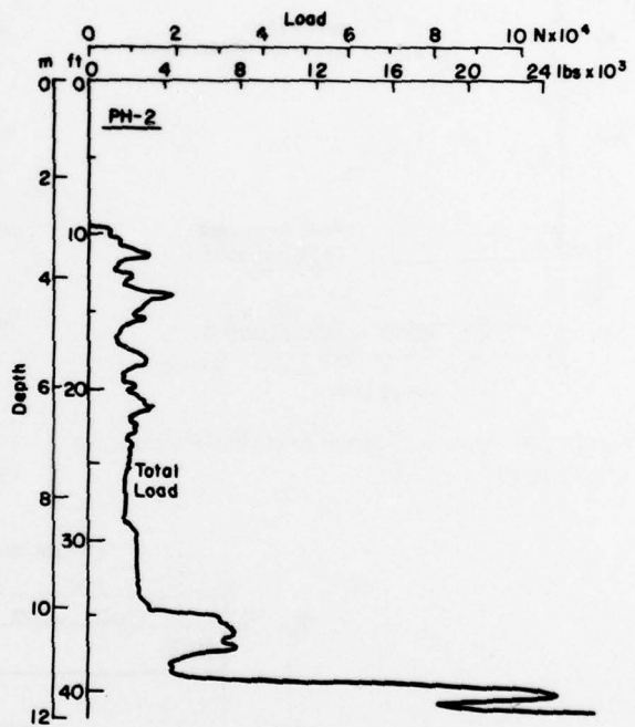
Figure B2. Point resistance and skin friction profiles, site PH-2.
