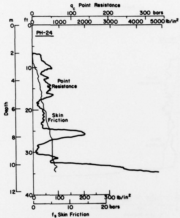
Figure B24. Point resistance and skin friction profiles, site PH-24.
