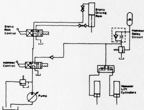
Figure A6. Schematic of hydraulic loading system.
