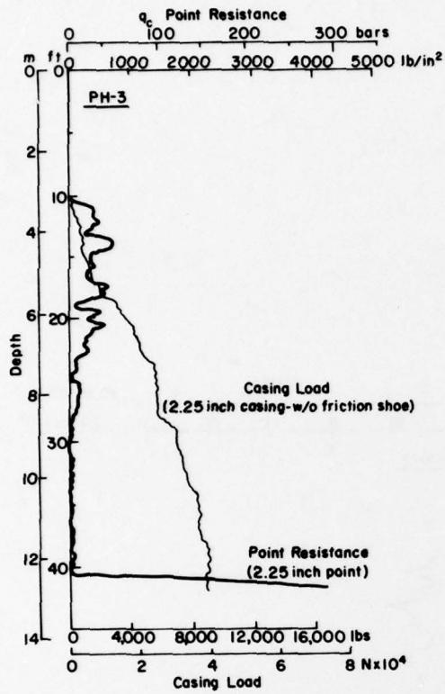
Figure B3. Point resistance and skin friction profiles, site PH-3.
