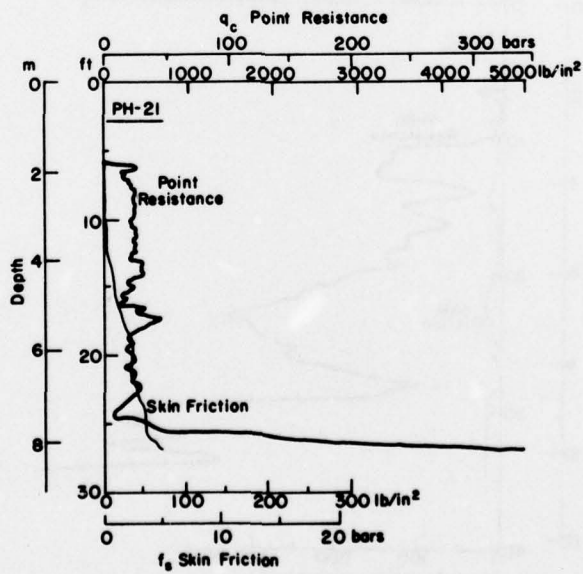
Figure B21. Point resistance and skin friction profiles, site PH-21.
