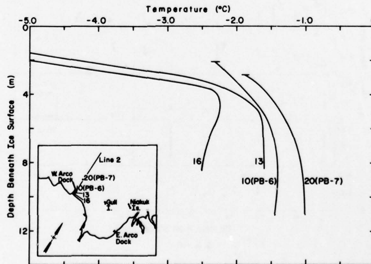
Figure 8. Temperature profiles, line 2.
