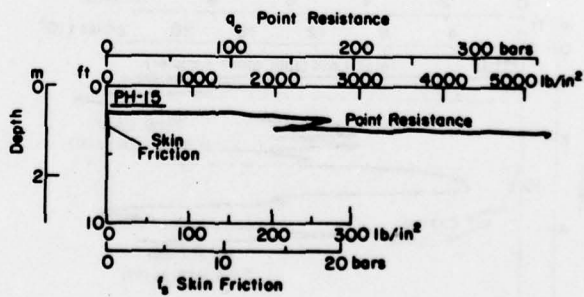
Figure B15. Point resistance and skin friction profiles, site PH-15.
