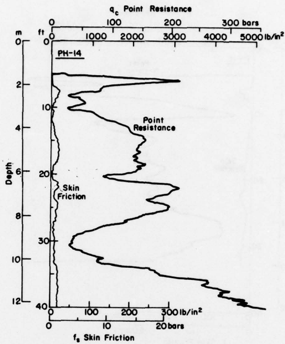
Figure B14. Point resistance and skin friction profiles, site PH-14.
