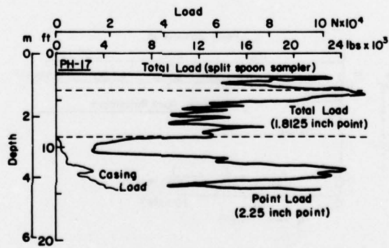
Figure B17. Point resistance and skin friction profiles, site PH-17.
