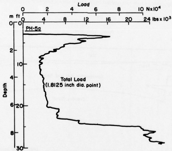
Figure 16. Results of special test at site PH-5a with small point.
