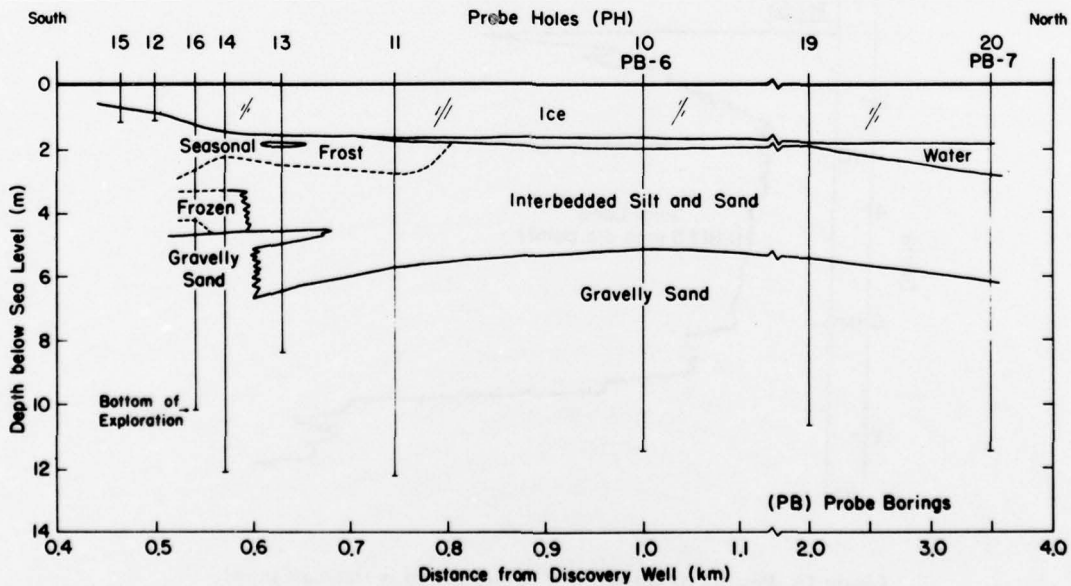
Figure 14. Stratigraphic profile interpreted from probe data along line 2. (1 m = 3.28 ft; 1 km = 0.62 mile)
