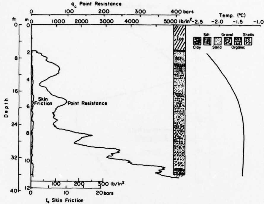
Figure 11. Comparison of point resistance and skin friction at probe PH-10 with geologic profile at drill site PB-6A.
