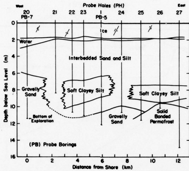
Figure 15. Stratigraphic profile interpreted from probe data along line 3. (1 m = 3.28 ft; 1 km = 0.62 mile)
