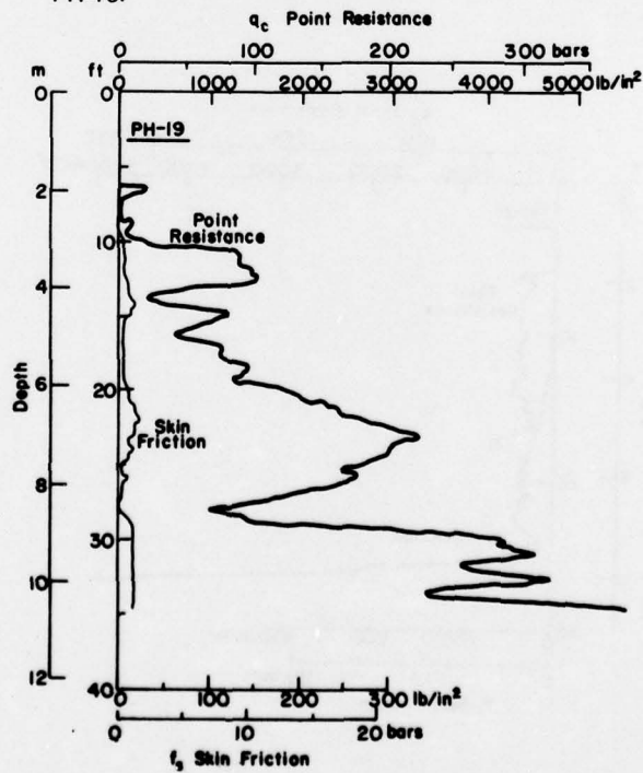
Figure B19. Point resistance and skin friction profiles, site PH-19.
