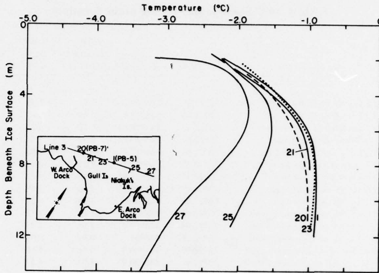
Figure 9. Temperature profiles, line 3.
