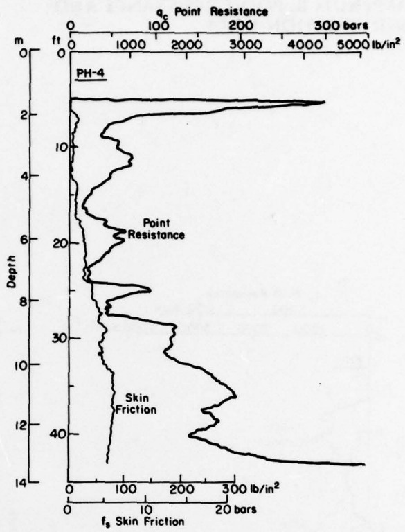
Figure B4. Point resistance and skin friction profiles, site PH-4.
