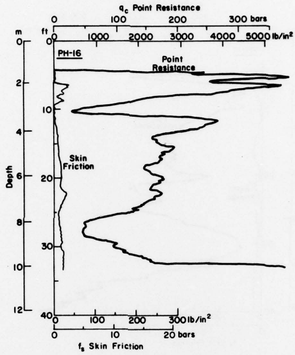
Figure B16. Point resistance and skin friction profiles, site PH-16.
