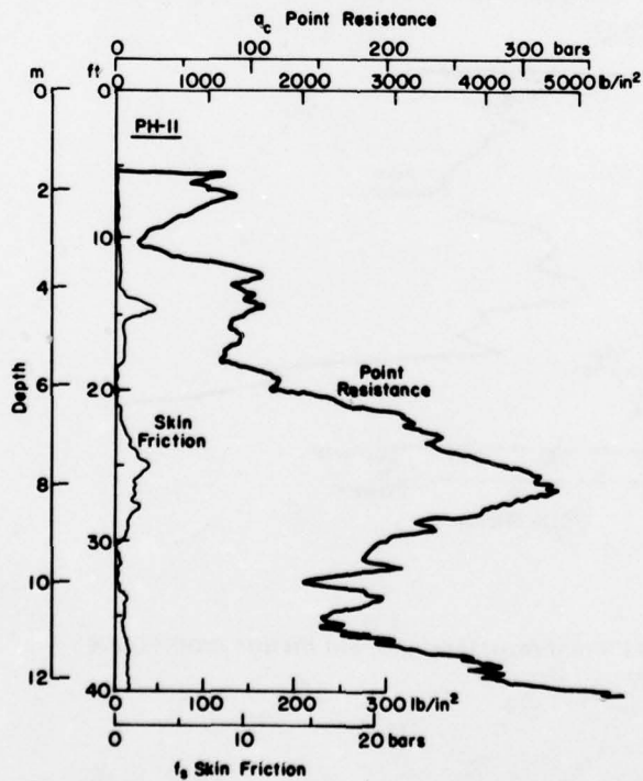
Figure B11. Point resistance and skin friction profiles, site PH-11.
