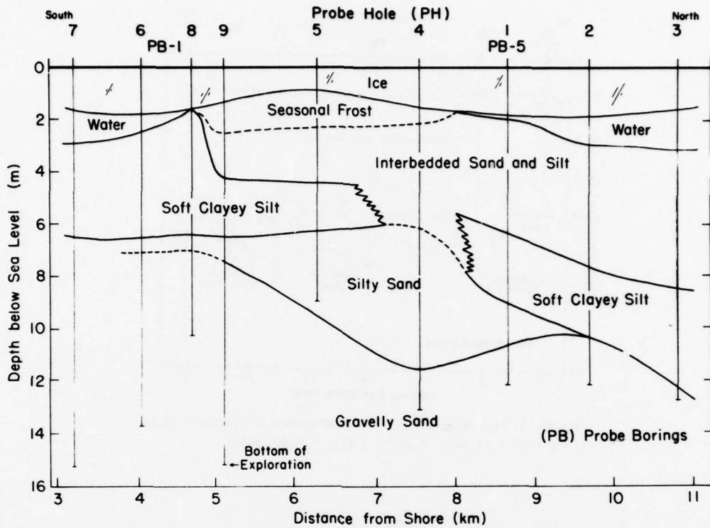
Figure 13. Stratigraphic profile interpreted from probe data along line 1. (1 m = 3.28 ft; 1 km = 0.62 mile)
