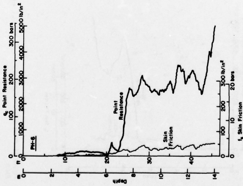
Figure B6. Point resistance and skin friction profiles, site PH-6.
