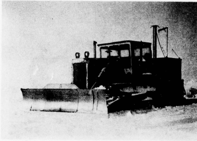
Figure A3. Tractor on sled runners to provide reaction force.
