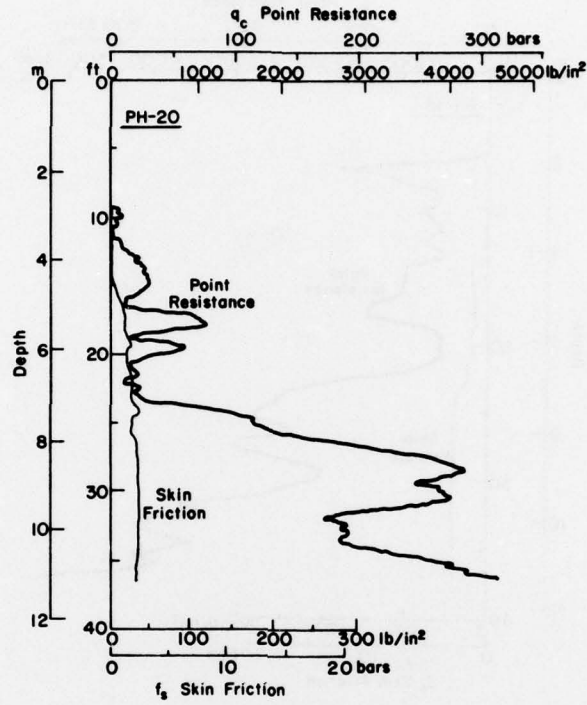
Figure B20. Point resistance and skin friction profiles, site PH-20.
