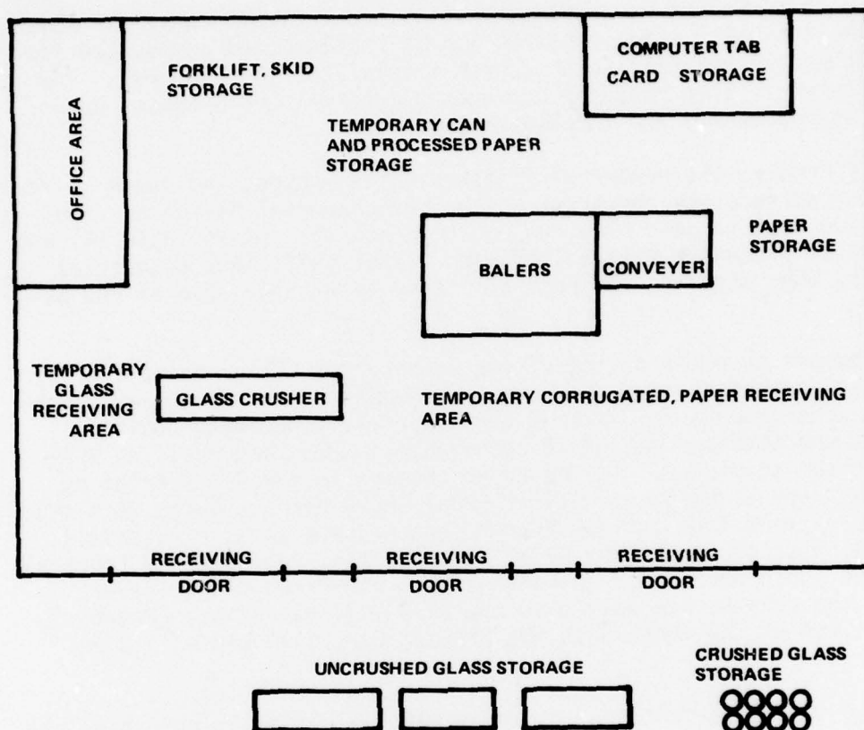
Figure 17. Recycle center processing activity (RCPA) layout.
