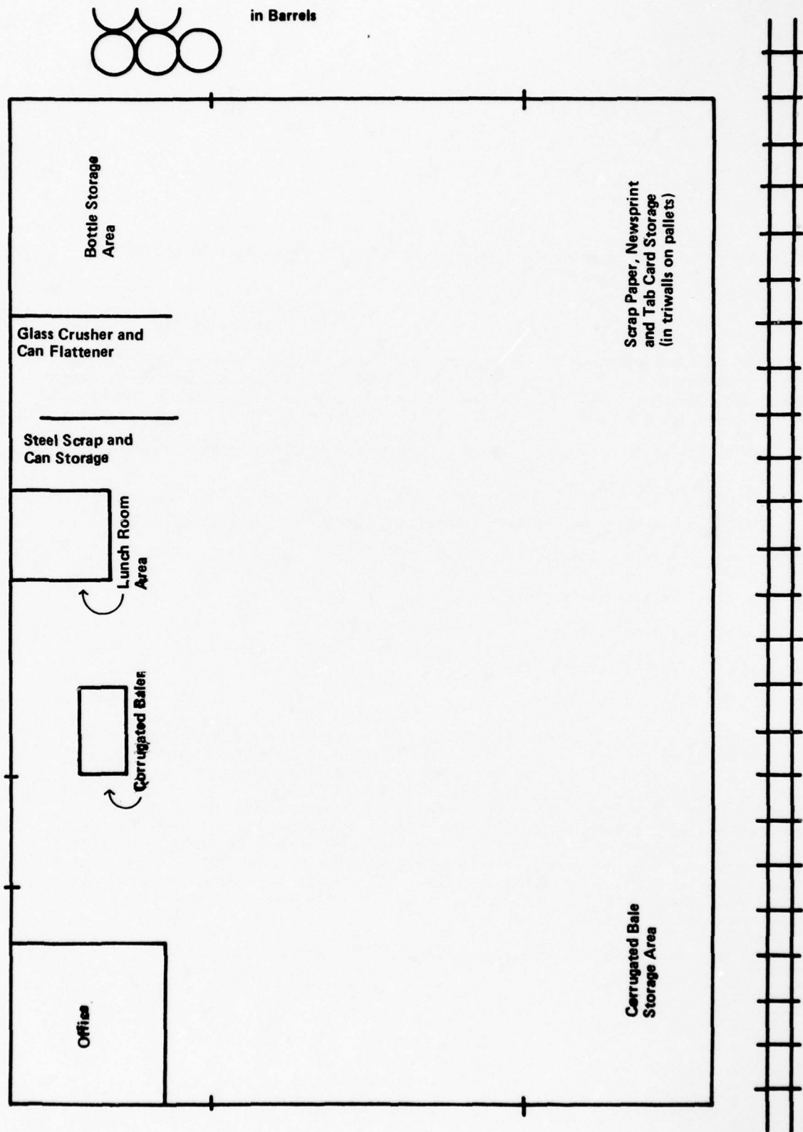
Figure 10. Layout of Recycling Center at Fort Lewis.
