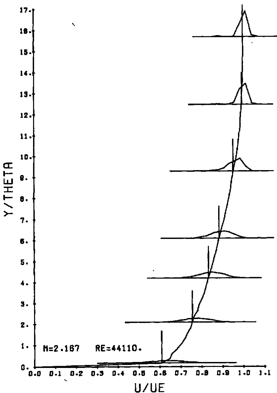
Figure 20. Representative histograms from the high-speed boundary layer.
