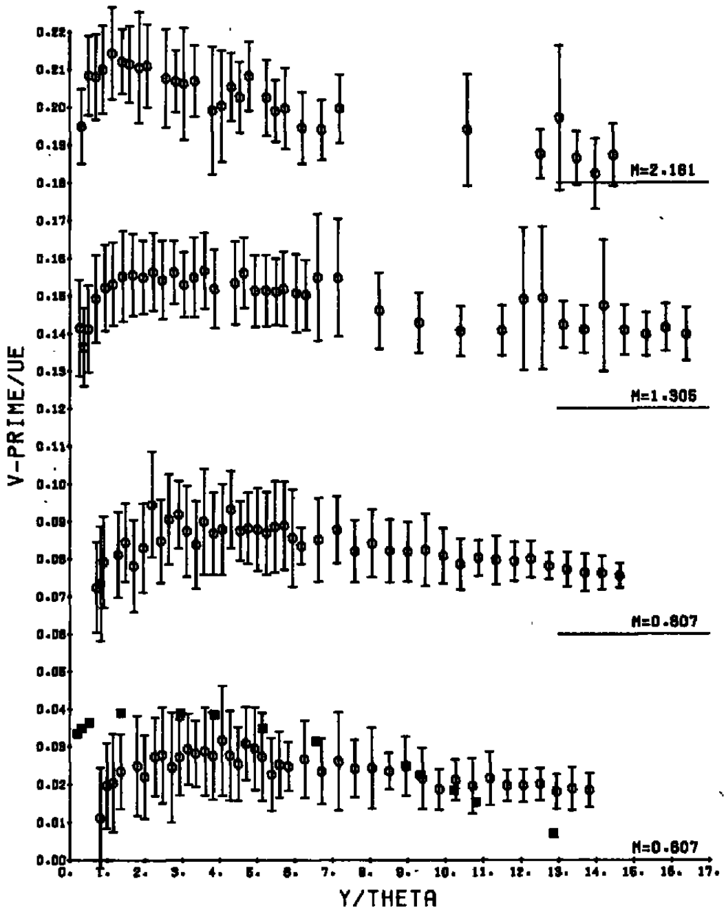
Figure 31. The distribution of the normal-velocity fluctuations, Re_{\theta} = 23,000 .
