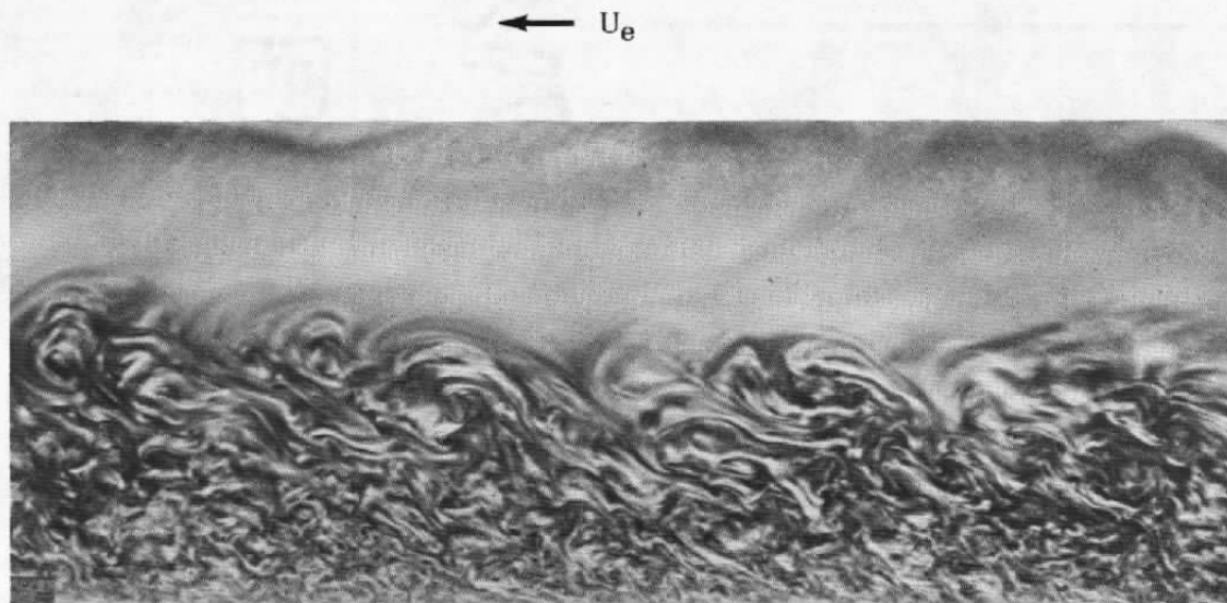
Figure 4. The structure of the turbulent boundary layer as visualized by the use of aluminum flakes in water; photograph courtesy of Brian Cantwell, Caltech (1978).
