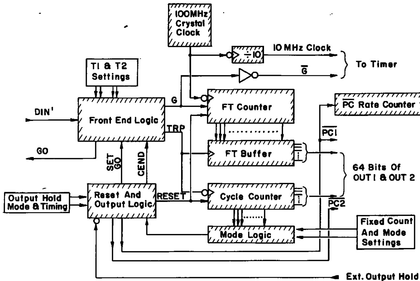
Figure 17. The digital input processor.
