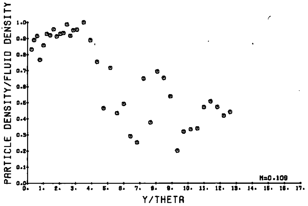
Figure 9. The distribution of particle number density, Re_c \approx 6,900 .
