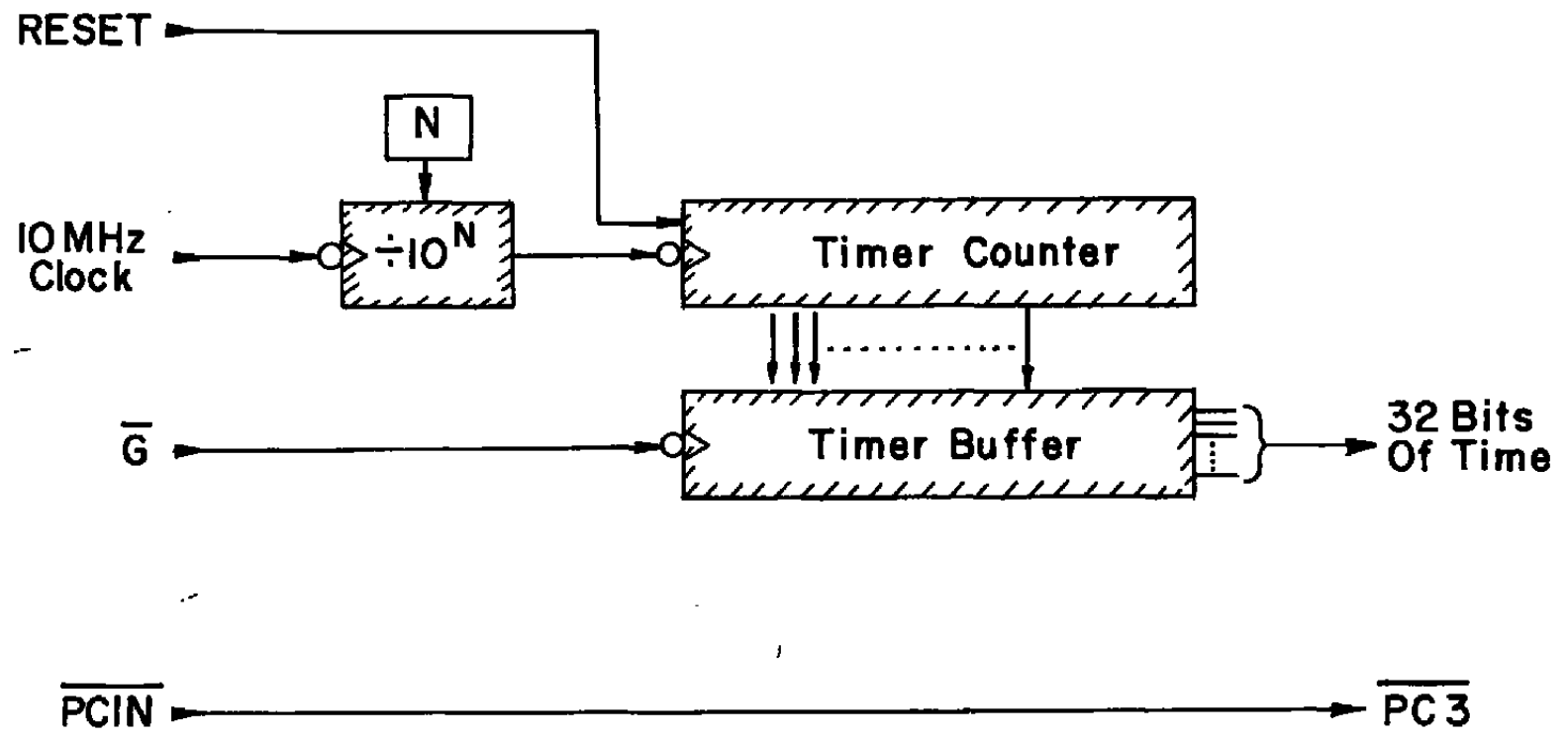
Figure 18. The timing circuit.
