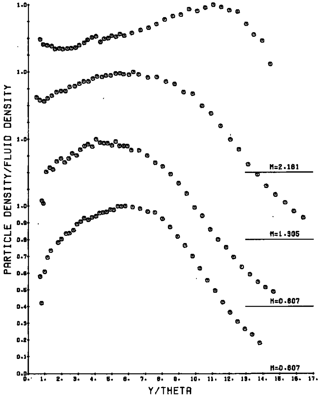
Figure 7. The distribution of particle number density, Re_0 \approx 23,000 .
