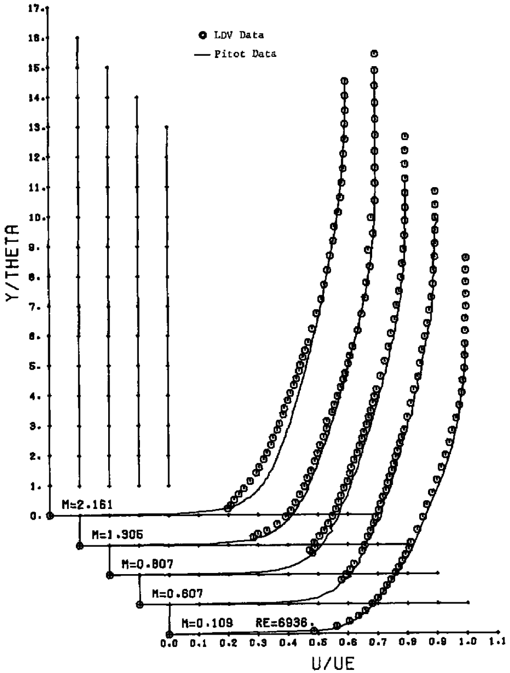
Figure 22. Mean velocity profiles, Re_{\theta} = 23,000 .
