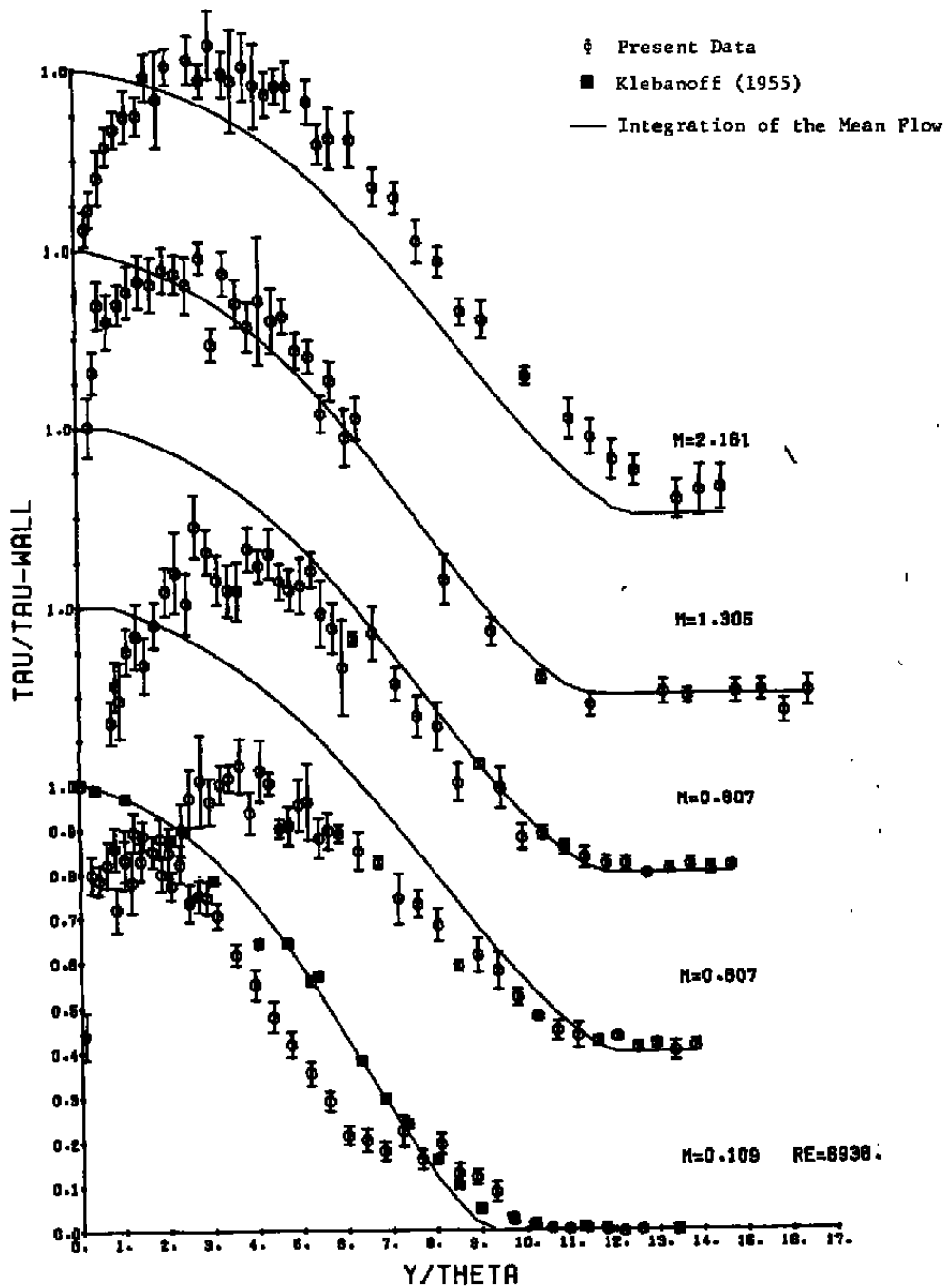
Figure 28. The distribution of Reynolds stress, Re_{\theta} = 23,000 .
