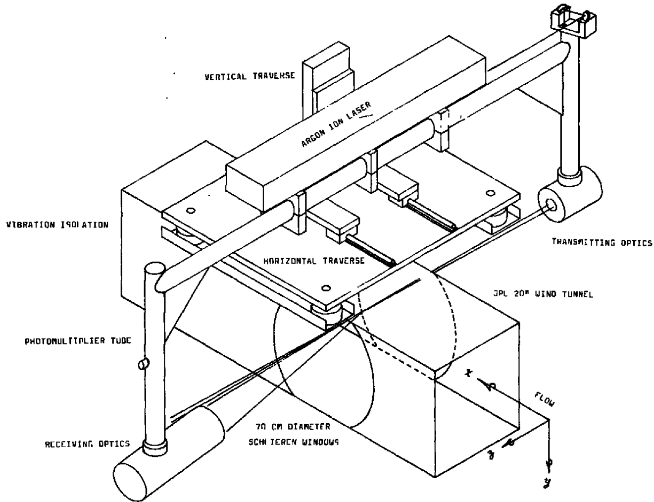
Figure 10. High-speed laser-Doppler velocimeter.
