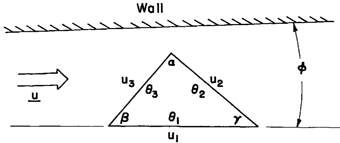
Figure 12. The optical geometry relative to the wall.
