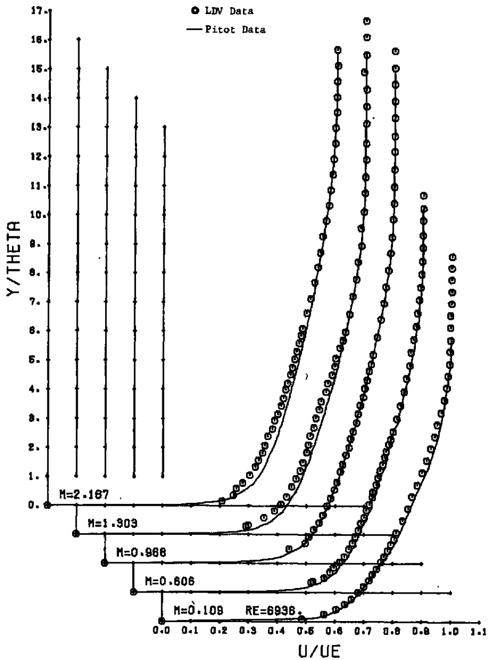
Figure 23. Mean velocity profiles, Re_{\theta} = 40,000 .
