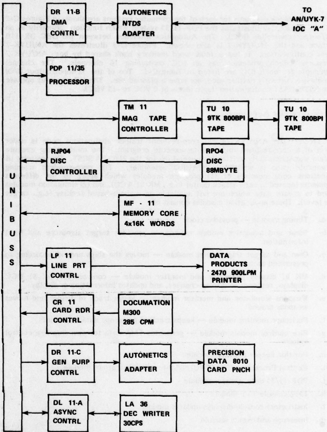
Figure C-2. PDP-11/35 System
