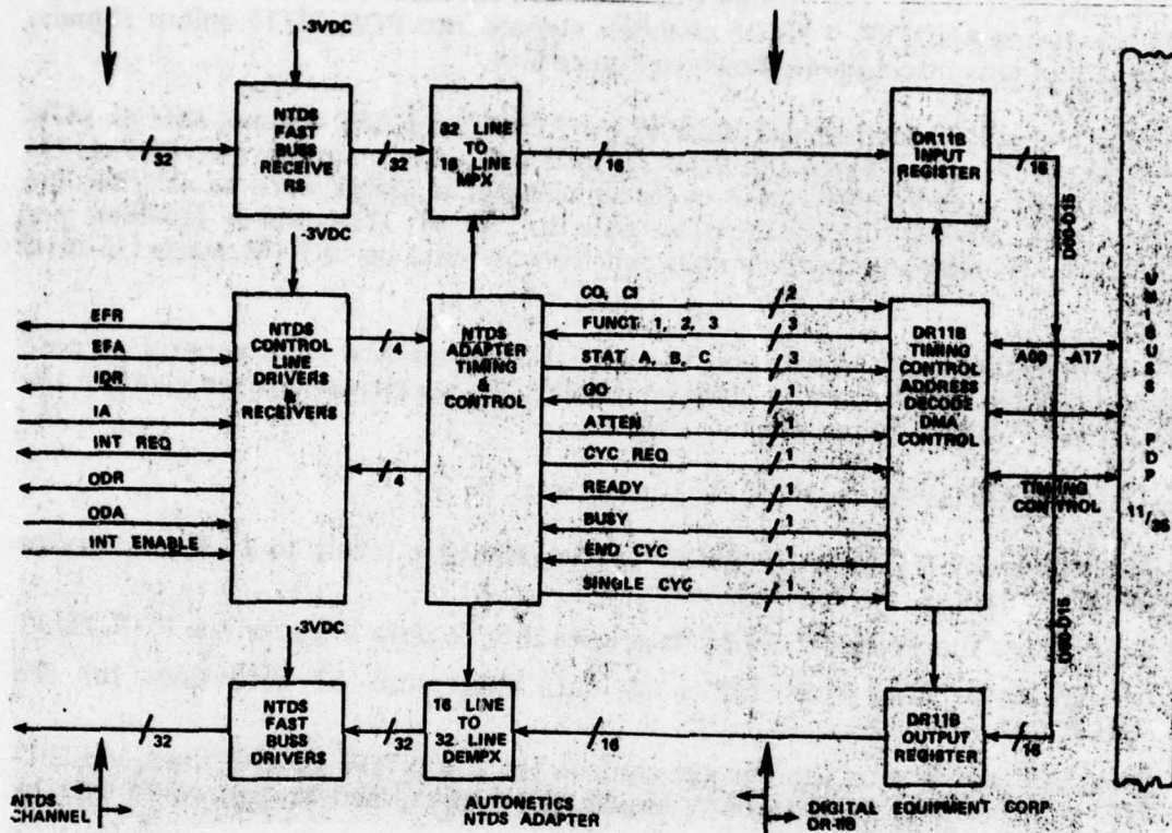
Figure C-6. Autonetics Interface
