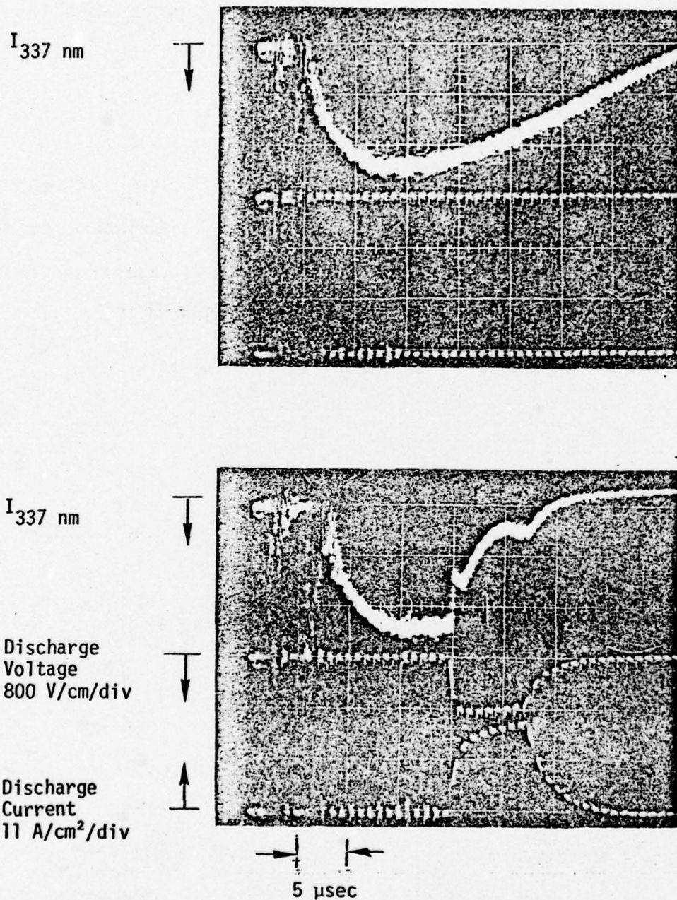
Figure 6. Fluorescence Emission from the v = 0 Level of the \text{N}_2(\text{C}^3\Pi_u) State. The upper oscillogram shows the emission produced by the e-beam; the lower oscillogram shows the effect of the discharge on this emission.
