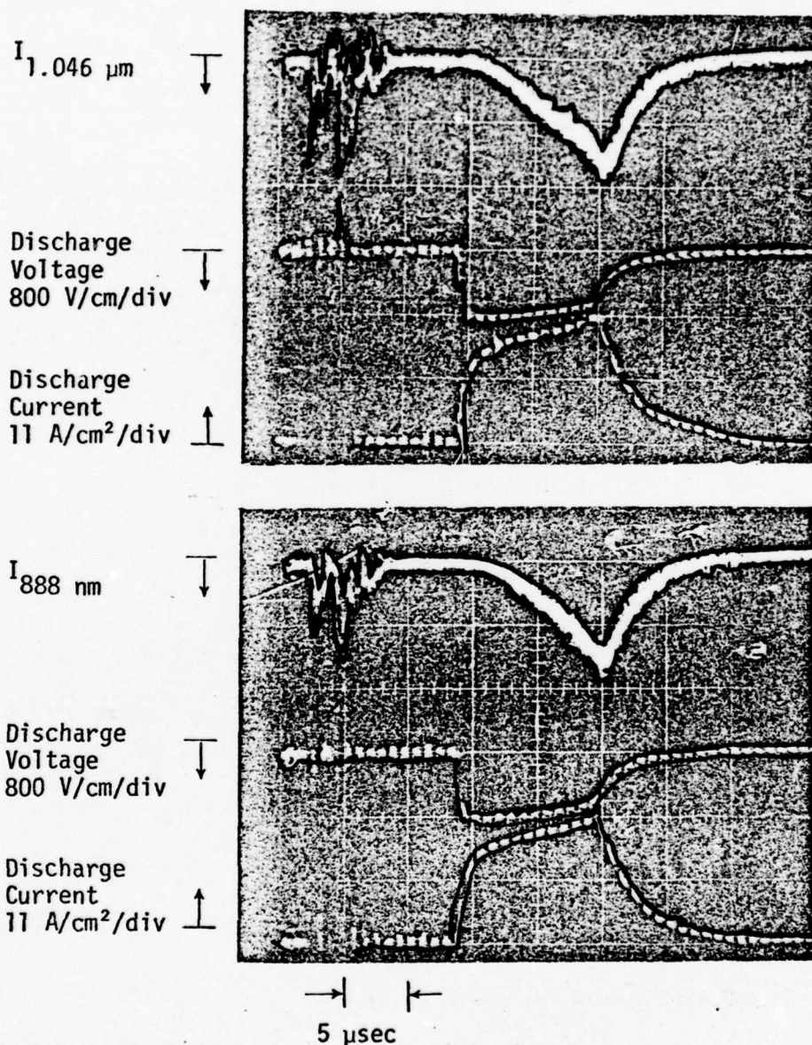
Figure 9. Fluorescence Emission from the v = 0 and v = 1 Levels of the \text{N}_2(\text{B}^3\Pi_g) State in a 5:1 Ar+N 2 Mixture at 200 Torr. The upper oscillogram shows the (0,0) band and the lower oscillogram shows the (1,0) band of the nitrogen first positive system.
