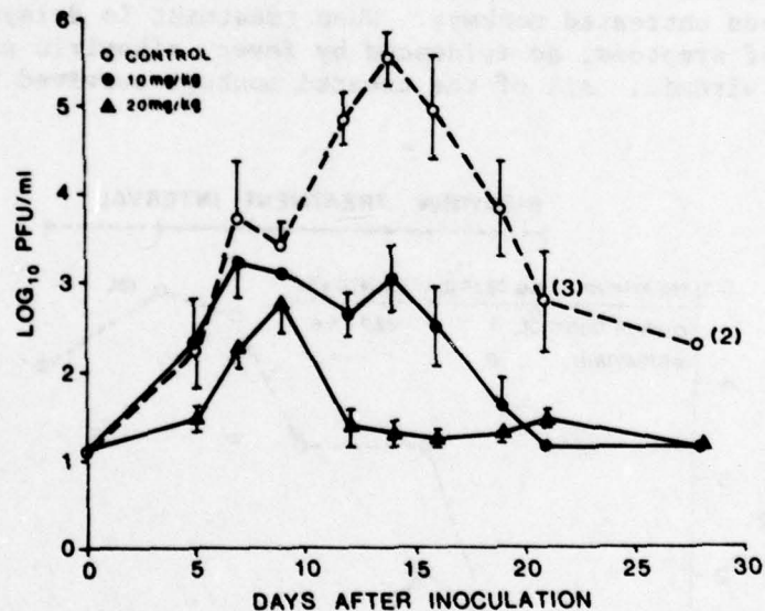
Fig. 6. Effect of ribavirin on viremia in MAC-infected rhesus monkeys
