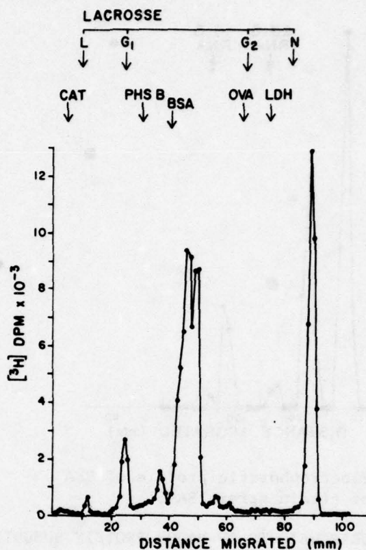
Fig. 1. Electrophoretic profile of RVF virus, strain SA-51
