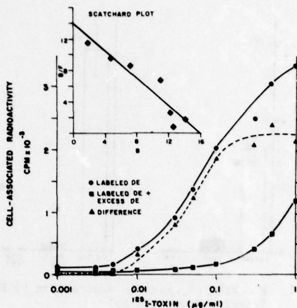
Fig. 2. Binding isotherm
