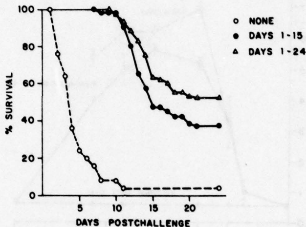
Fig. 2. Effect of oral ribavirin on RVF-infected mice
