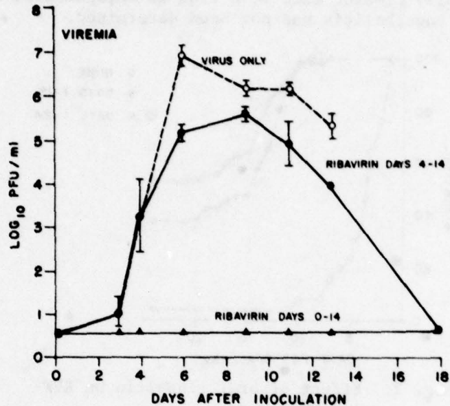
Fig. 4. Effect of ribavirin treatment on viremia
