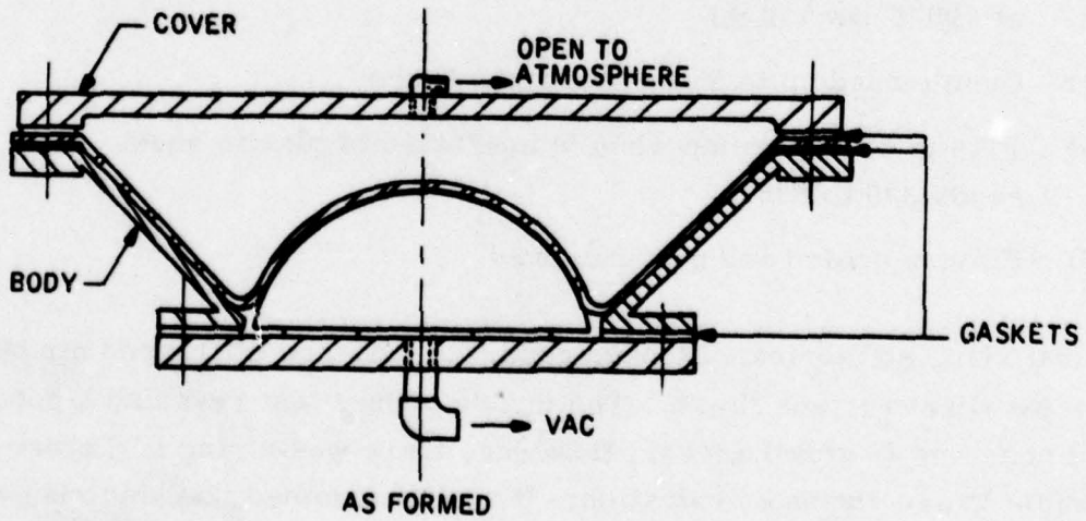
Figure 3-16 Closed Vacuum Forming System
