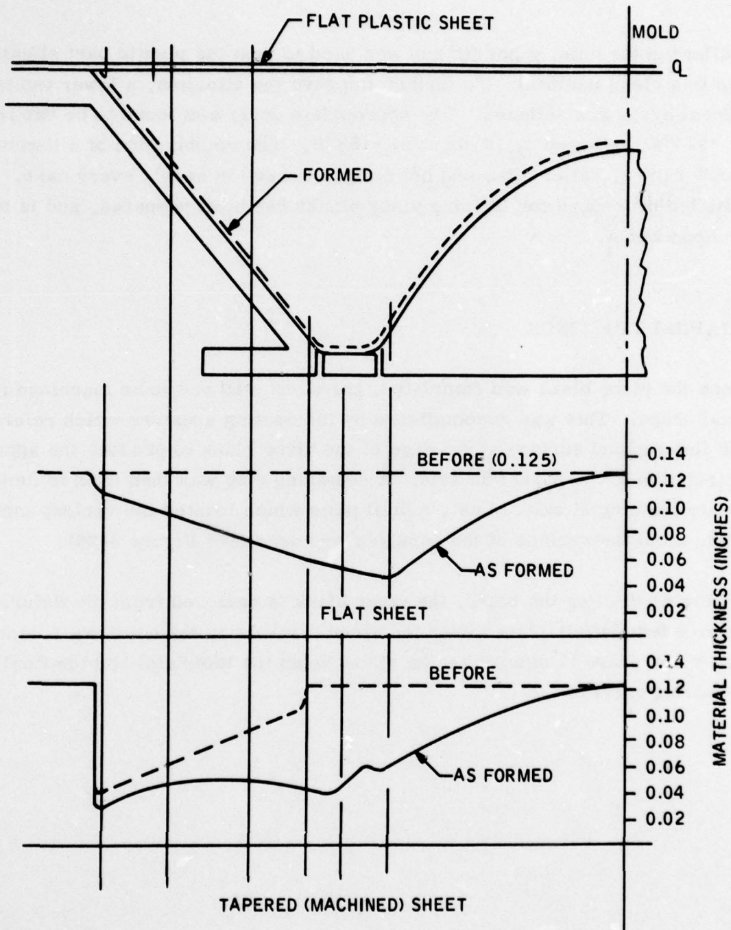
Figure 3-24. Sheet Thinning Comparison
