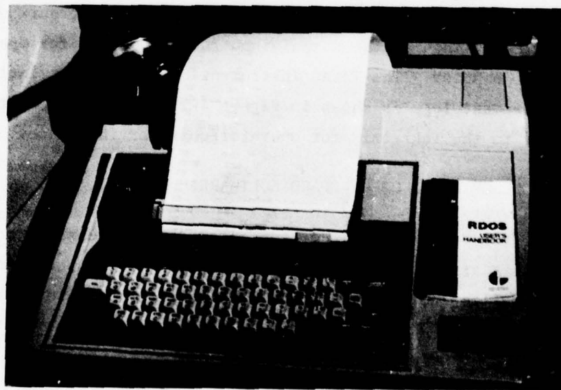
Figure 4-2. Alternate Operator Console or Operation Logging Device
