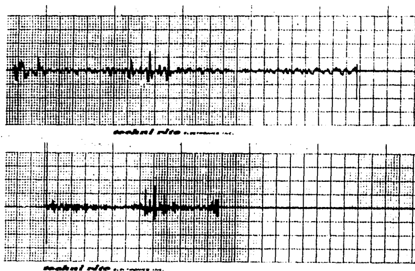
TAPE NO. 18. SCAN OF HOLE NO. 65. THIS SHOWS A SMALL CRACK ON ONE SIDE OF THE INTERFACE.
