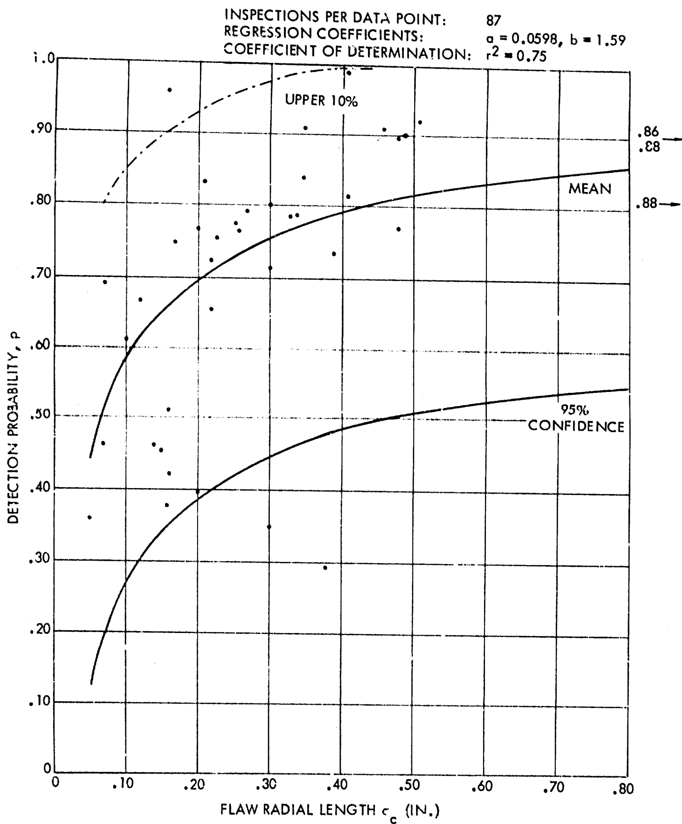
Figure 10-4. Probability of Detection Versus Fatigue Crack Radial Length, Eddy Current Surface Scans Around Countersunk Fasteners, Skin and Stringer Wing Segments, Sample B.
