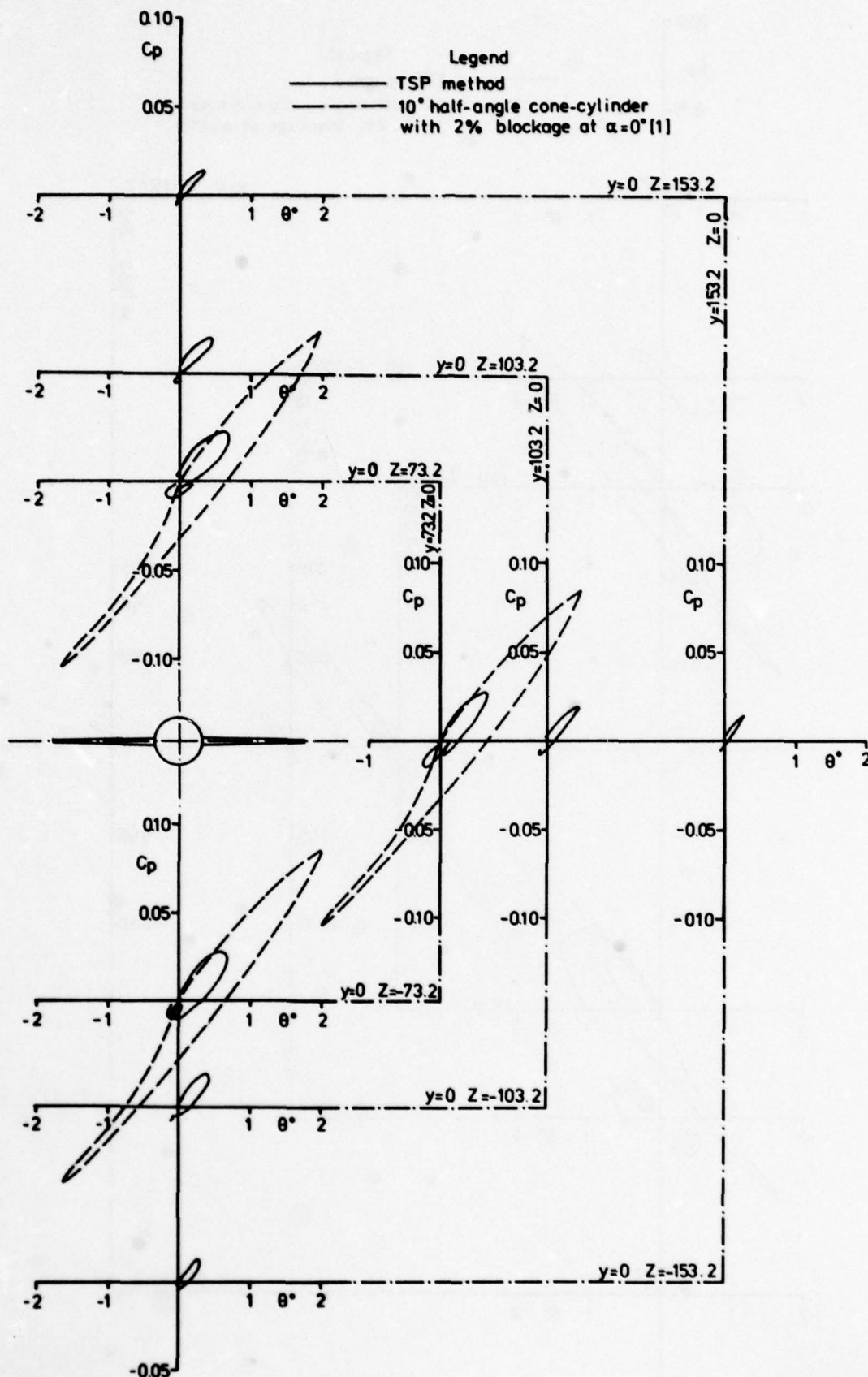
Figure 12. Calculated disturbance distribution of the wing-body configuration at M_\infty = 1.2 and \alpha = 0
