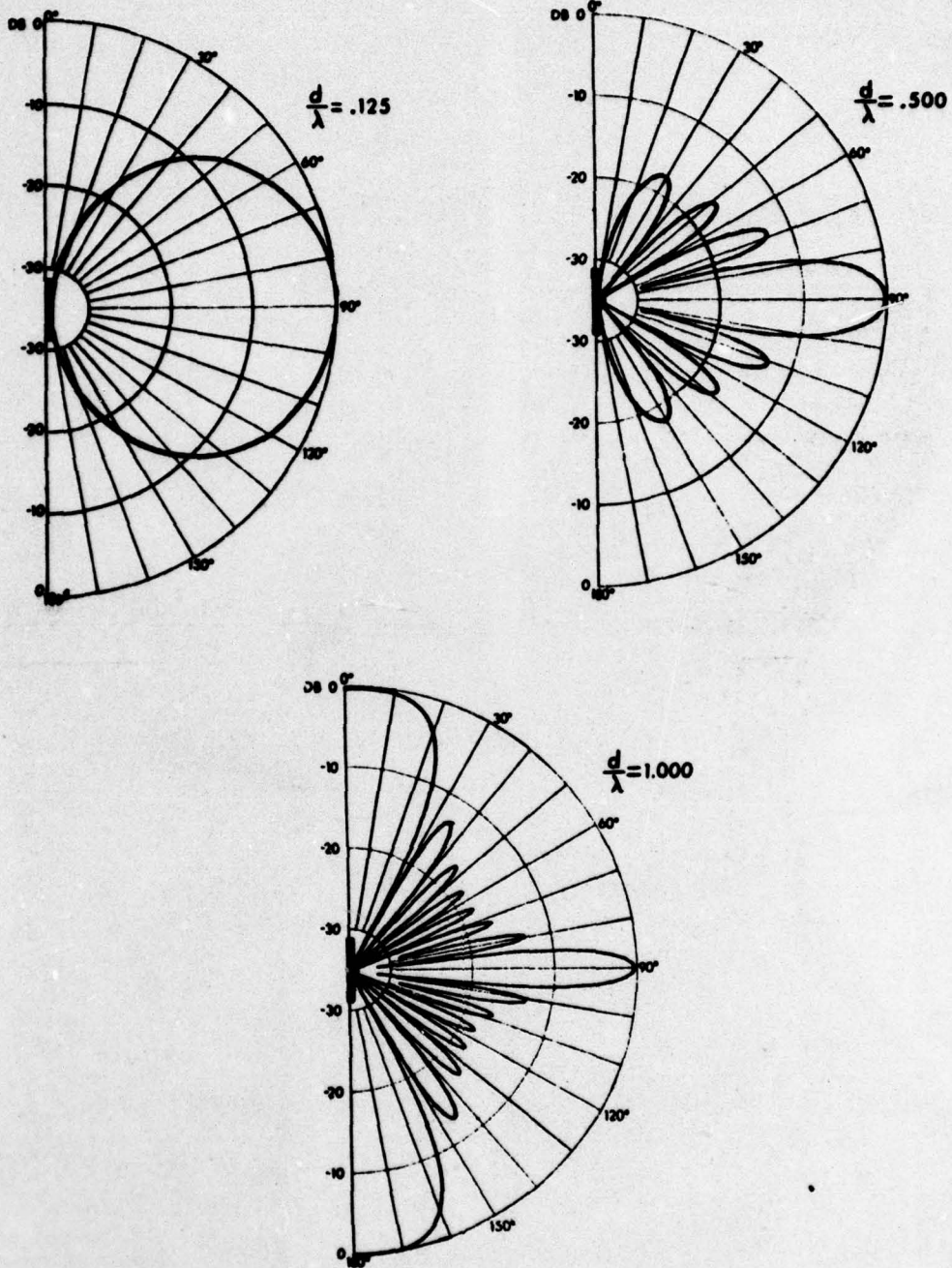
Intensity Patterns for 8 Vertical Elements and Single Frequency with Broadside Steering
