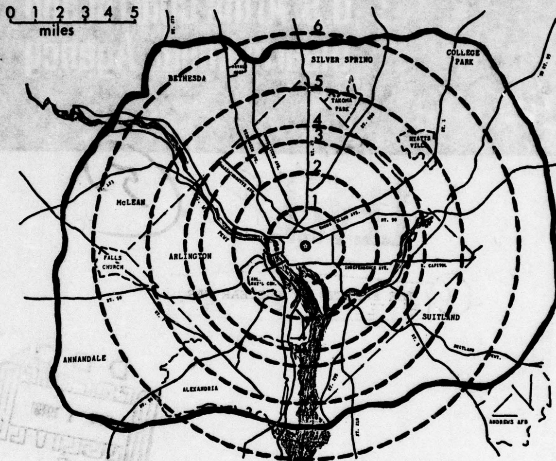
One Megaton Weapon Air Burst
