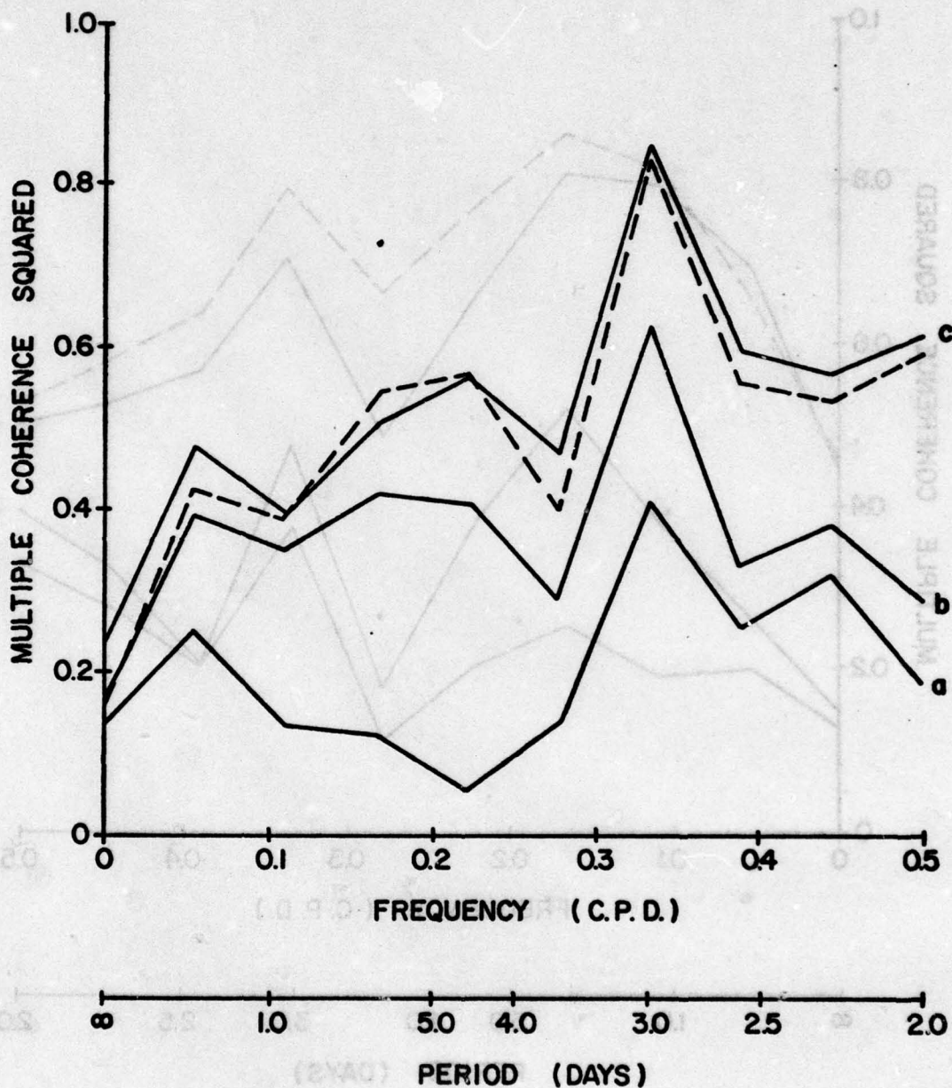
Fig. B19. Summer multiple coherence.
