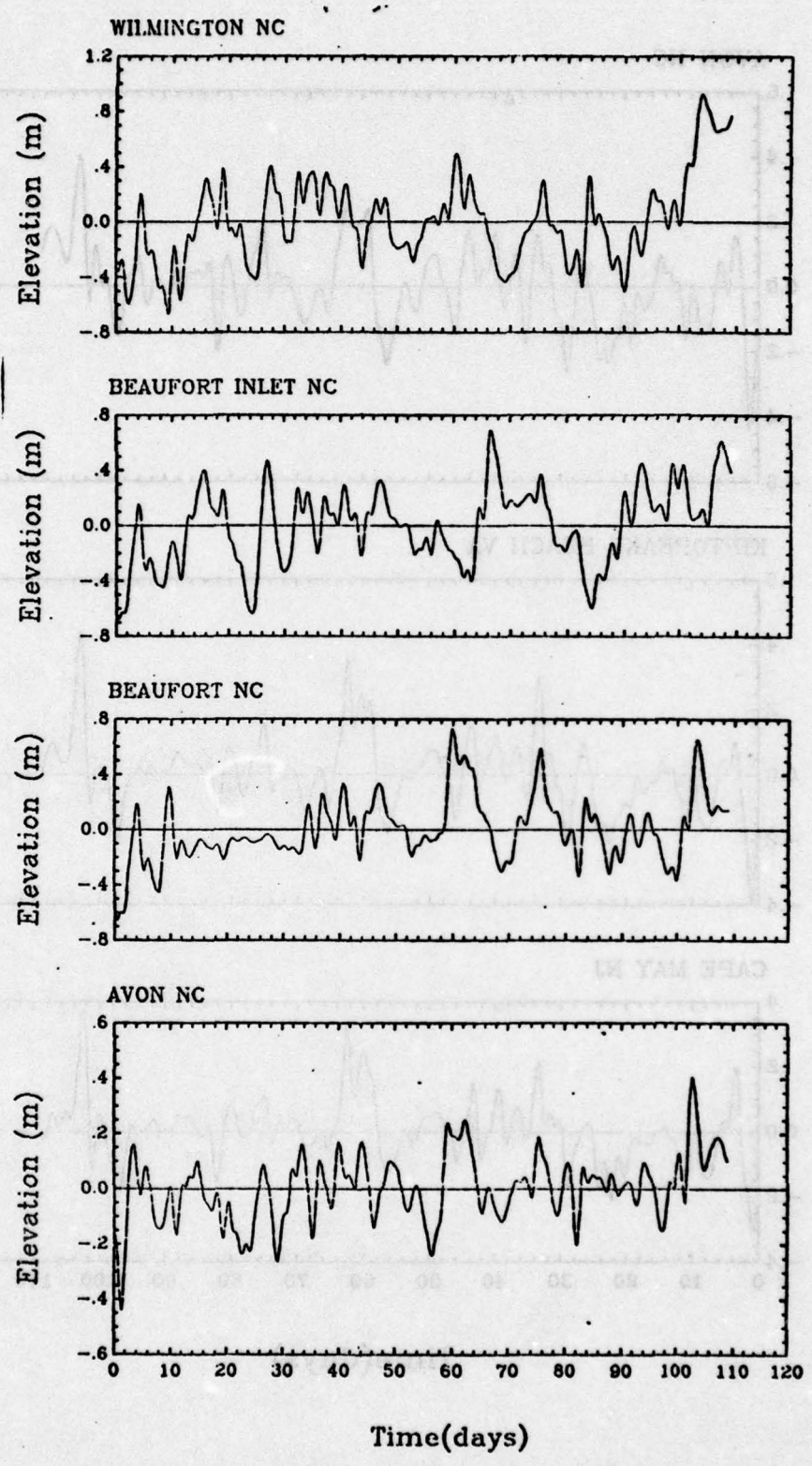
Fig. A.8 Summer adjusted sea level.
