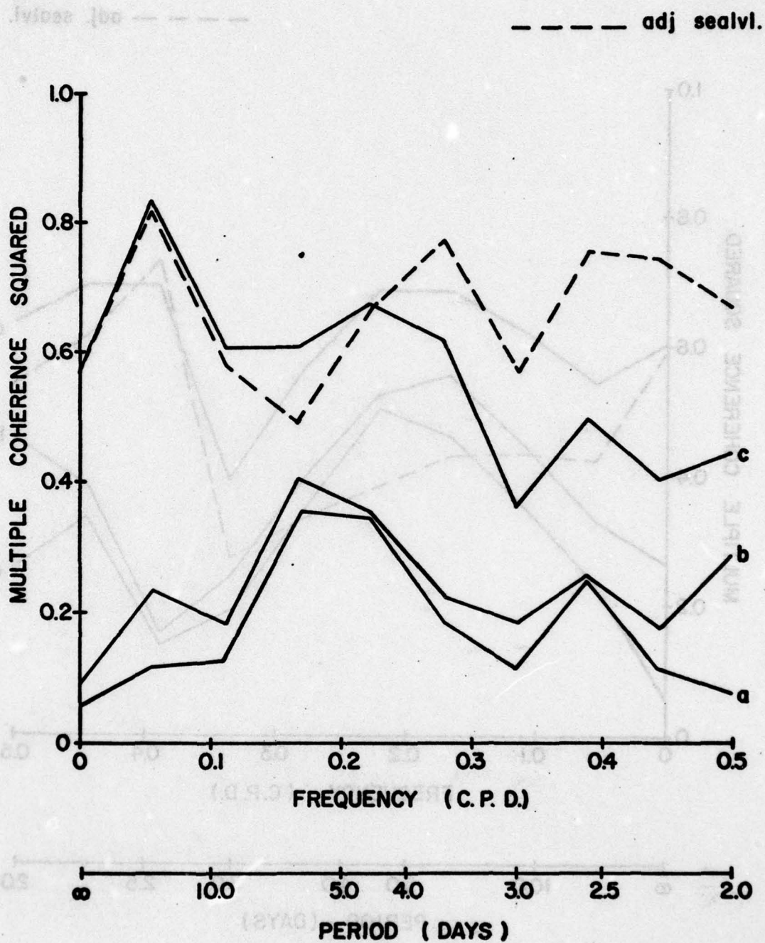
Fig. B2. Winter multiple coherence.
