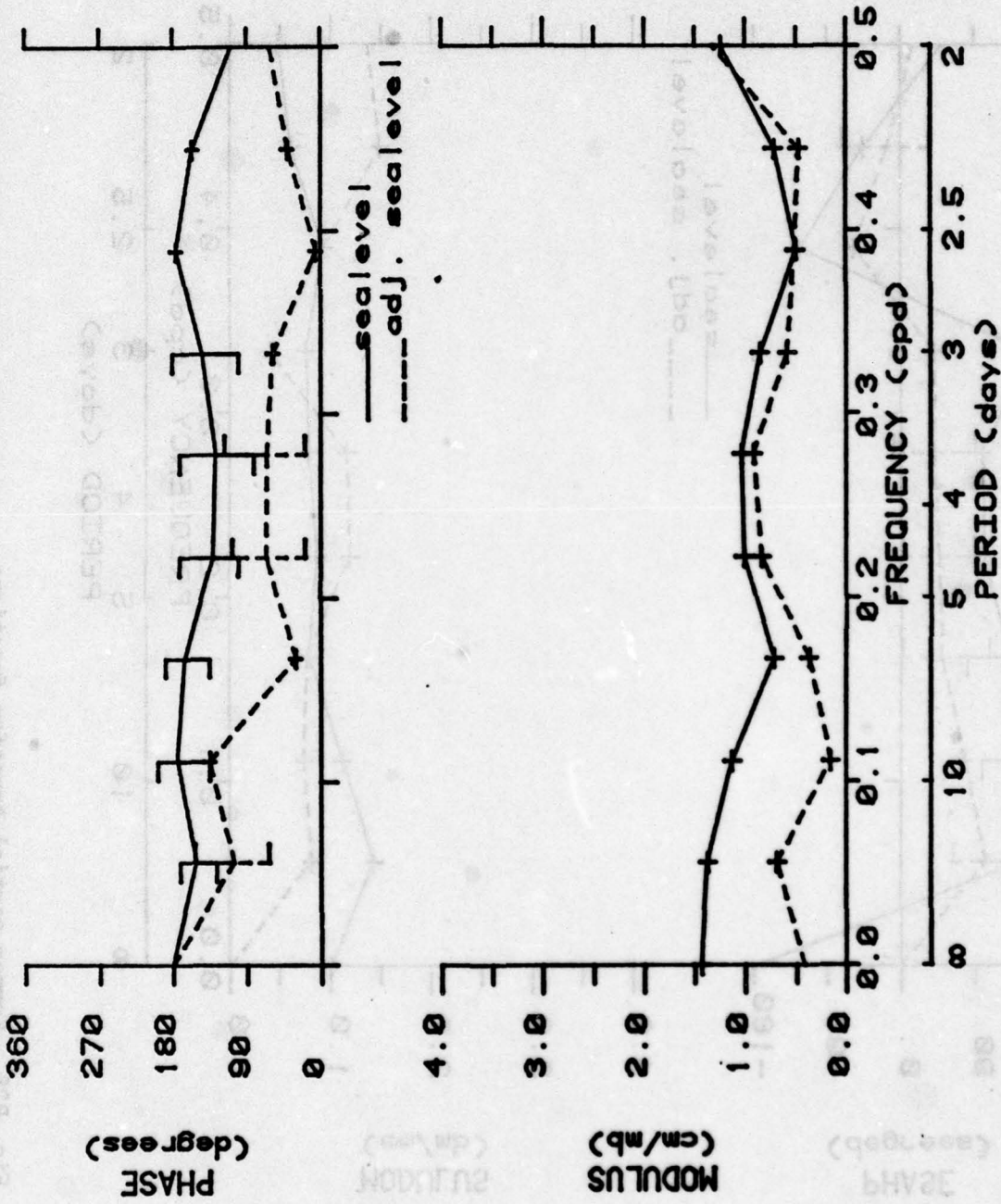
Fig. B25. Summer partial transfer functions.
