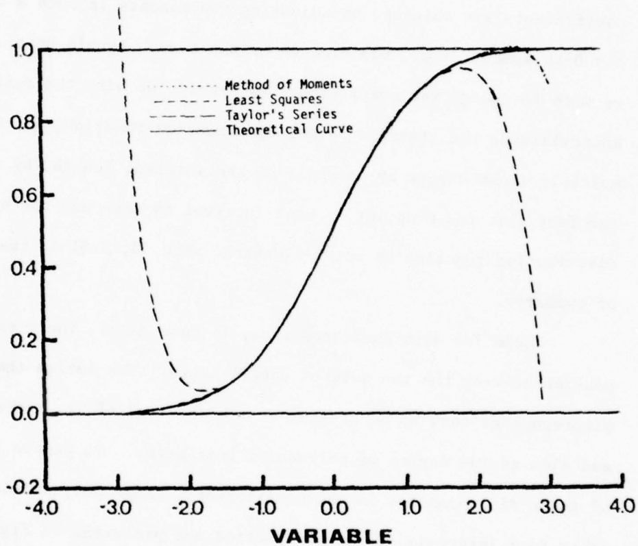
FIGURE 7-1 (Continued): Polynomials Are of Degree 7 .
