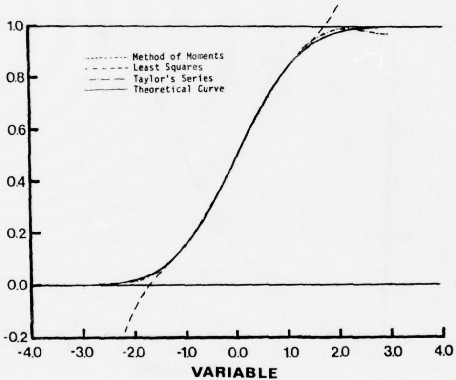
FIGURE 7-1 (Continued): Polynomials Are of Degree 5 .
