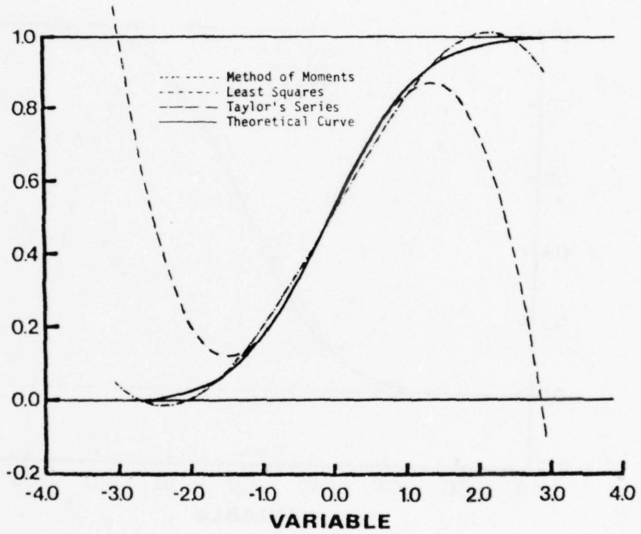
FIGURE 7-1 (Continued): Polynomials Are of Degree 4 .
