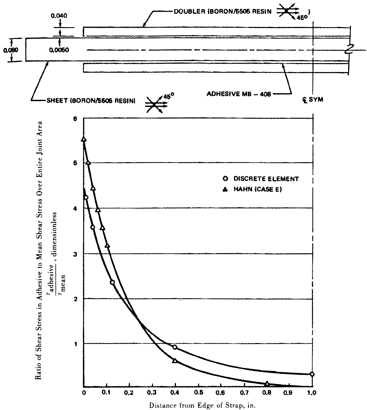
Figure 2-9. Comparative Discrete Element and Analytic Analyses of a Bonded Joint 3
