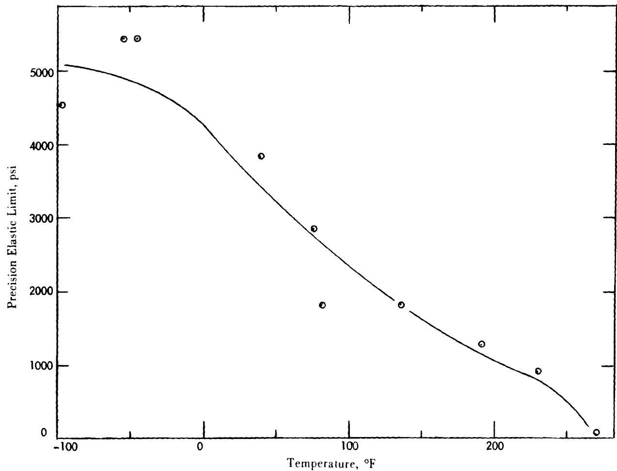
Figure 3-18. Tensile Tests, Metlbond 329, Aluminum Adherends 4
