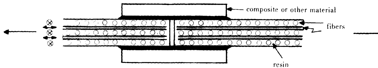
(A) Poor --surface fibers normal to load
