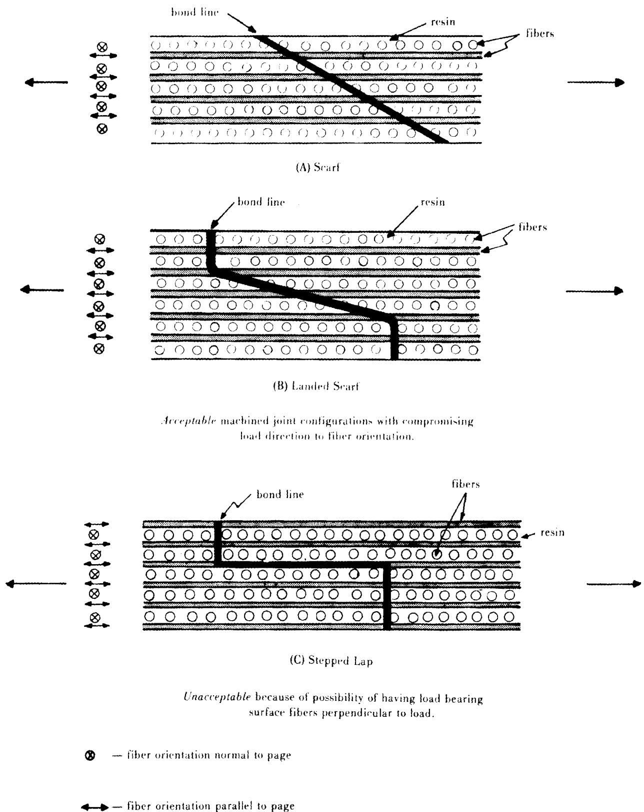
Figure 2-20. Machined Joints
