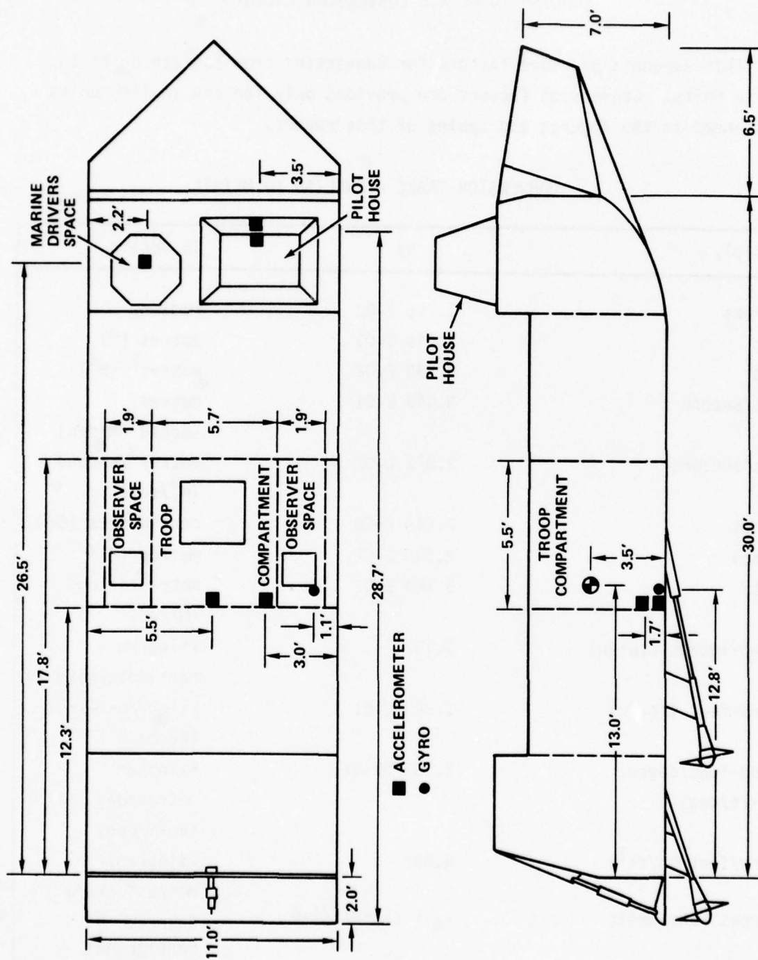
(not drawn to scale) Figure 1 - Sketch of FSHV Showing Dimensions and Transducer Layout
