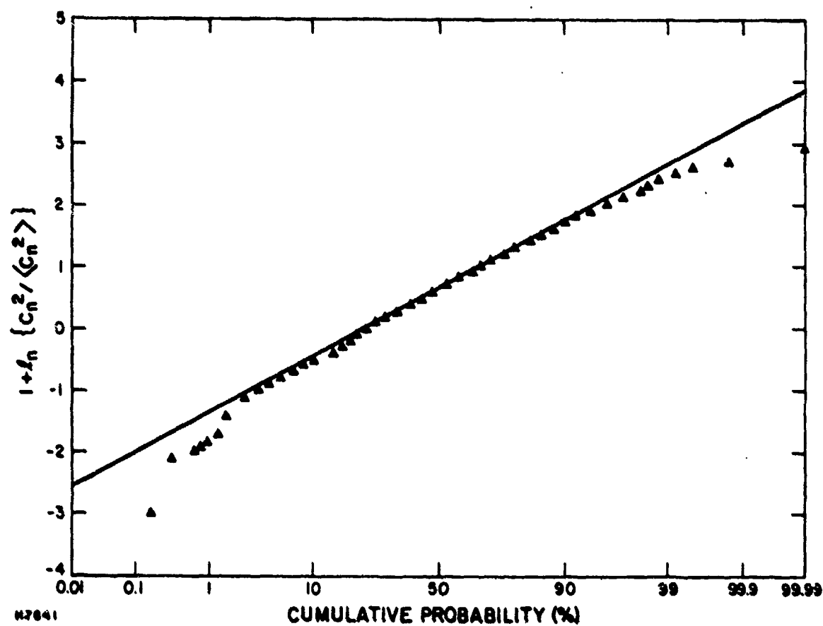
Figure 8 Normalized Upper Atmospheric Turbulence Levels. Data is from Model I Star Sensor. The straight line is for Gaussian statistics with the empirical mean and variance.
