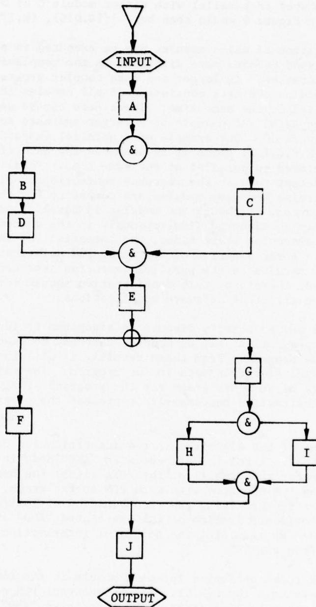
Figure 9. The R-net of a simple program for illustrating the identification of modules executable in parallel.
