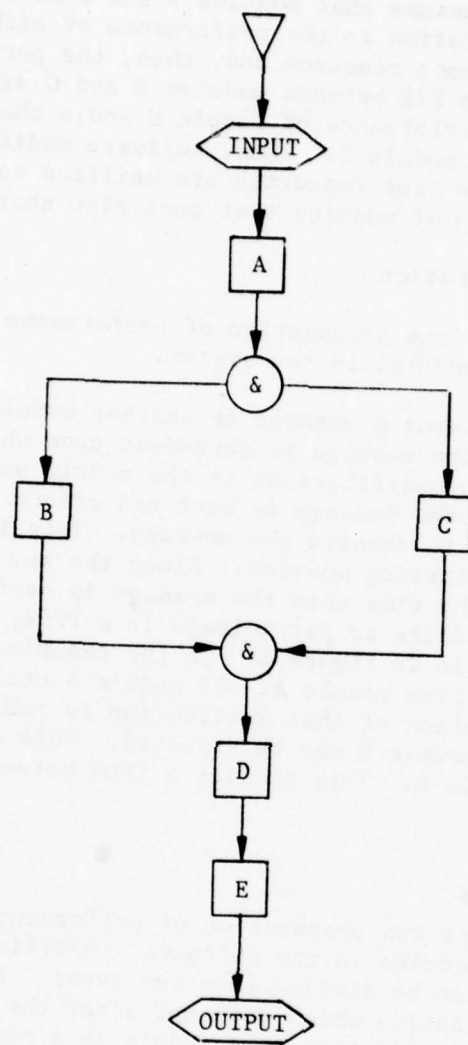
Figure 7. The R-net of a simple program for illustrating shared resources mechanism.
