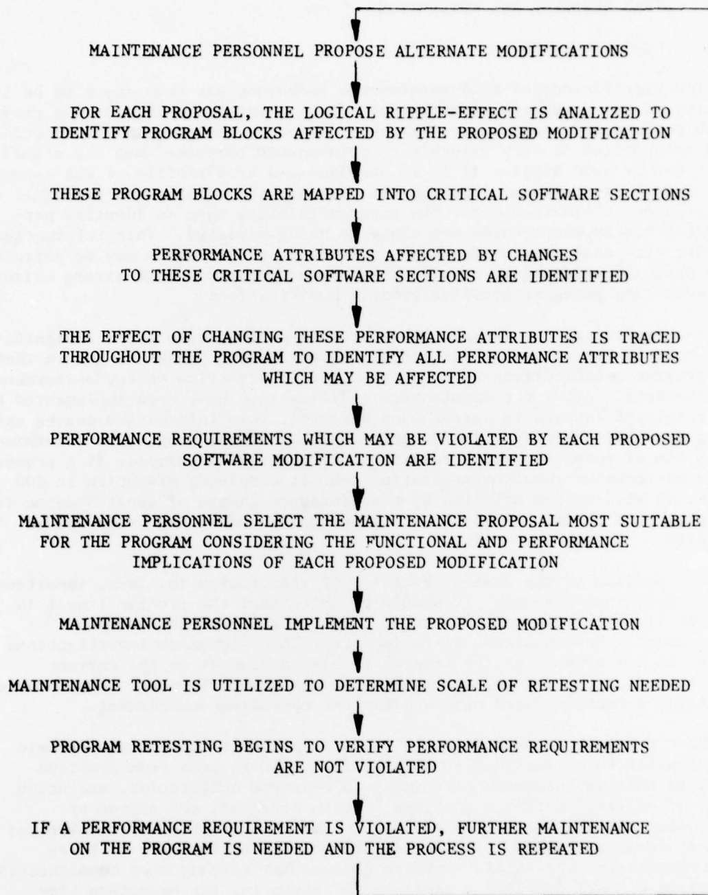
Figure 15. Application of the maintenance technique in the prediction of performance requirements affected by the maintenance activity and in the retesting phase.
