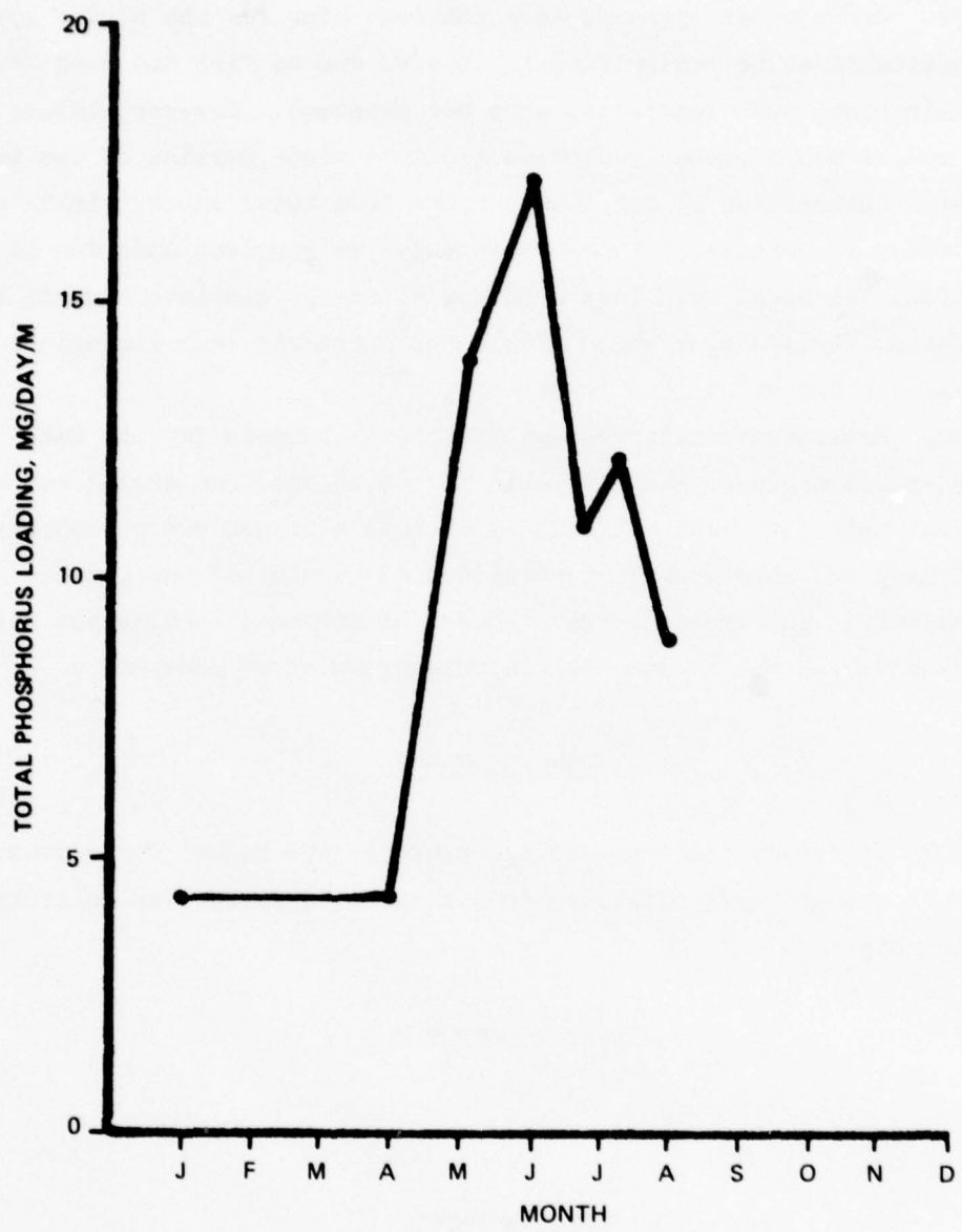
Figure 6. Total phosphorus seepage loading rates, Lake Conway system
