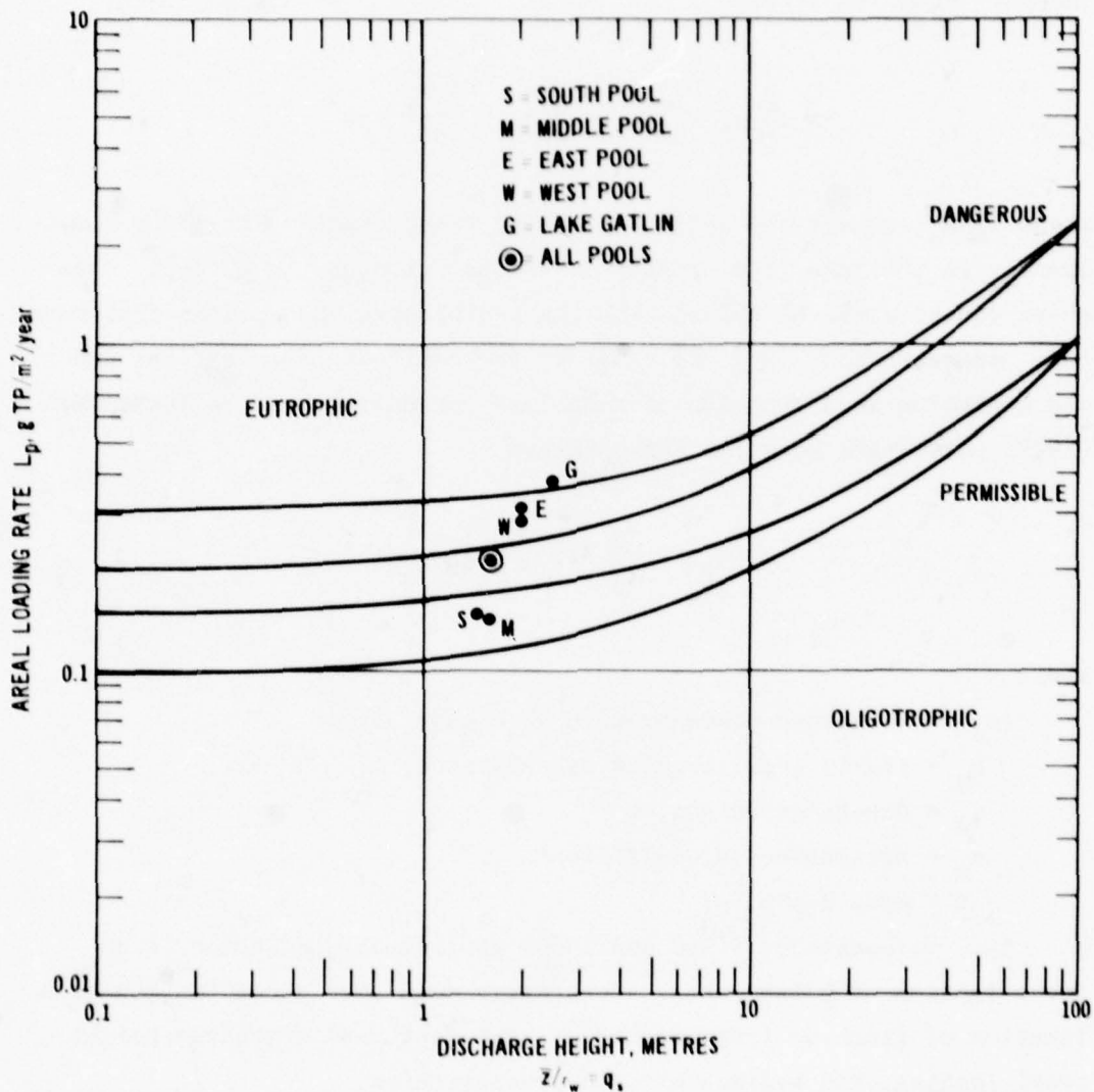
Figure 7. Areal phosphorus loadings of Lake Conway system
