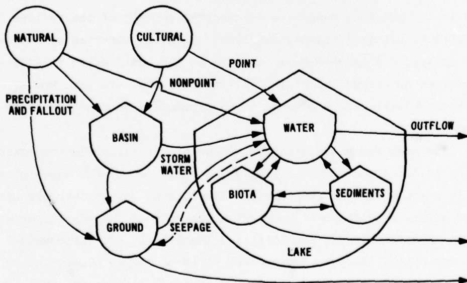
Figure 1. Simplified model of nutrient pathways in a lake ecosystem (symbols after Odum 1971)
