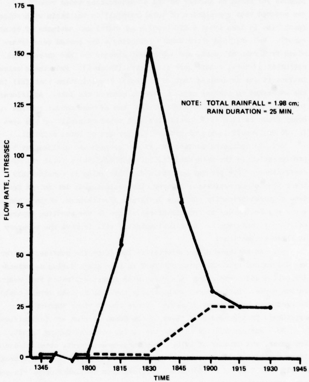
Figure 4. Runoff hydrograph of 21 August 1976 at Gatlin Avenue and Bumby Drive for Lake Conway basin
